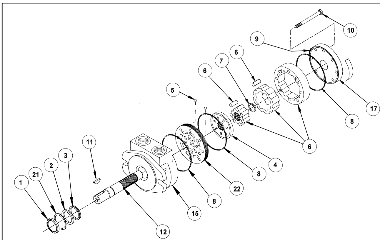
Figure 1-48 Winch Motor Assembly
