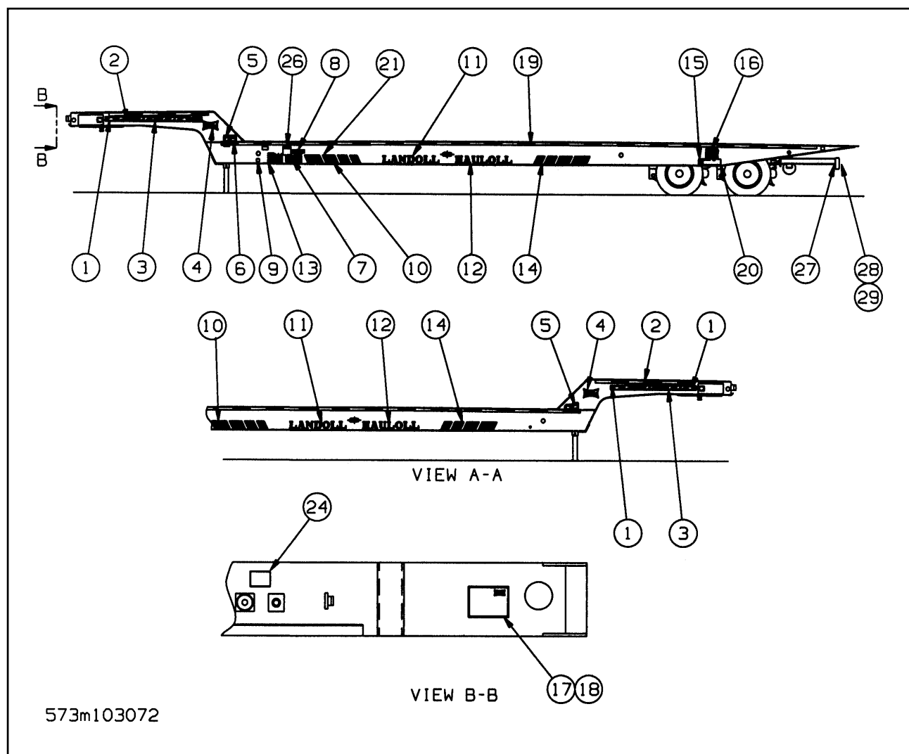
Figure 1-61 Decal Installation
