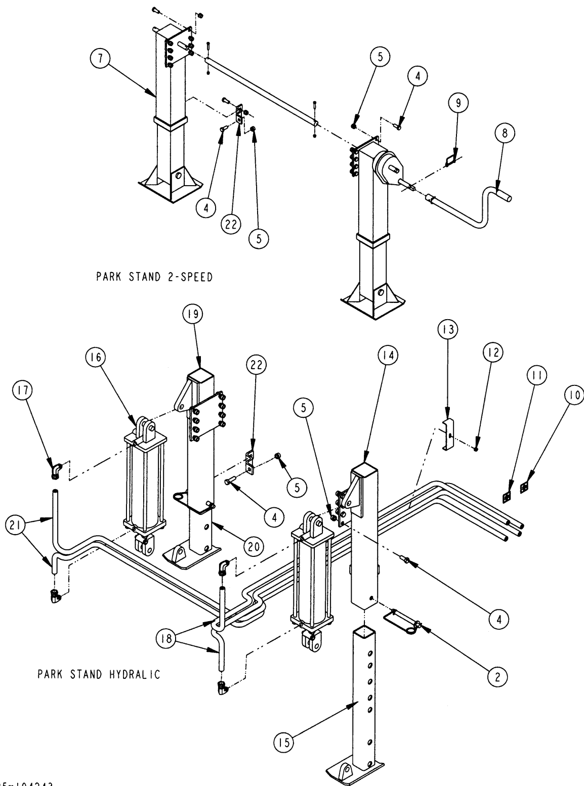
Figure 1-82 Landing Gear Instal.- Bolt-On (Optional)
