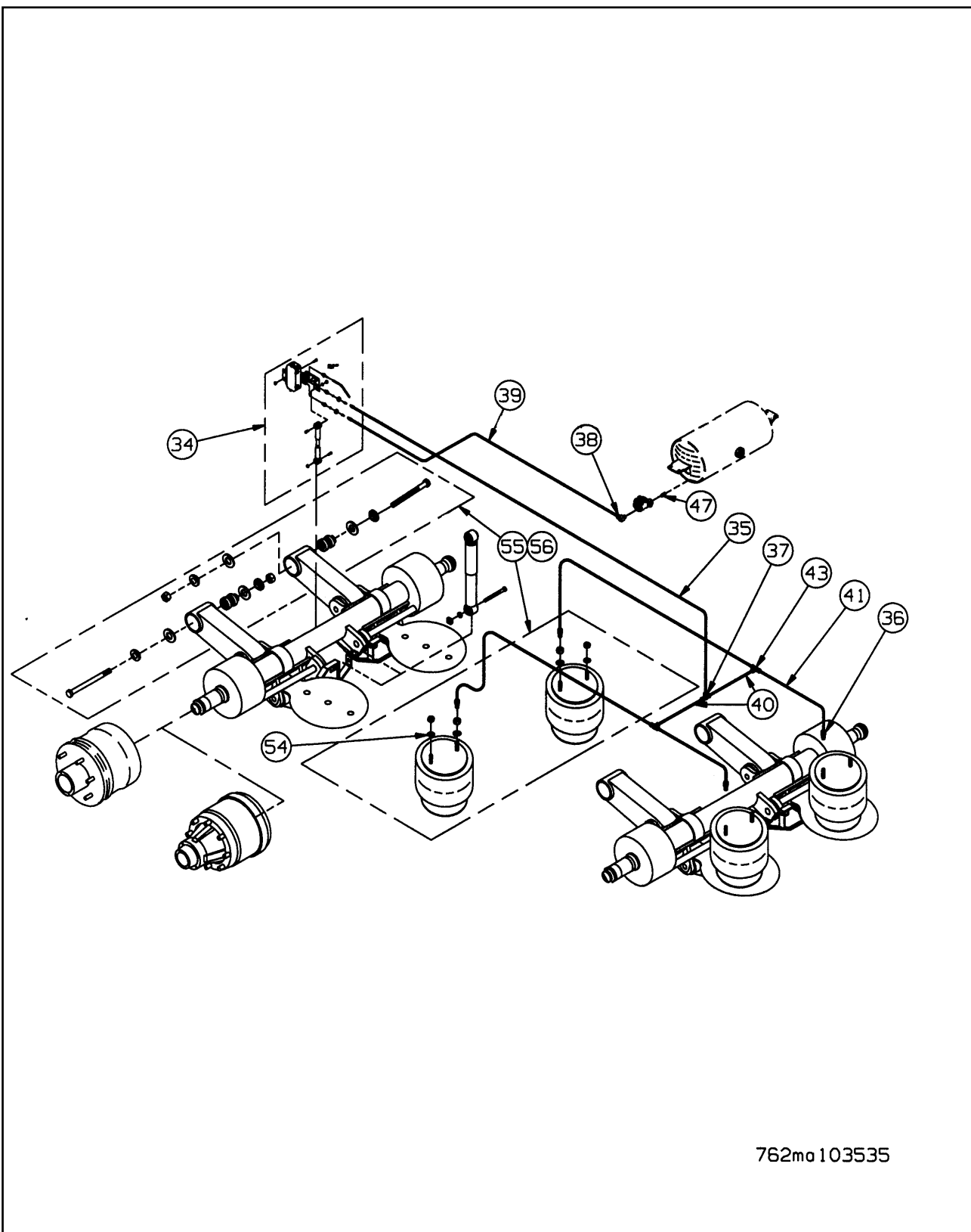
Figure 1-22 Undercarriage Suspension Air Ride (317B & 319B) (2 of 2)
