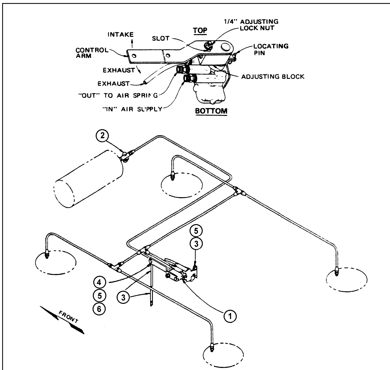
Figure 1-25 Air Control Kit, RLU-228 (2 of 2)
