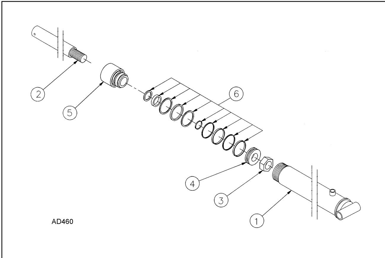
Figure 1-8 Cylinder 4" X 42"
