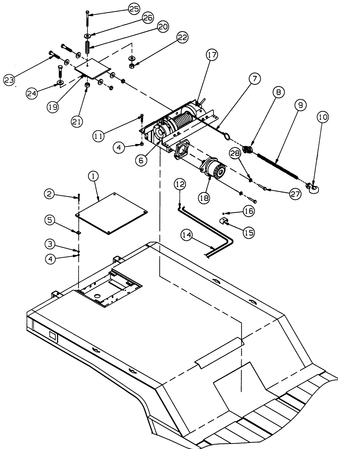
Figure 1-40 Winch Installation, Slope
