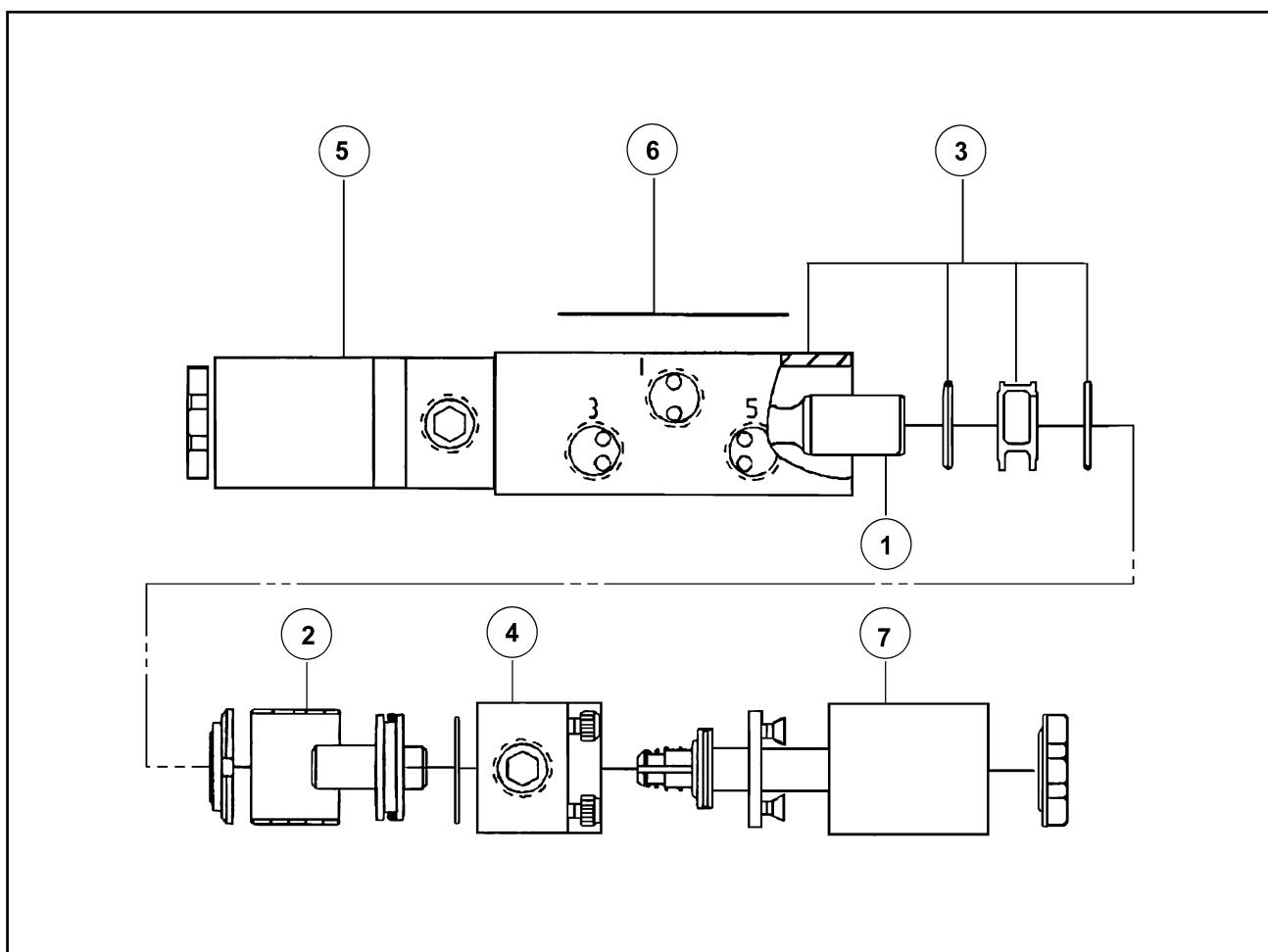
Figure 1-11 Pneumatic Valve
