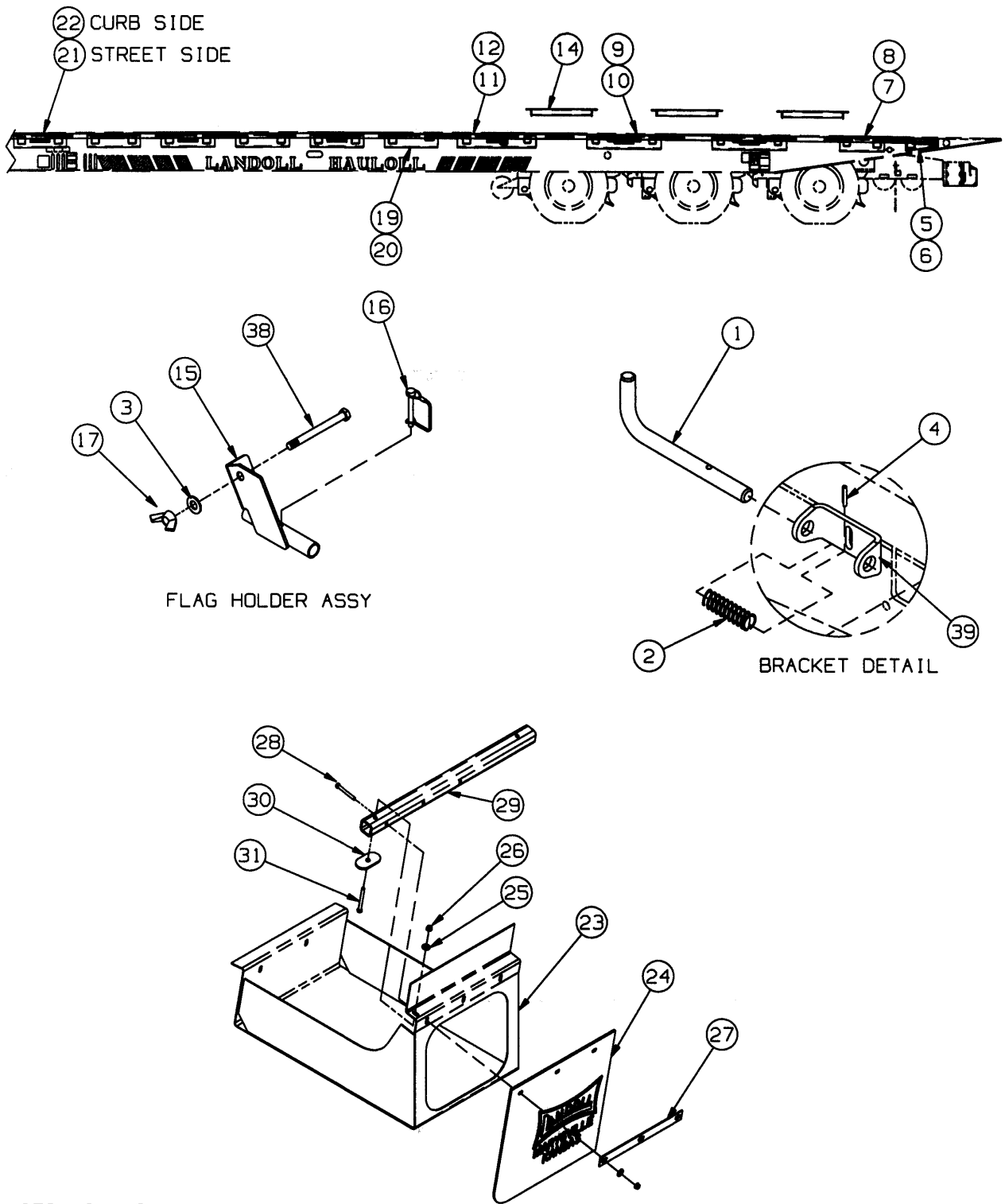
Figure 1-77 Extension Installation 318B (Optional)
