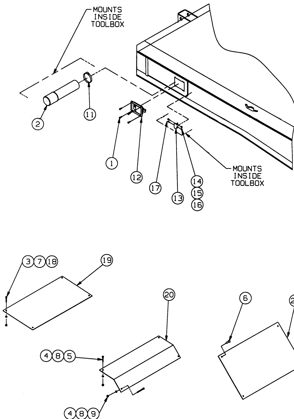
Figure 1-58 Door Latch Installation
