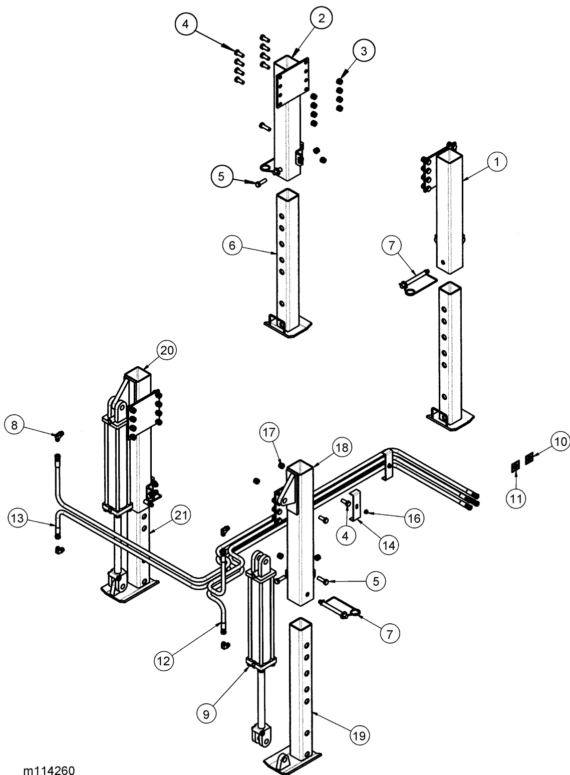
Figure 1-71 Landing Gear Installation - Bolt-On
