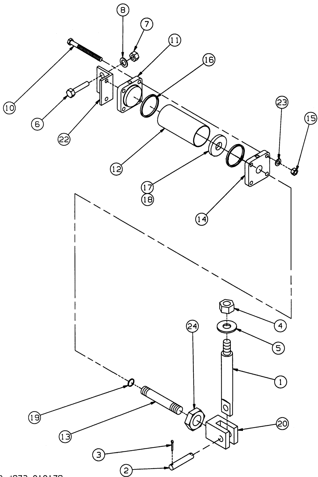
Figure 1-45 Winch Air Shift Cylinder
