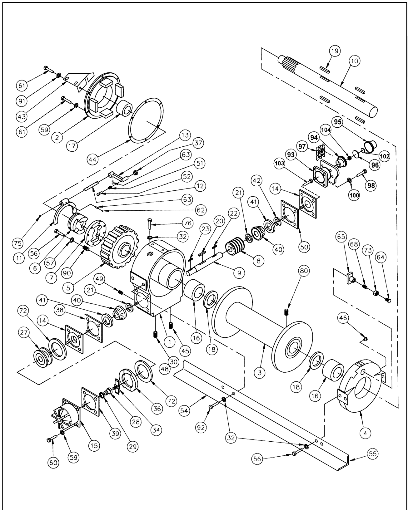
Figure 1-42 20,000# Winch Items
