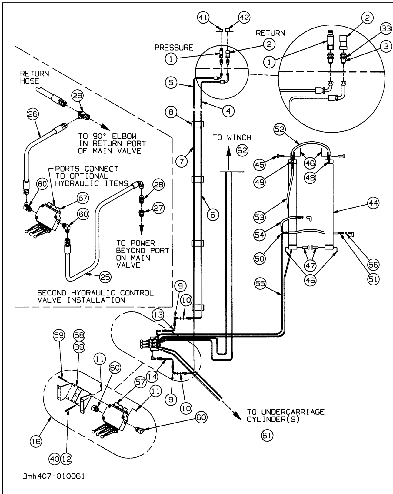
Figure 1-5 Hydraulic System (319C)
