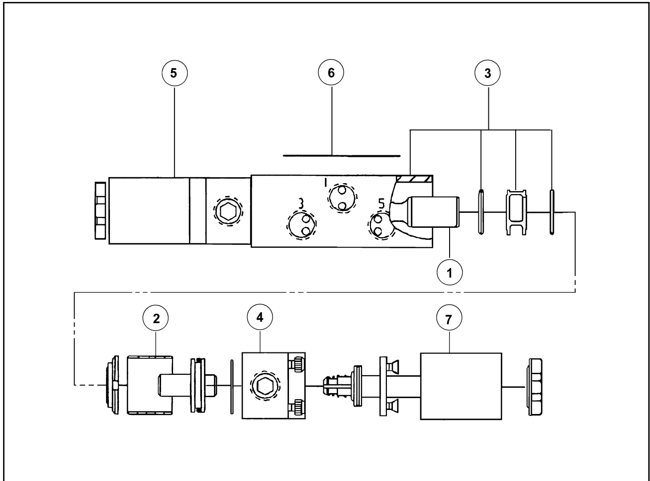
Figure 1-10 Pneumatic Valve
