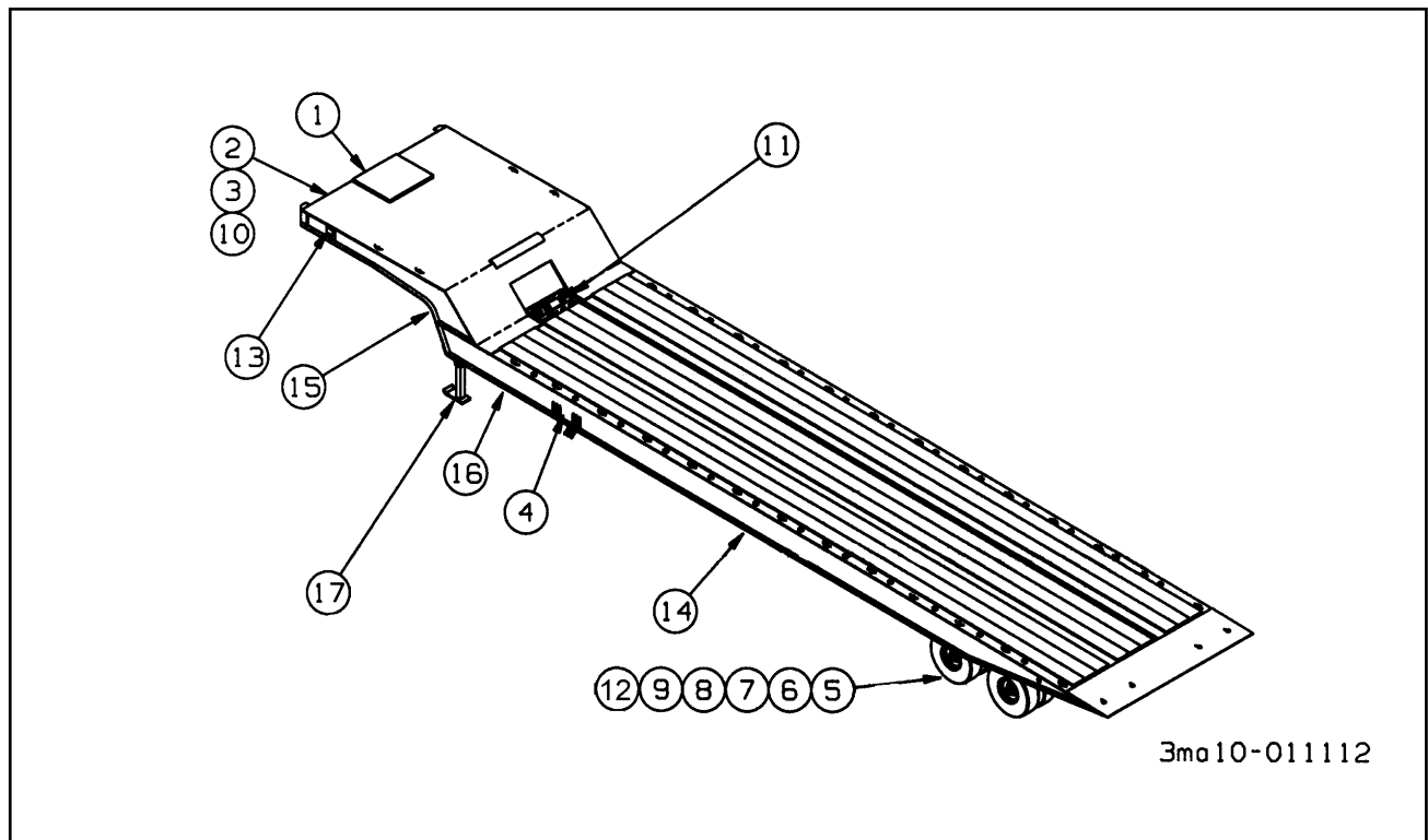
Figure 1-1 General Assembly
