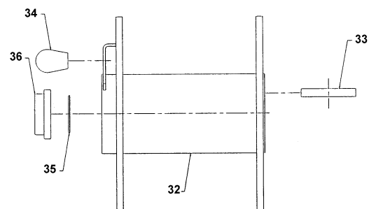
DRUM INSTALLATION
