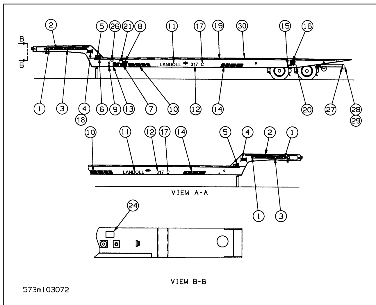
Figure 1-55 Decal Installation
