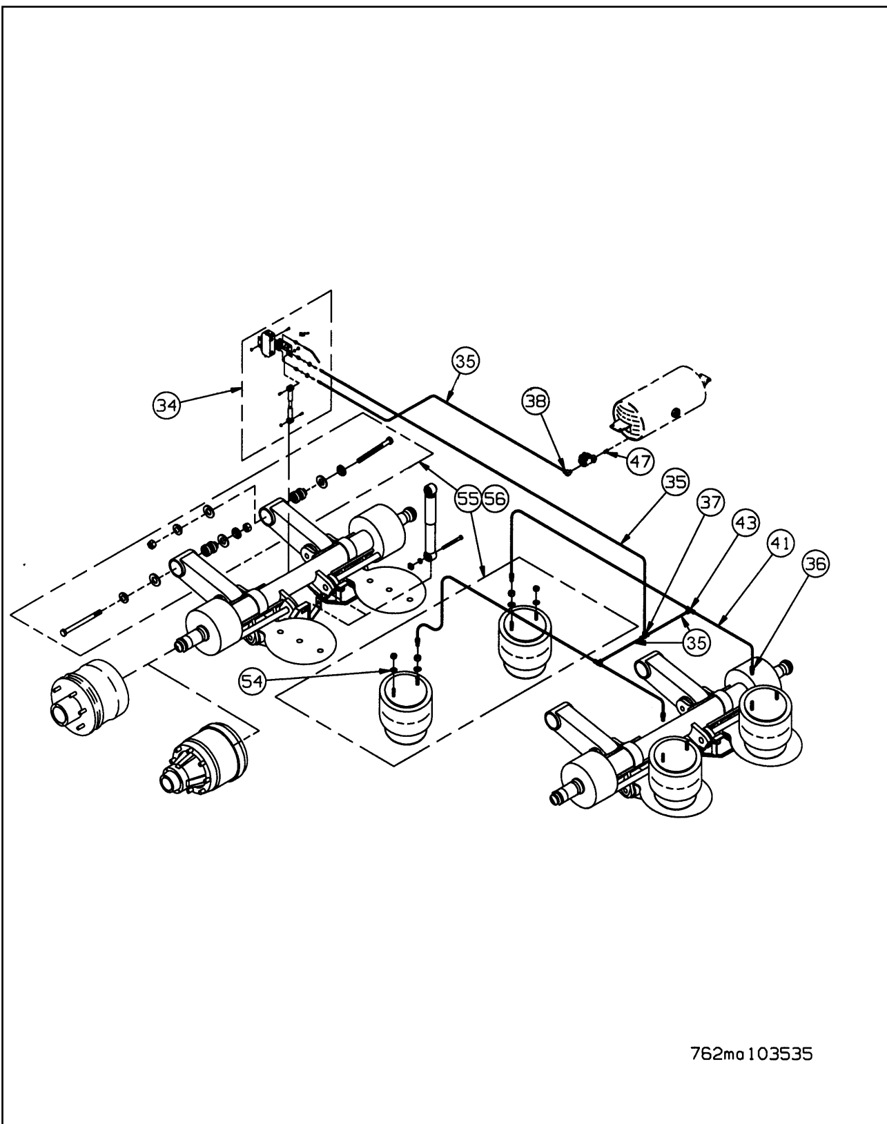
Figure 1-22 Undercarriage Suspension Air Ride (317C & 319C) (2 of 2)
