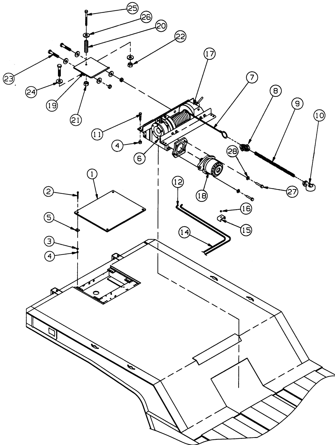
Figure 1-35 Winch Installation, Slope
