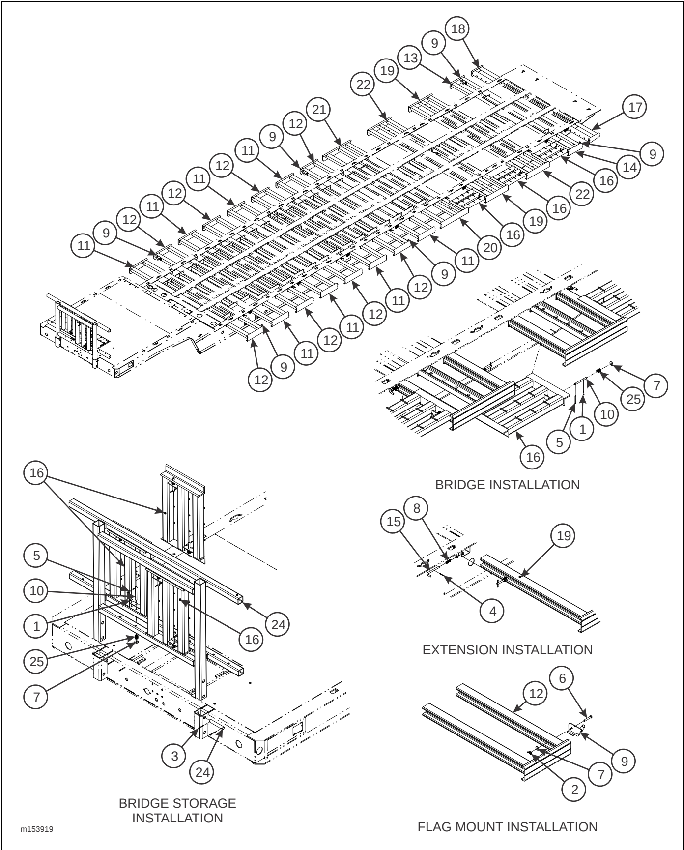
Figure 2-43: Pullout Extension Installation (318-53)
