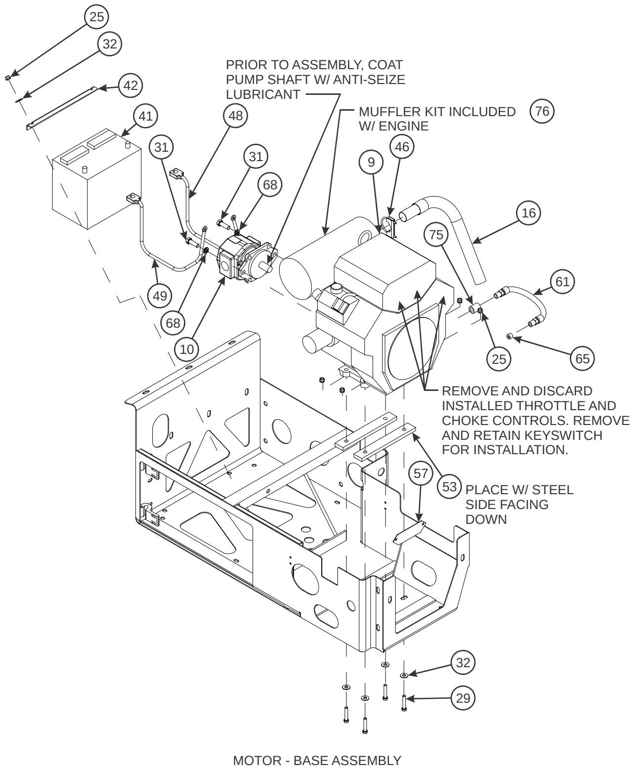
Figure 2-83: Upper Deck Engine Installation (2 of 4)
