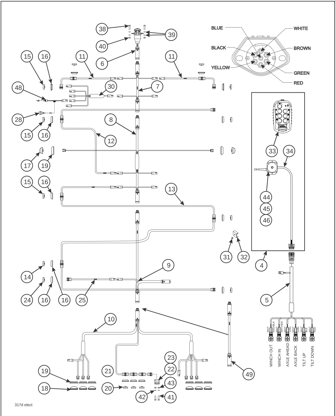
Figure 2-19: Electrical System
