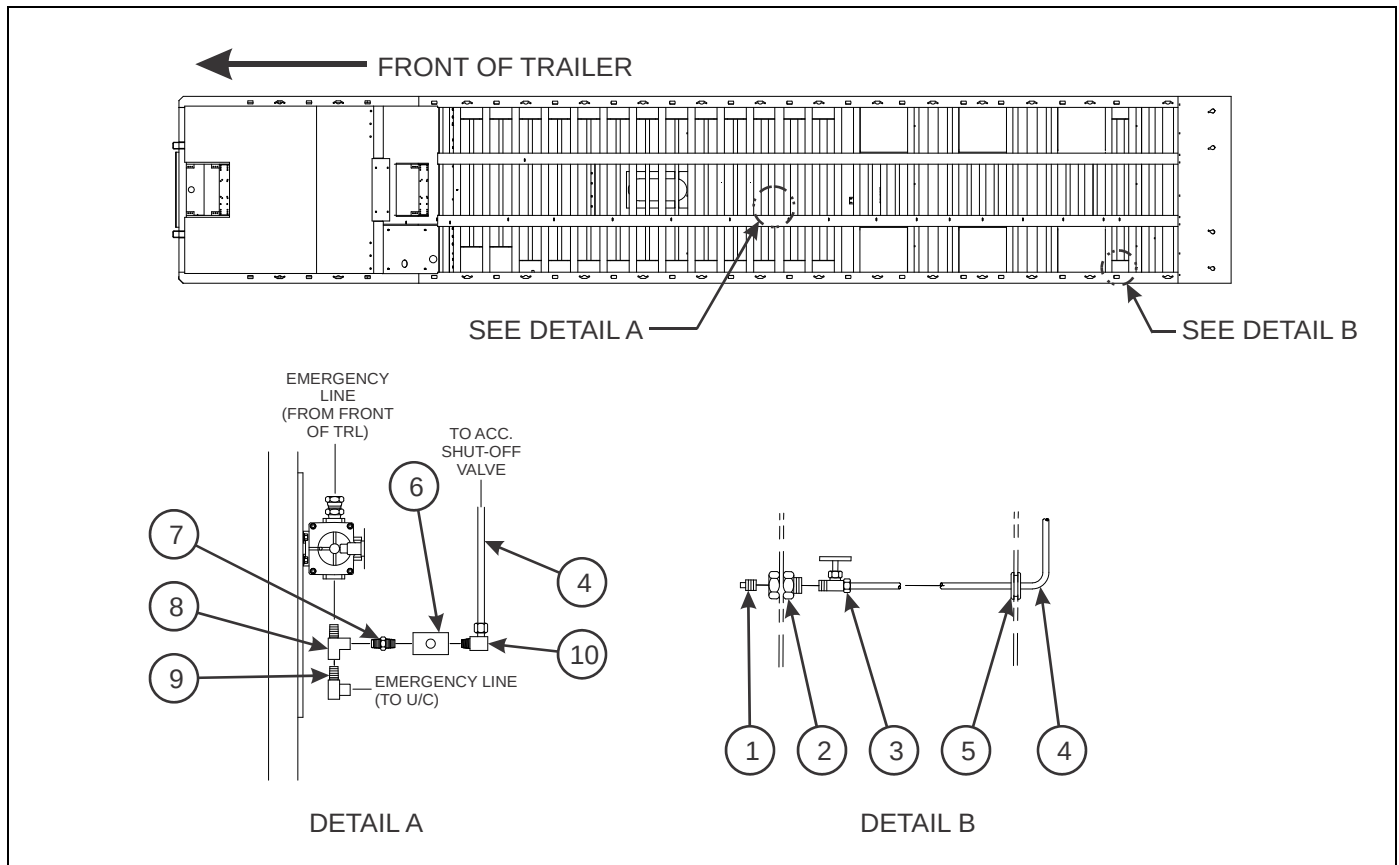
Figure 2-90: Air Outlet Accessory (Option)
