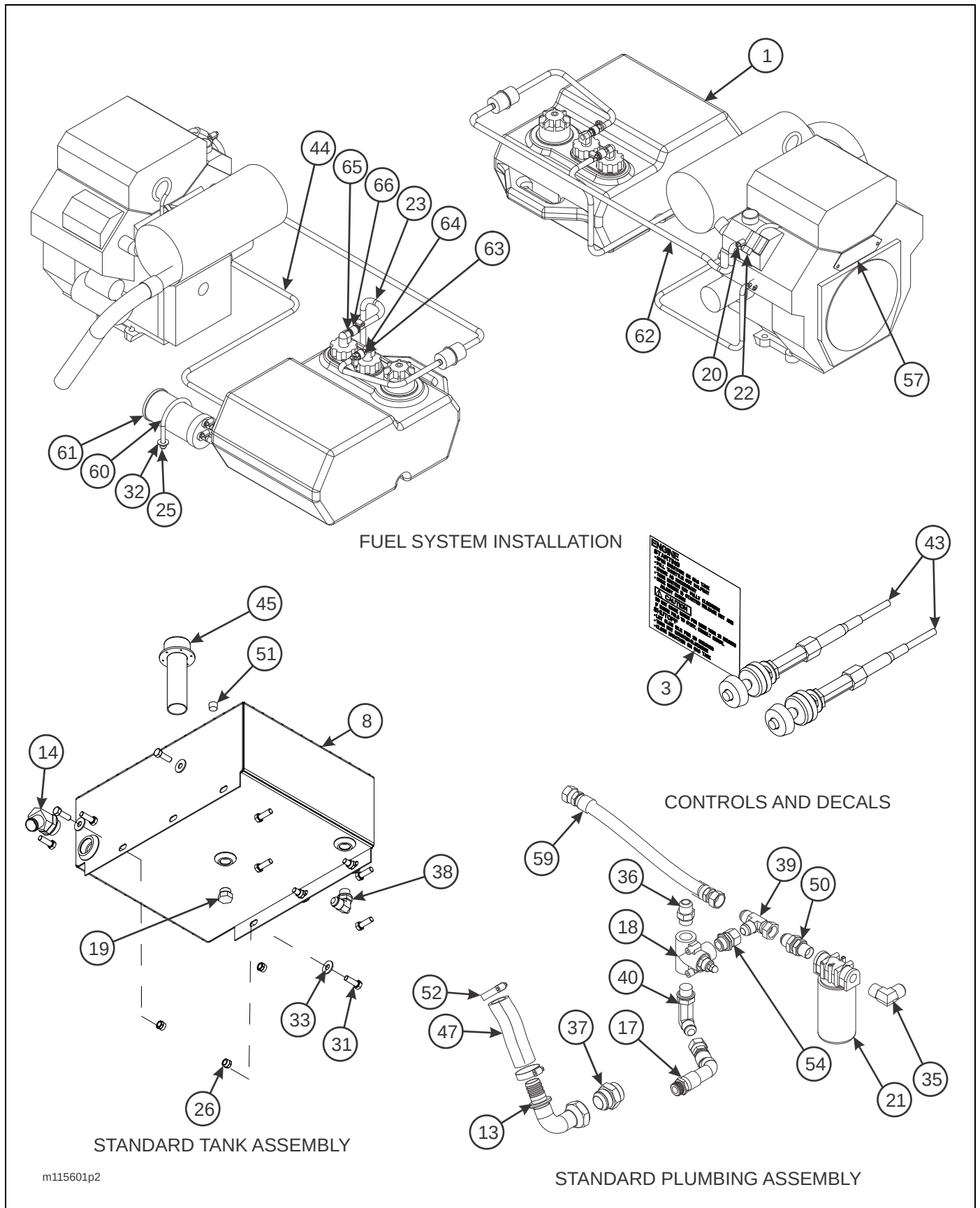
Figure 2-80: Upper Deck Engine Installation (2 of 2)
