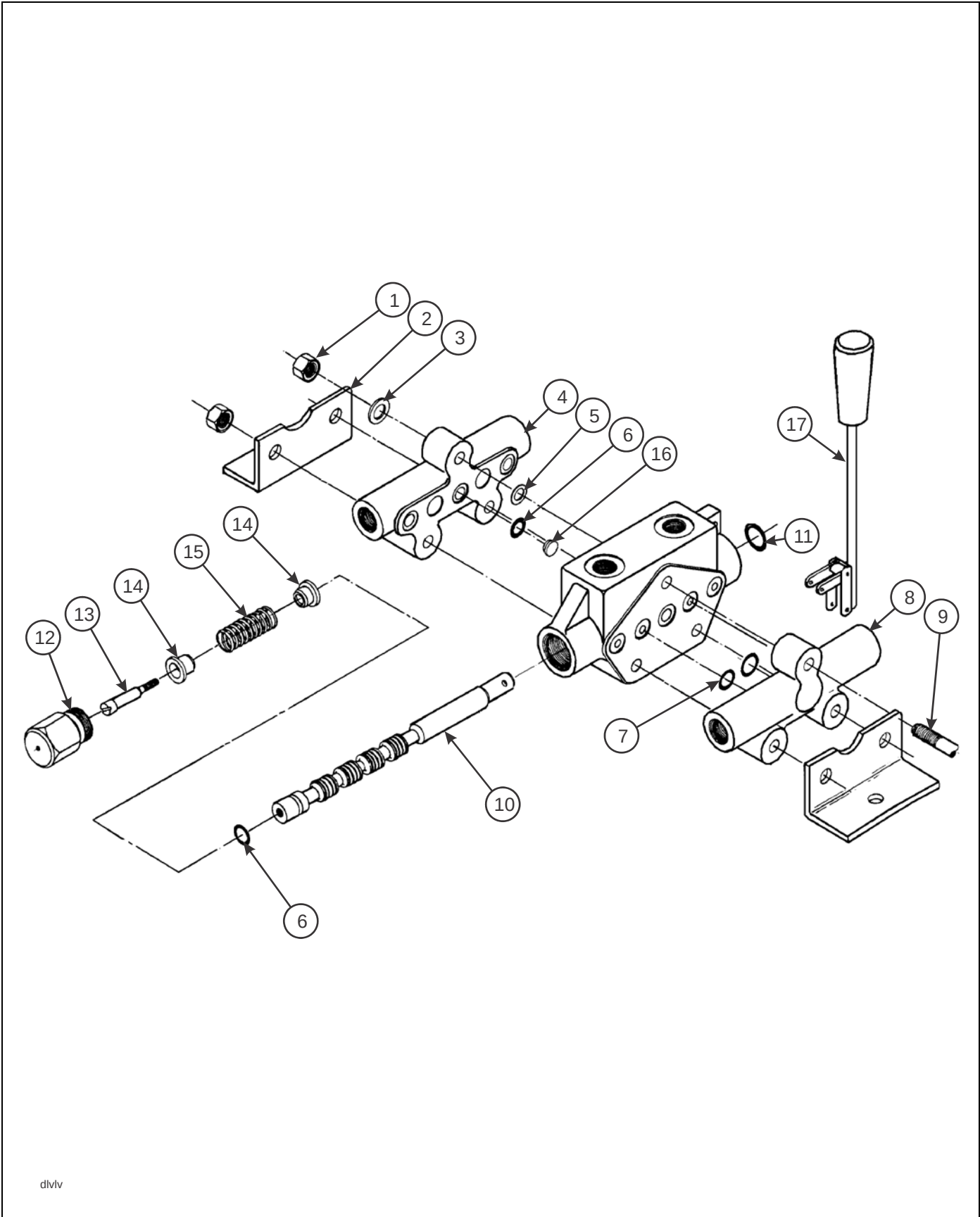
Figure 2-73: Dock Leveler Valve
