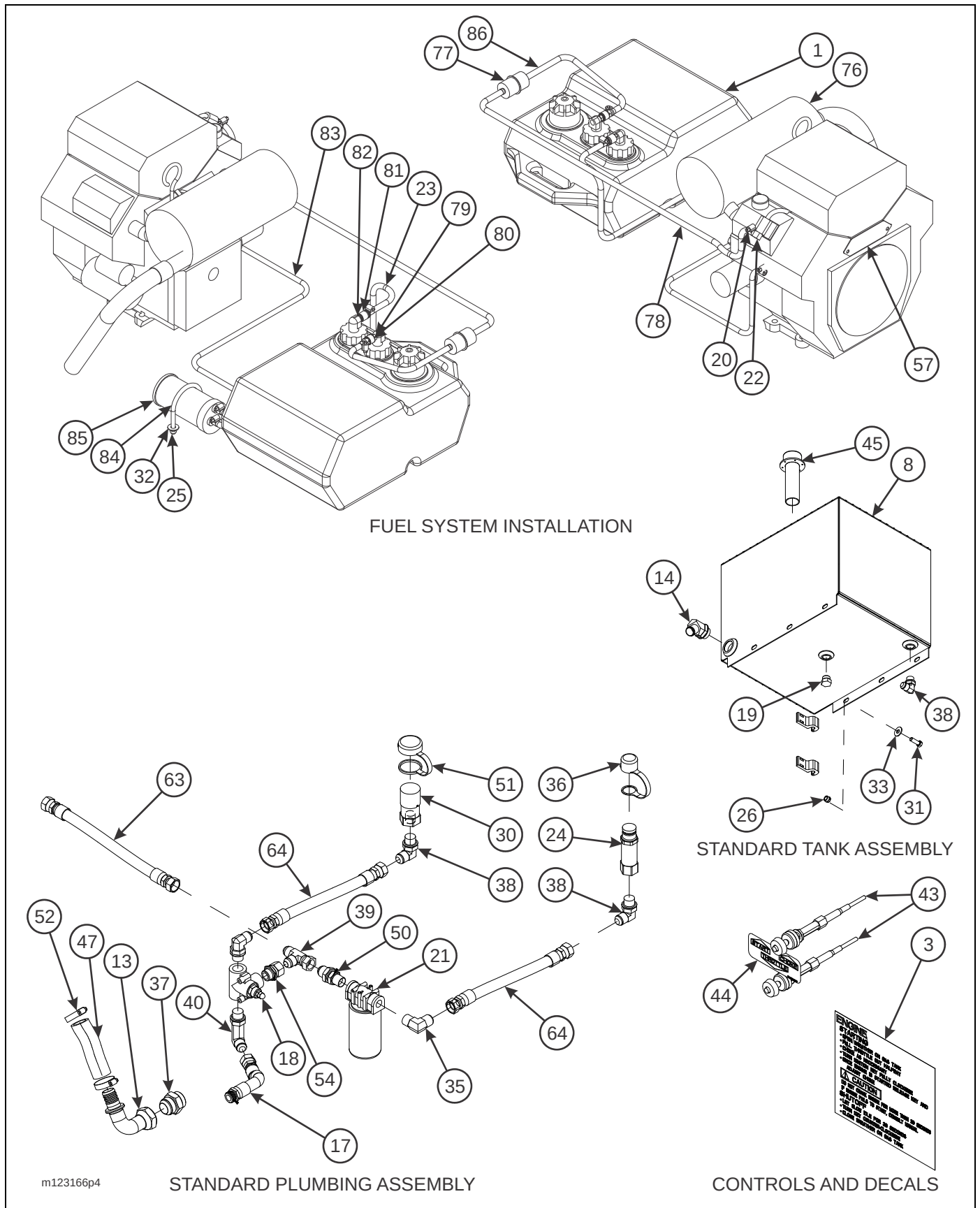
Figure 2-85: Upper Deck Engine Installation (4 of 4)
