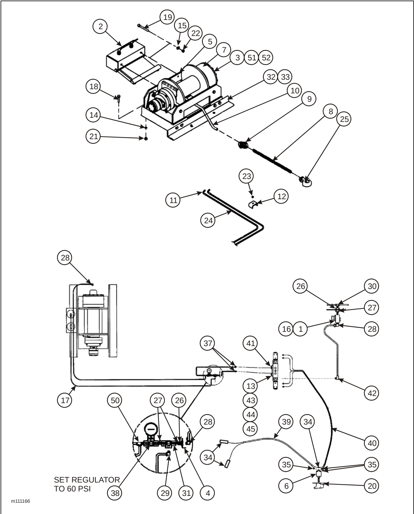
Figure 2-49: Winch Installation, 30K Air, No Remote
