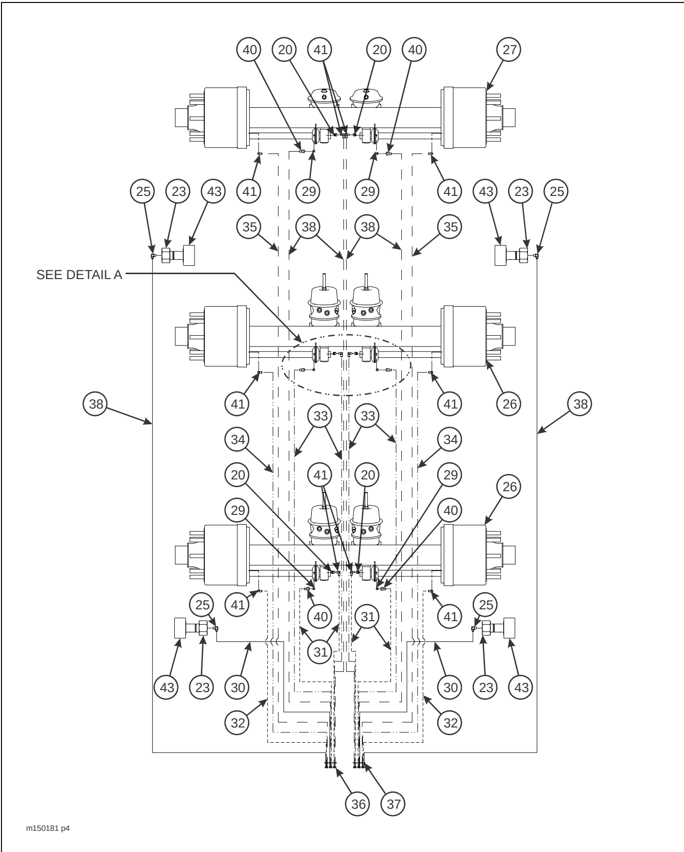
Figure 2-32: U/C Assembly, Air Ride Suspension (318D) (3 of 4)
