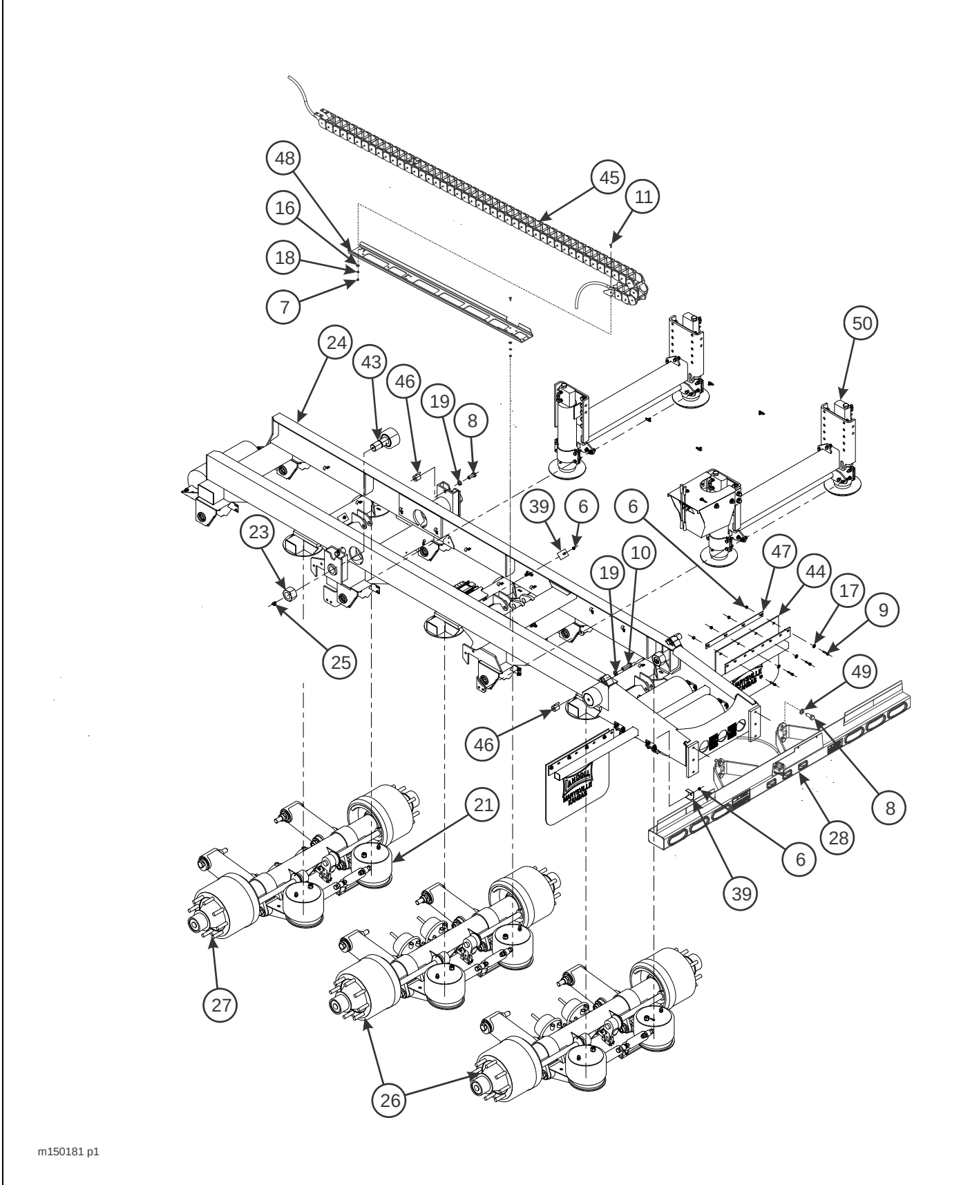
Figure 2-30: U/C Assembly, Air Ride Suspension (318D) (1 of 4)
