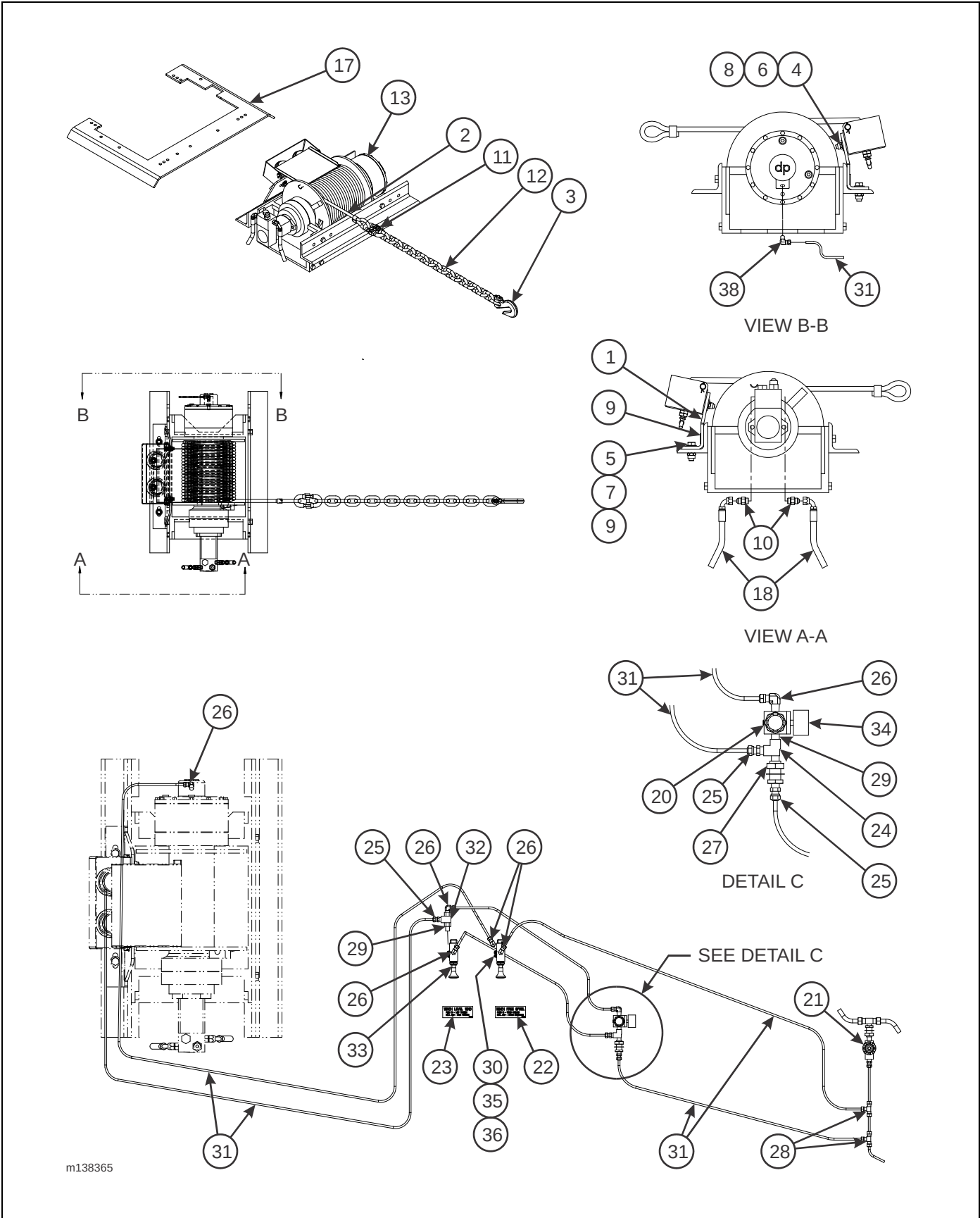
Figure 2-50: Winch Installation, 30K W/ Air Tension/Release
