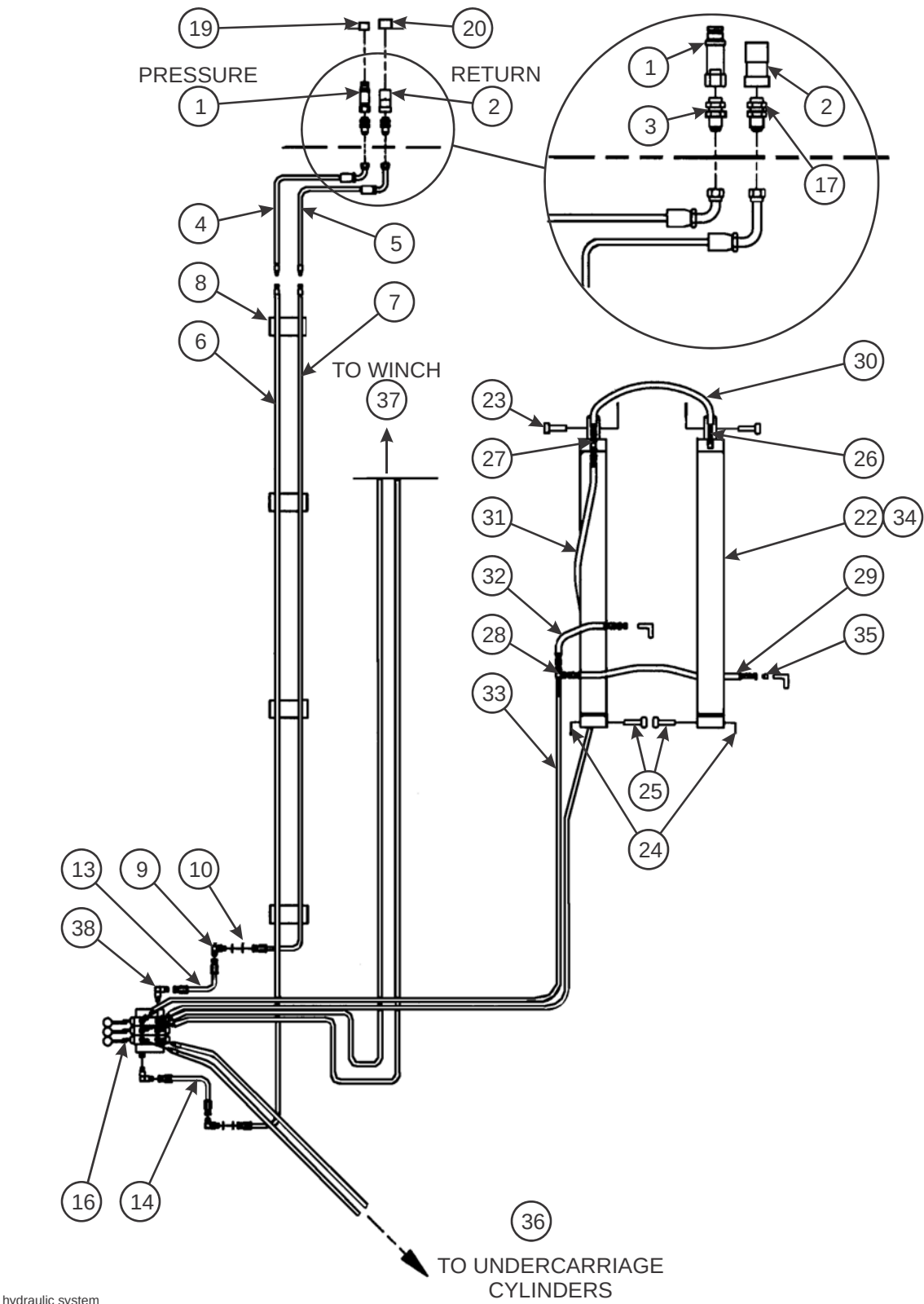
Figure 2-8: Hydraulic System
