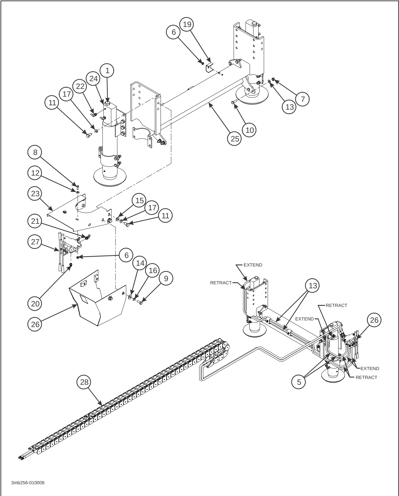
Figure 2-67: Dock Leveler Assembly, 60K (Option) (317D)
