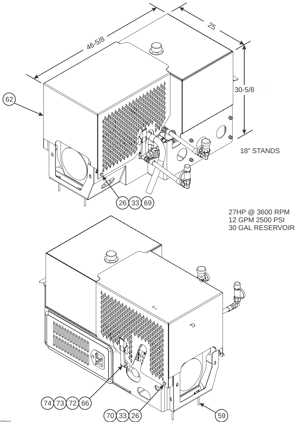
Figure 2-82: Upper Deck Engine Installation (1 of 4)
