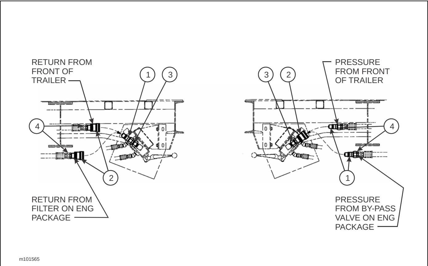
Figure 2-97: Hydraulic Dual Plumbing (Option)
