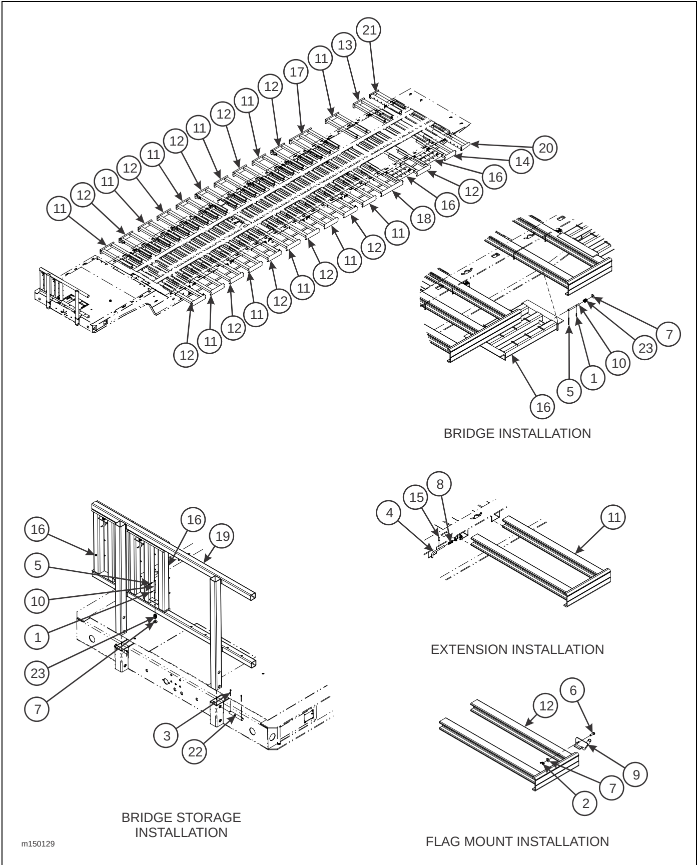
Figure 2-41: Pullout Extension Installation (317-53)
