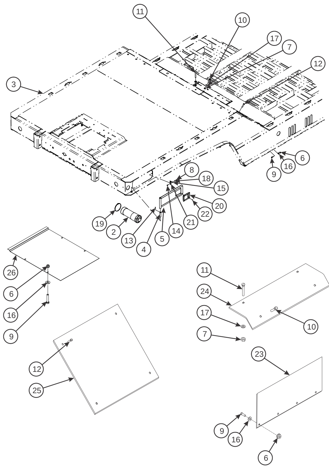
Figure 2-7: Door Latch Installation
