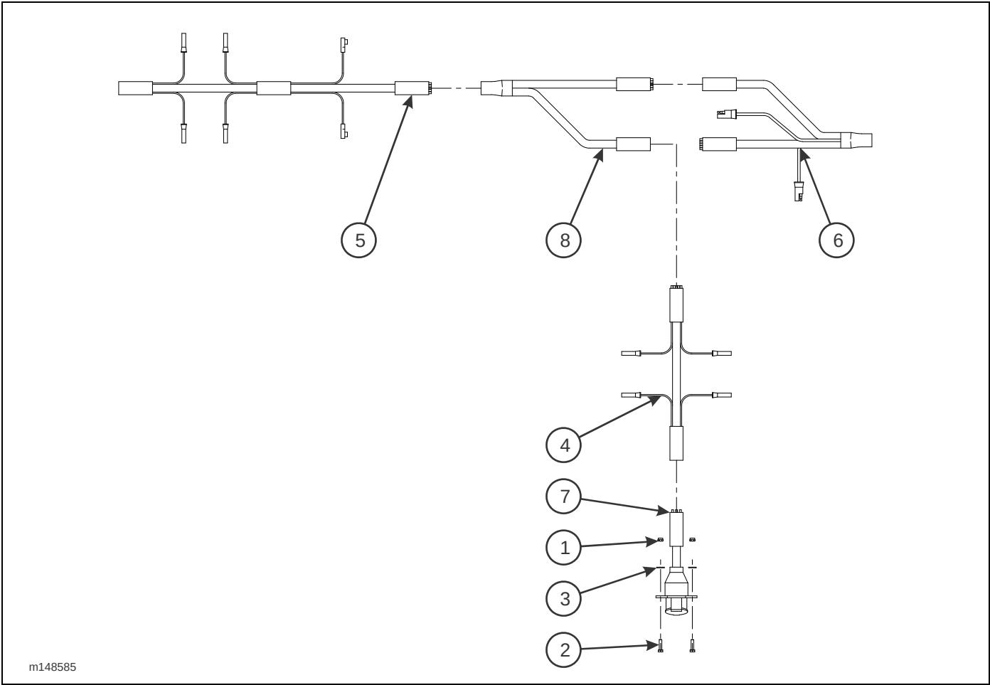
Figure 2-87: 7-Way Electrical Installation (Option)
