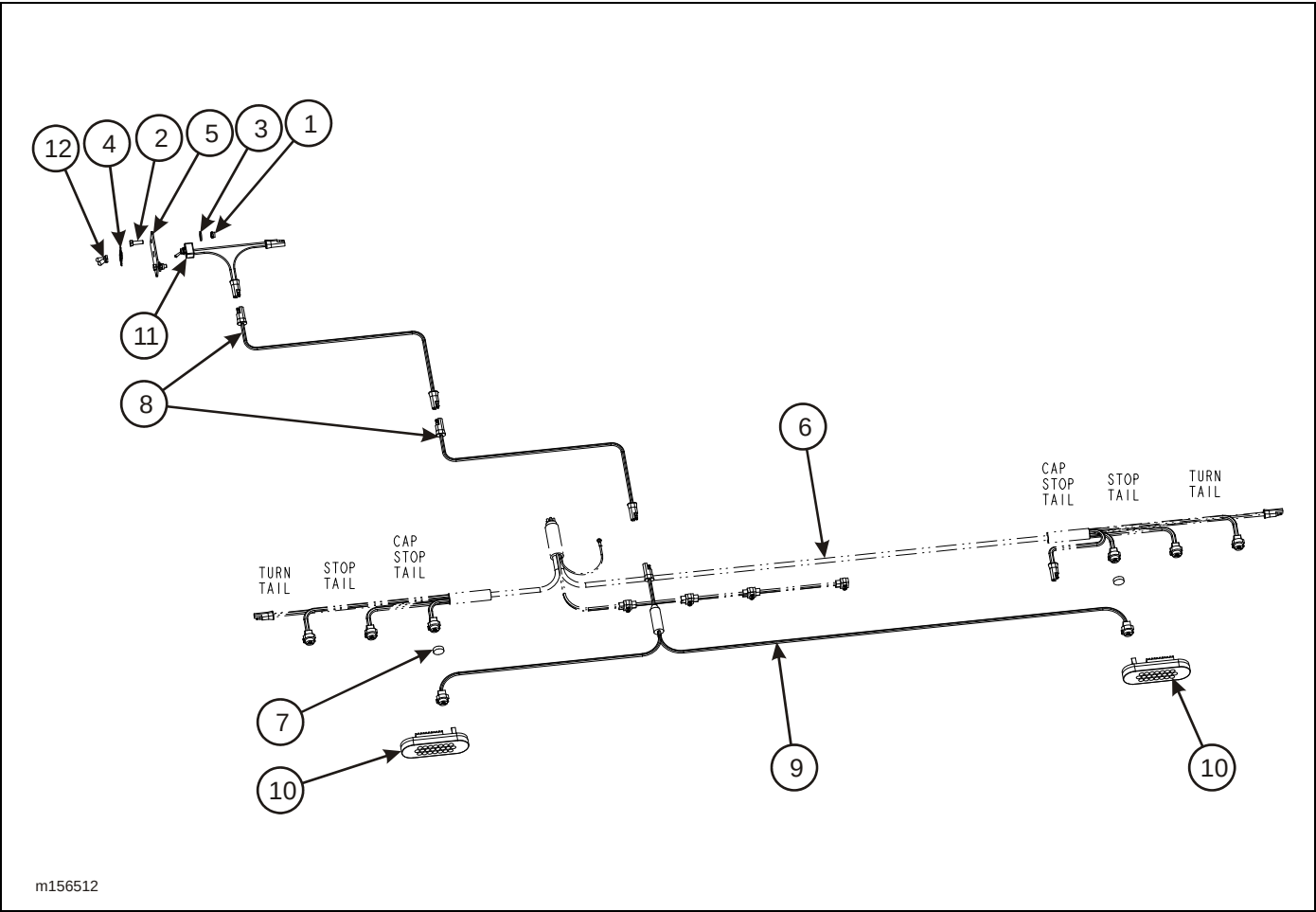
Figure 2-89: Strobe Installation, Bumper (Option)
