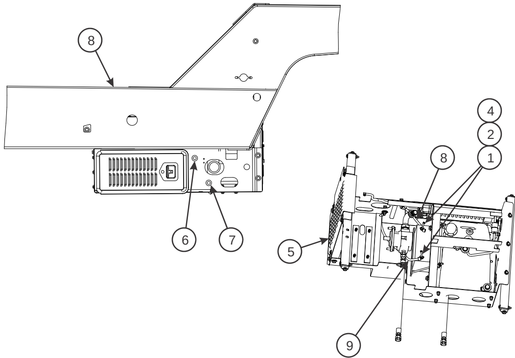
Figure 2-98: Jump Start Kit (Option)
