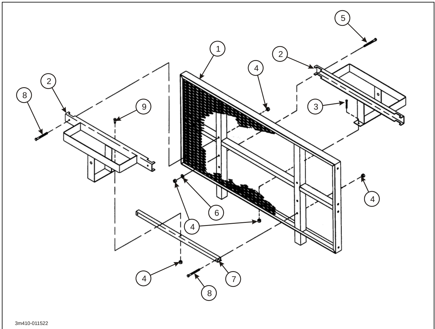
Figure 2-95: Spare Tire Carrier (Option)
