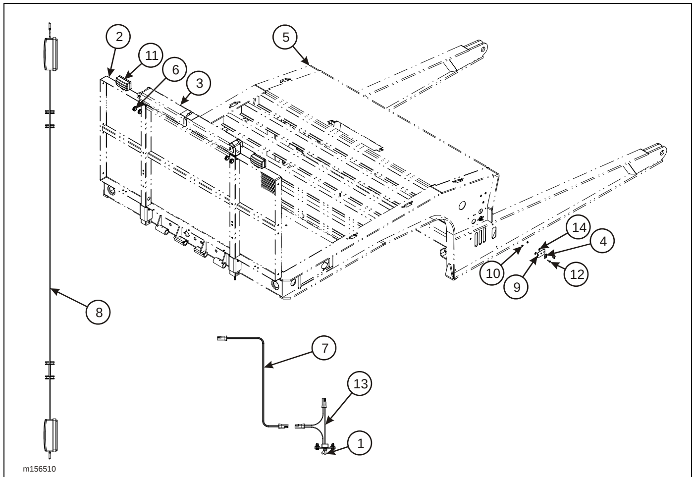
Figure 2-88: Work Light Assembly, Bulkhead (Option)
