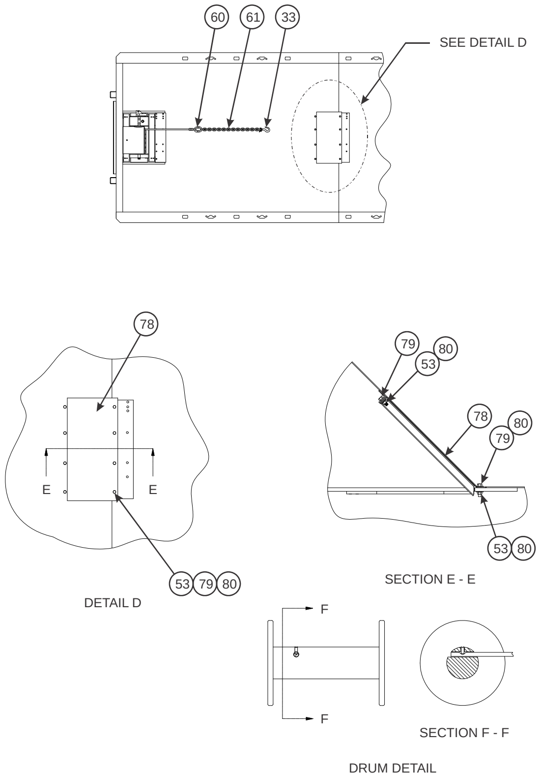
Figure 2-54: Winch Air Tension Installation, Upper Deck 20K (4 of 4)
