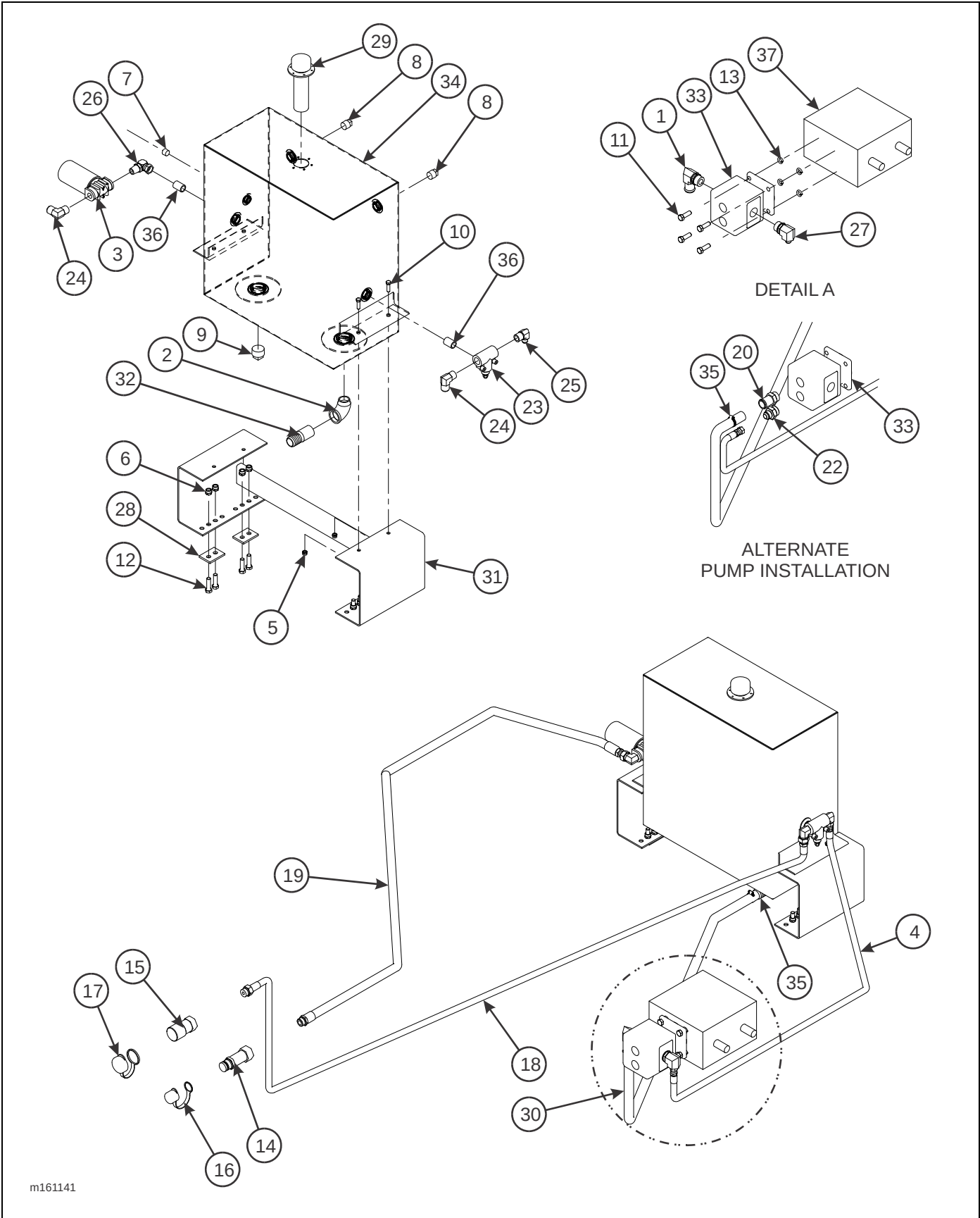
Figure 2-18: 30 Gallon Hydraulic Wet Kit Items
