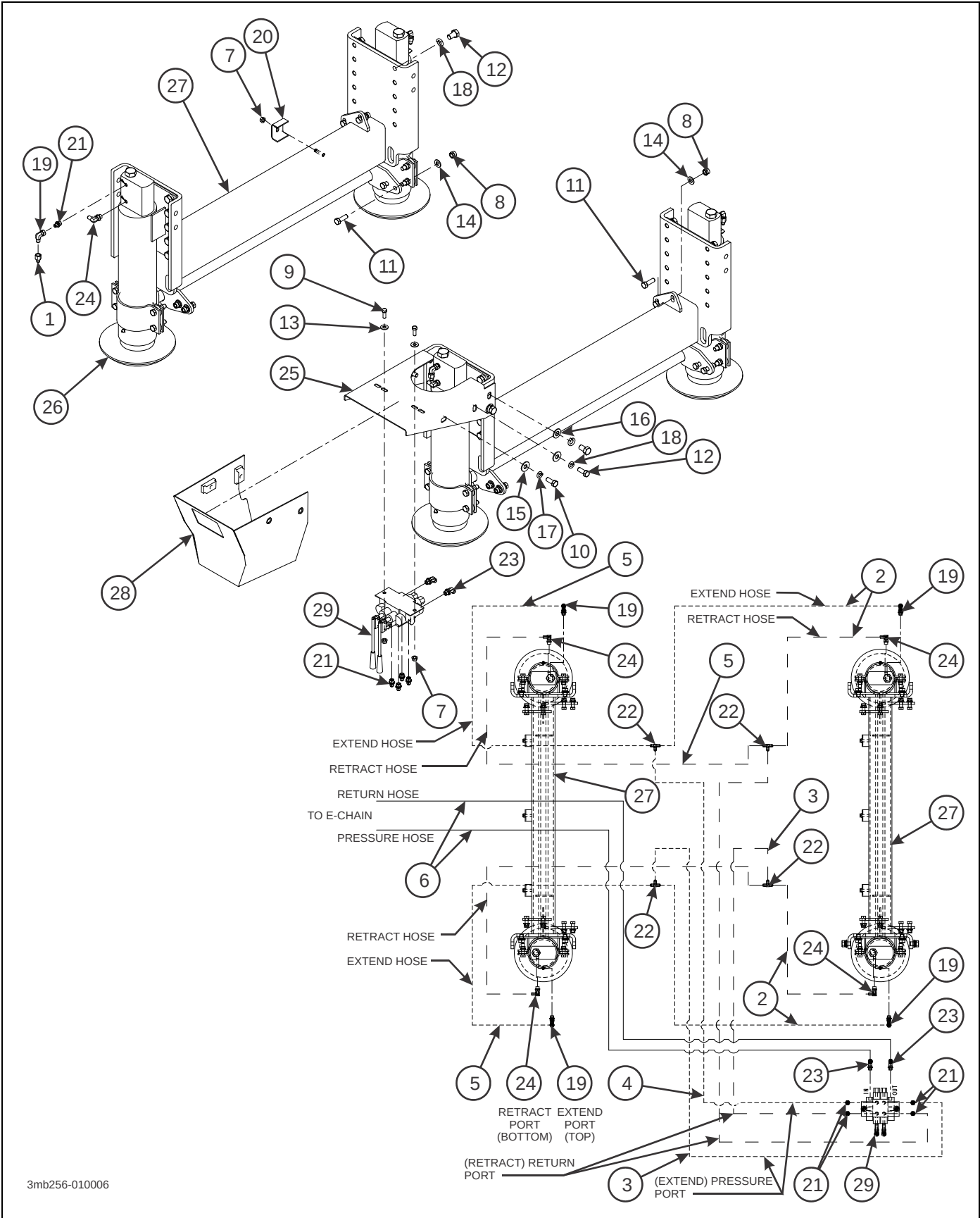
Figure 2-70: Dock Leveler Assembly, 120K
