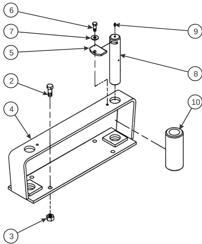
Figure 2-60: Winch Cable Roller Guide (Option)
