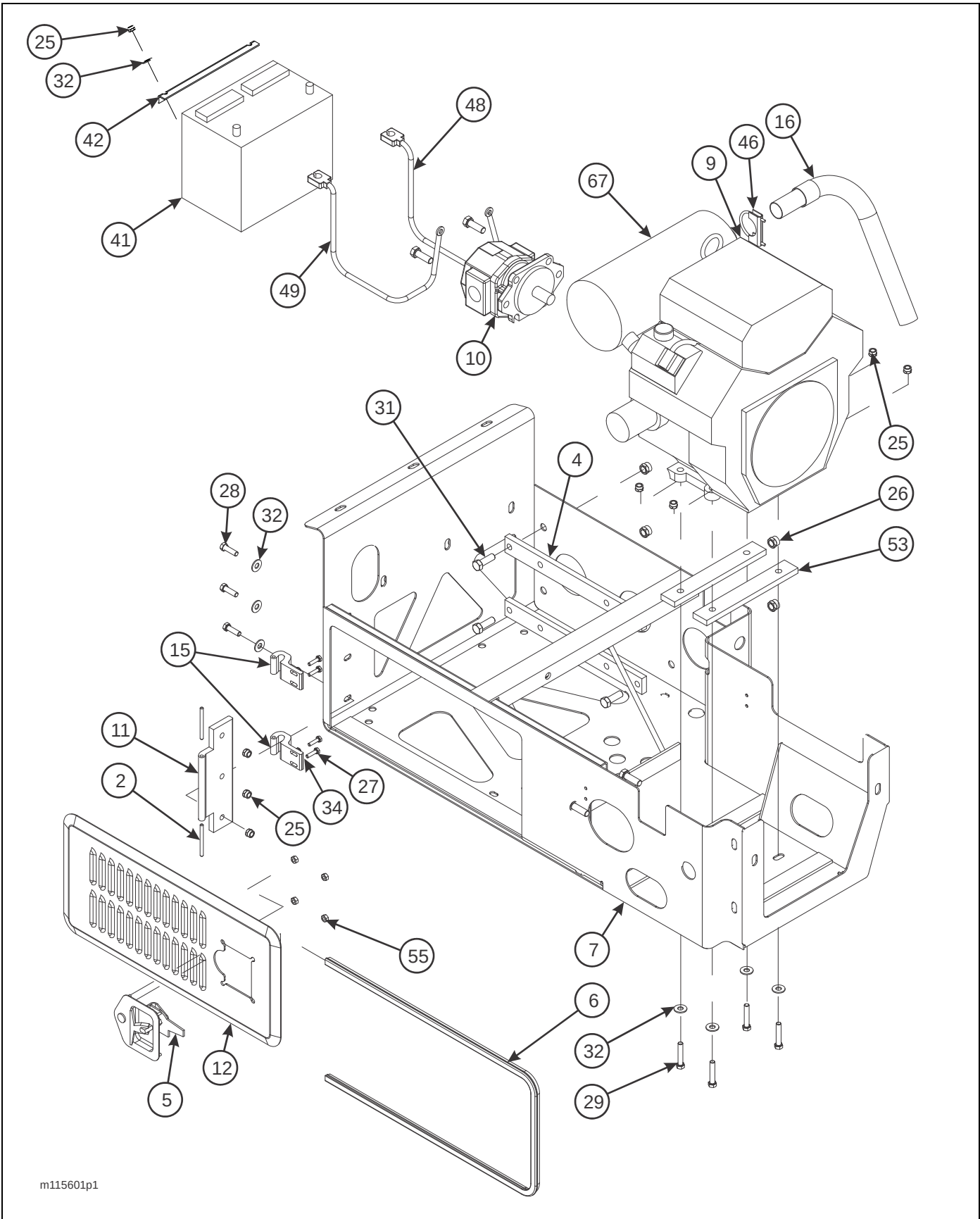
Figure 2-79: 27 HP Gas Engine Installation (1 of 2)
