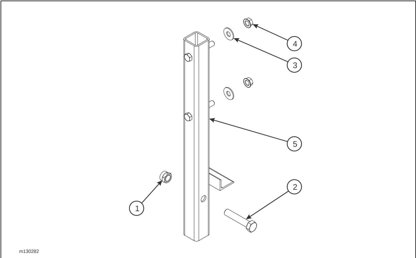
Figure 2-94: Spare Tire Mount Assembly
