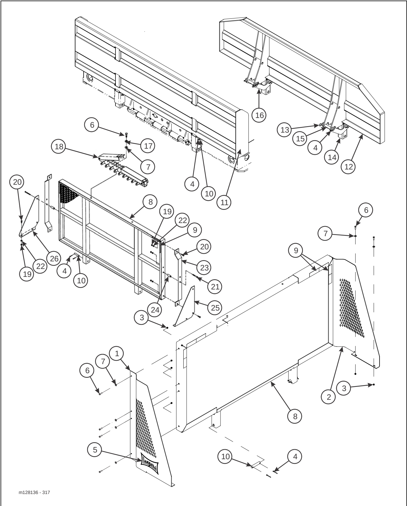
Figure 2-39: Bulkhead Assembly
