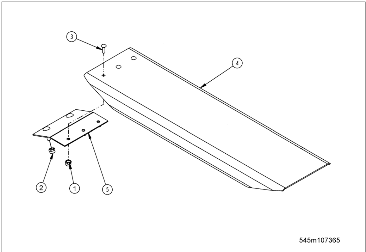
Figure 2-92: Ramps (Option)
