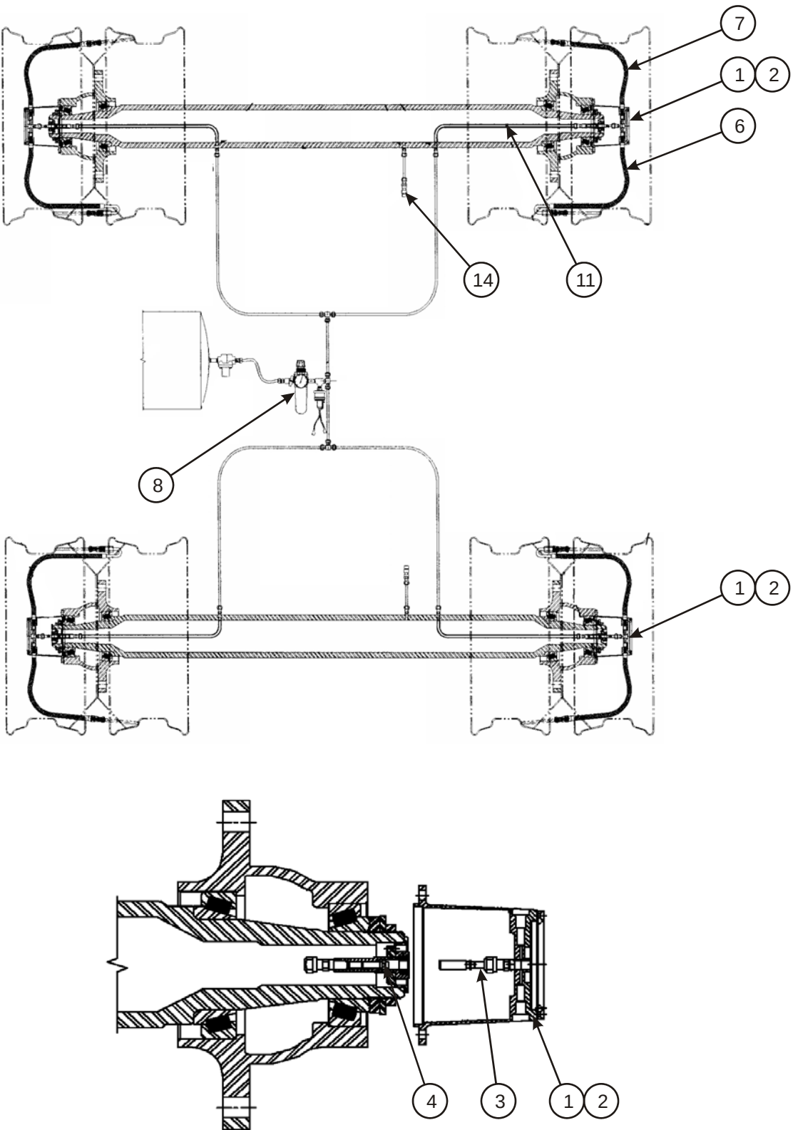
Figure 2-93: Tire Inflation System (Option)
