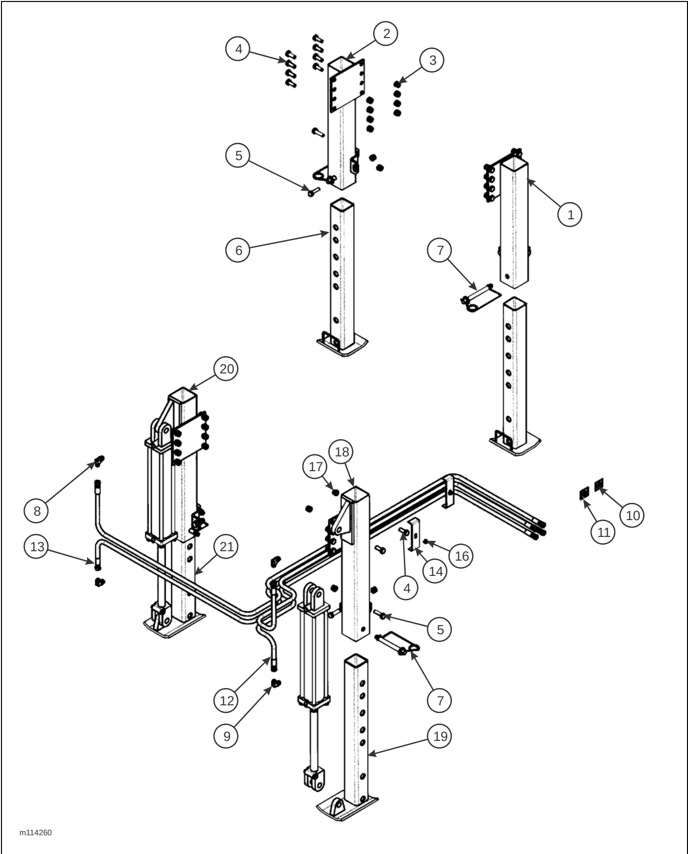
Figure 2-77: Landing Gear Installation - Bolt-On
