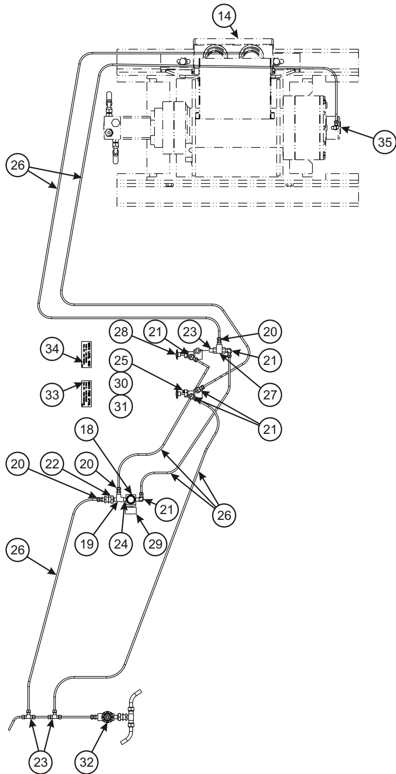
FIGURE 1-29 WINCH INSTALLATION 30K, AIR RELEASE, AIR TENSION (3 OF 3)
