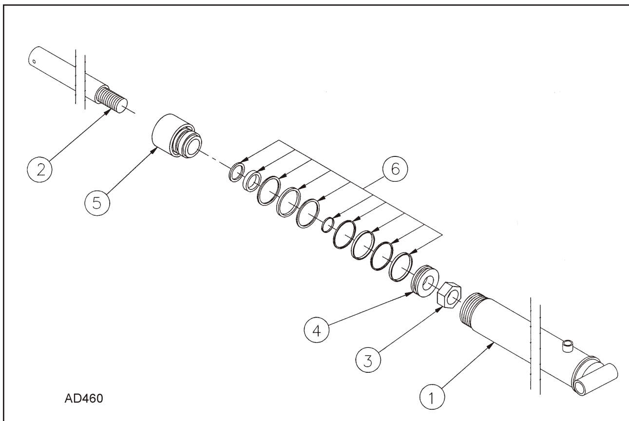
FIGURE 1-6 CYLINDER 4" X 42"
