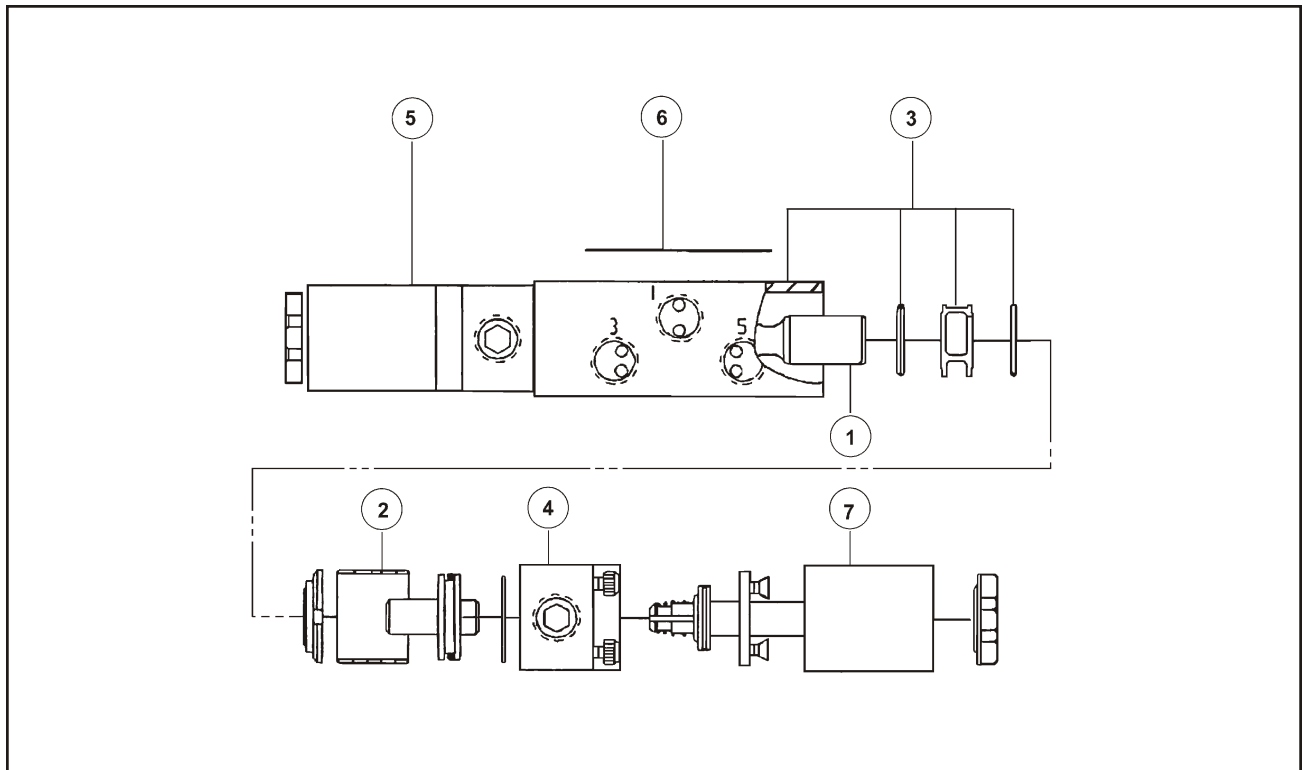
Figure 1-10 Pneumatic Valve
