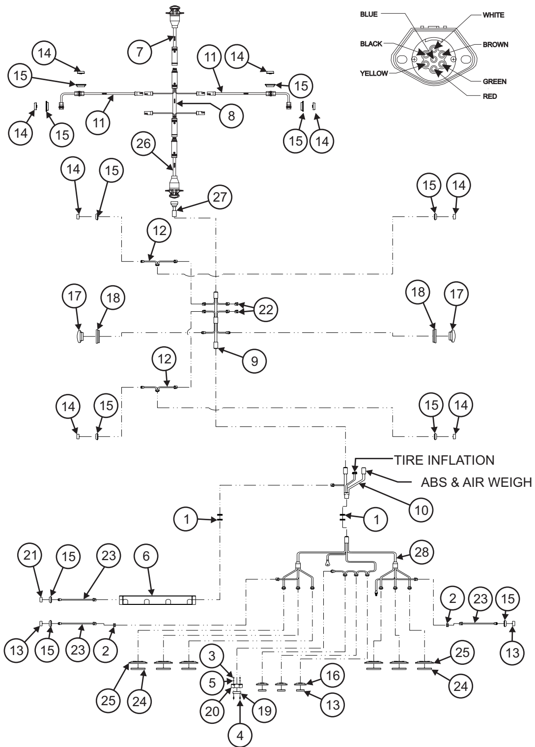
Figure 1-33 Electrical System
