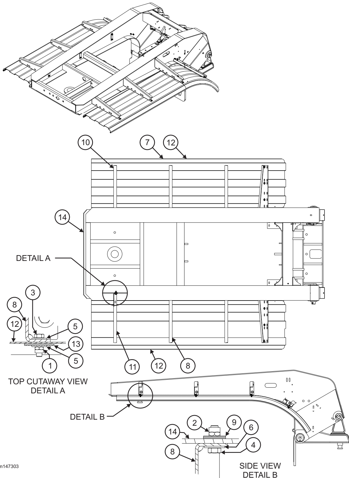
Figure 1-56 Fender Installation, 10'-7" G/N (Option)
