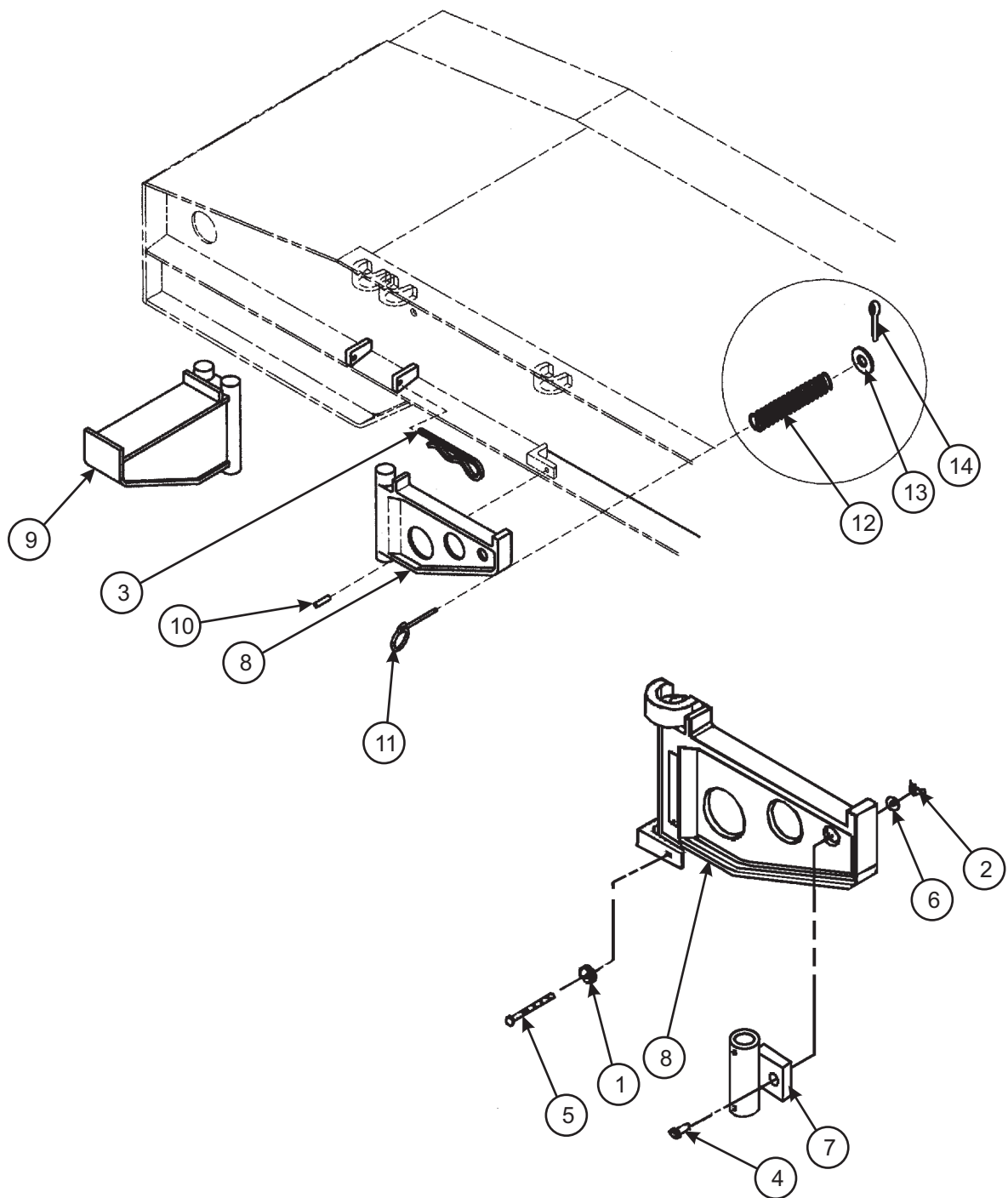
Figure 1-41 Swing Out Outrigger Installation
