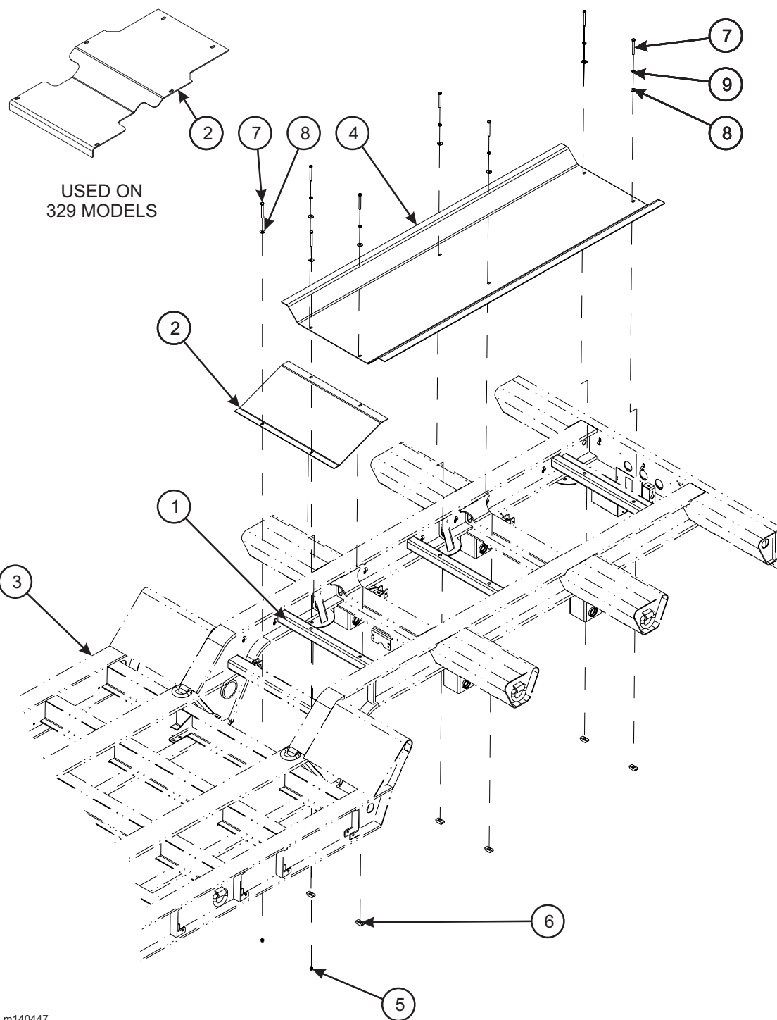
Figure 1-40 Boom Trough Cover Installation
