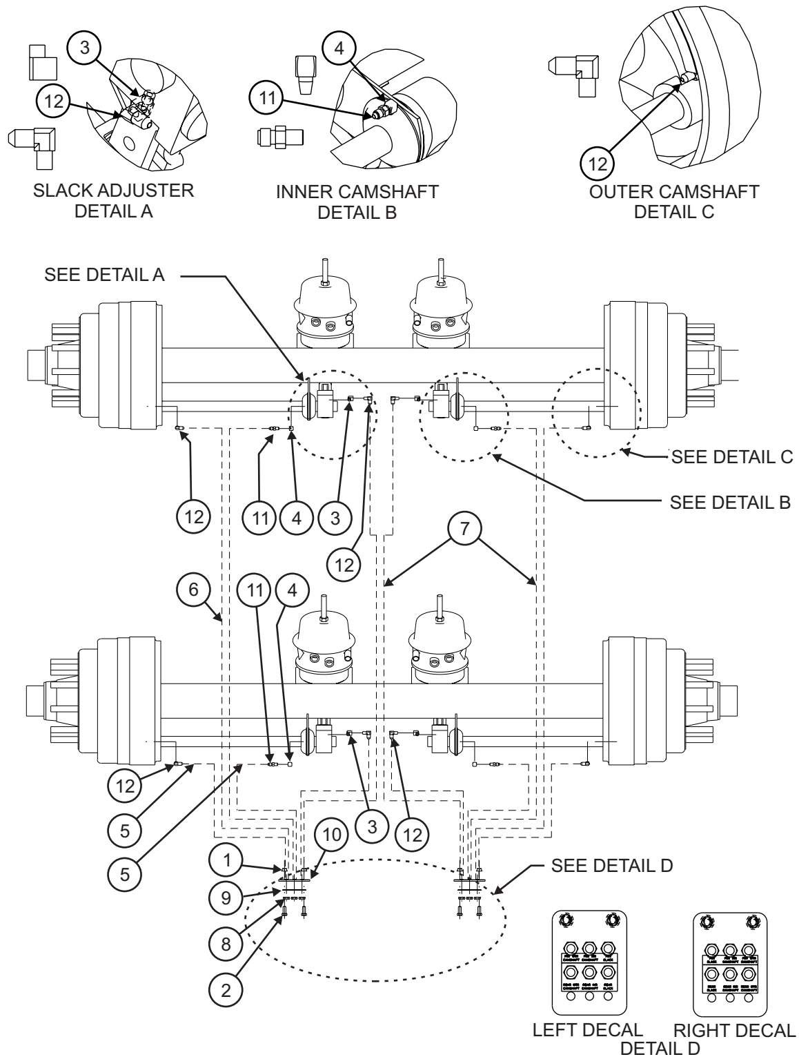
Figure 1-18 Grease System - Tandem Axle (326C)
