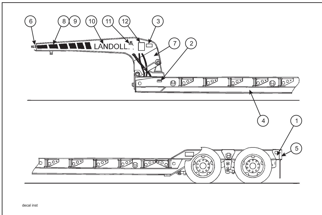
Figure 1-44 Decal Placement
