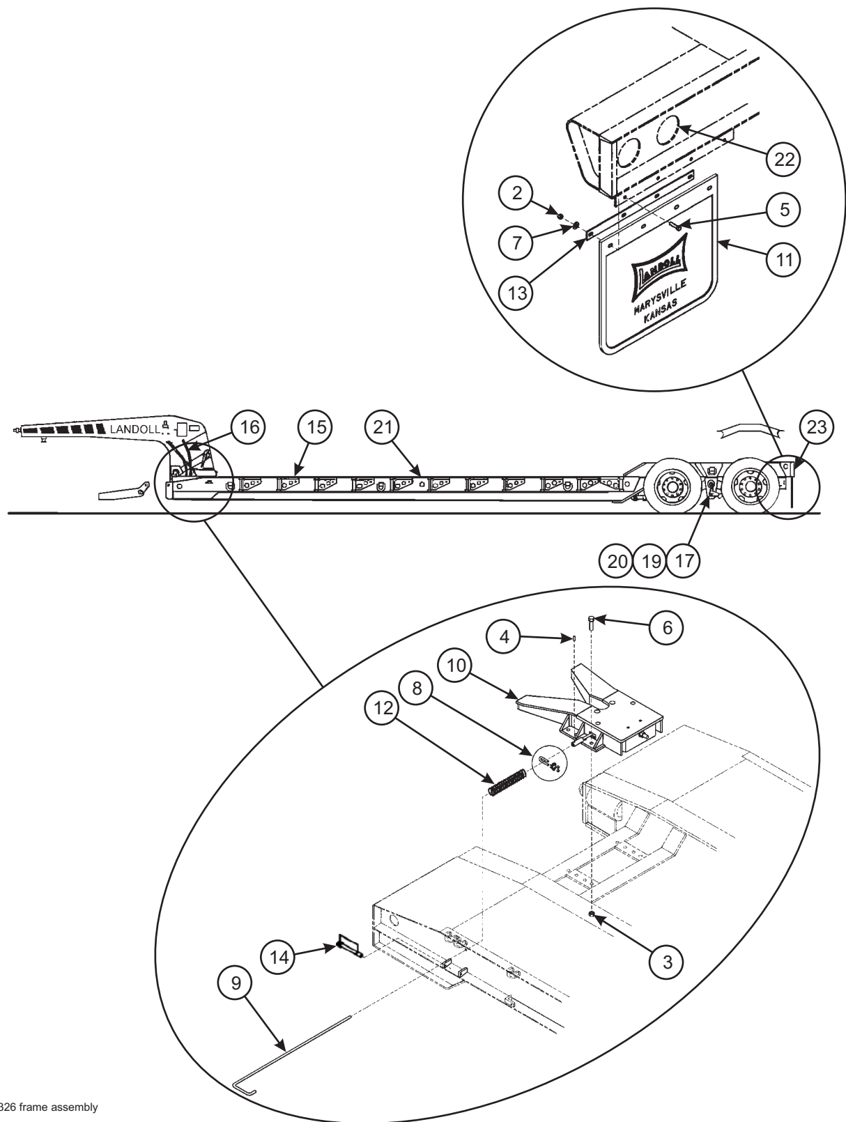
Figure 1-17 Frame Assembly, Spring Ride (326C)
