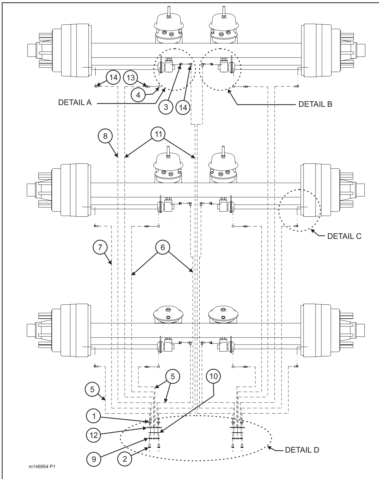
Figure 1-19 Grease System - Triple Axle (325C, 327C, 329C) (1 of 2)
