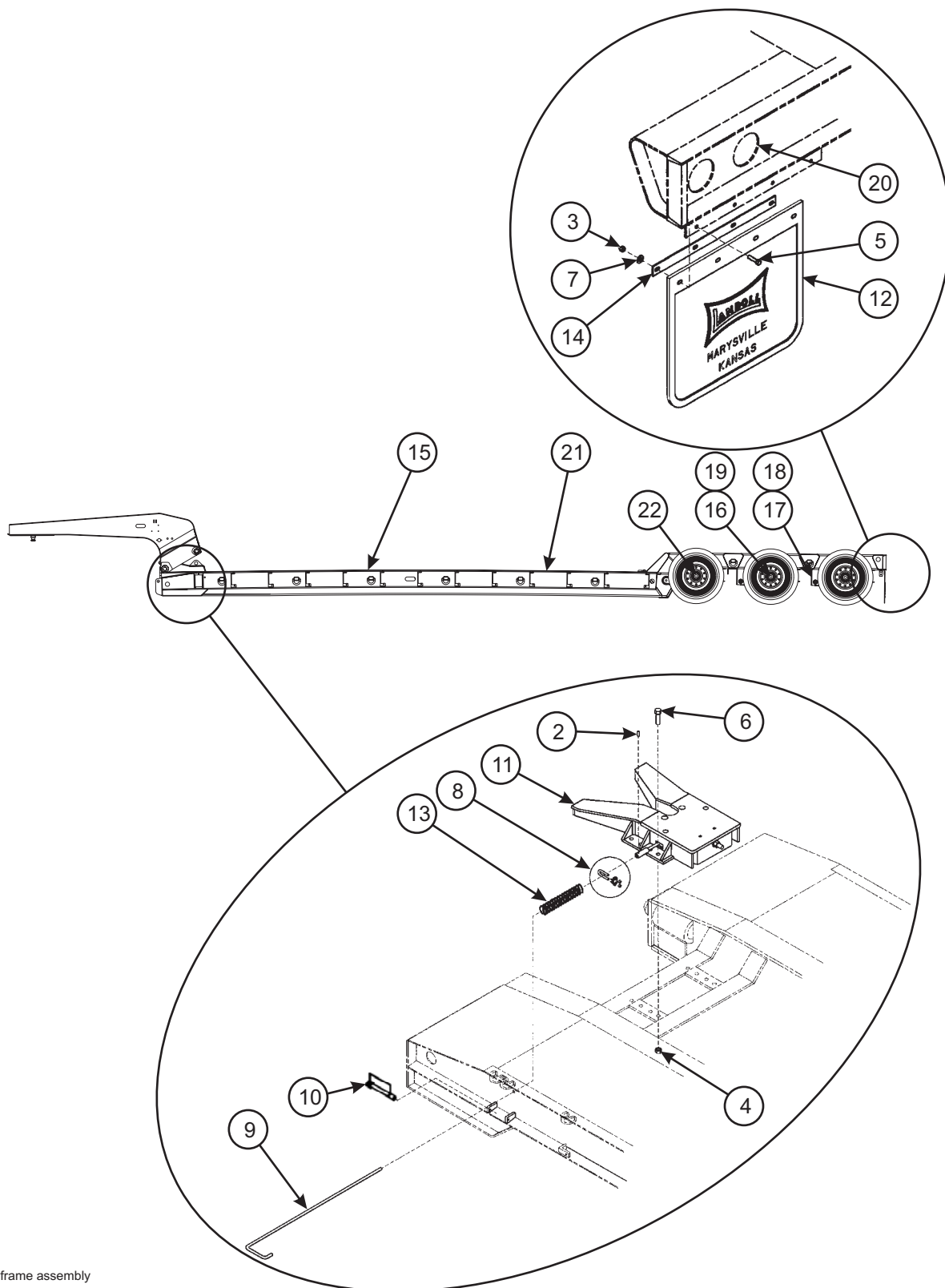
Figure 1-16 Frame Assembly, Air Ride (325C, 326C, 327C, 329C)
