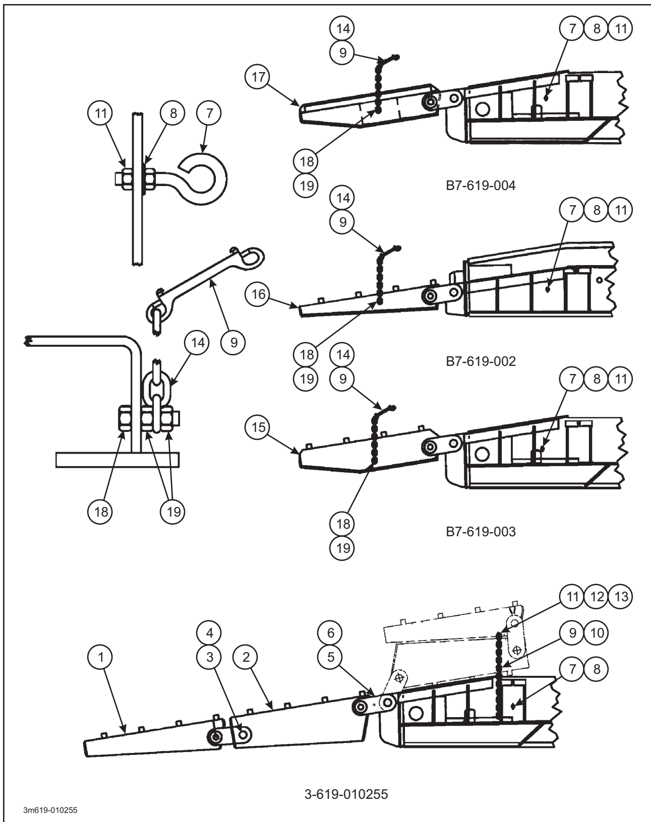
Figure 1-42 Ramp Installation
