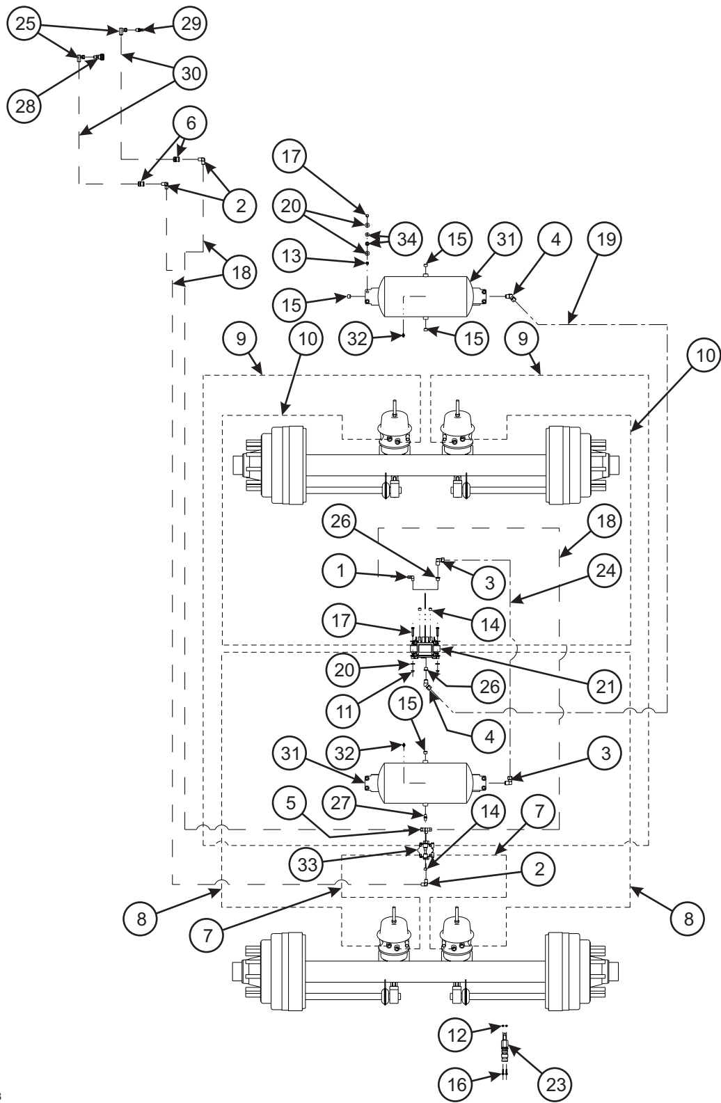
Figure 1-37 Air Brake System (326C)
