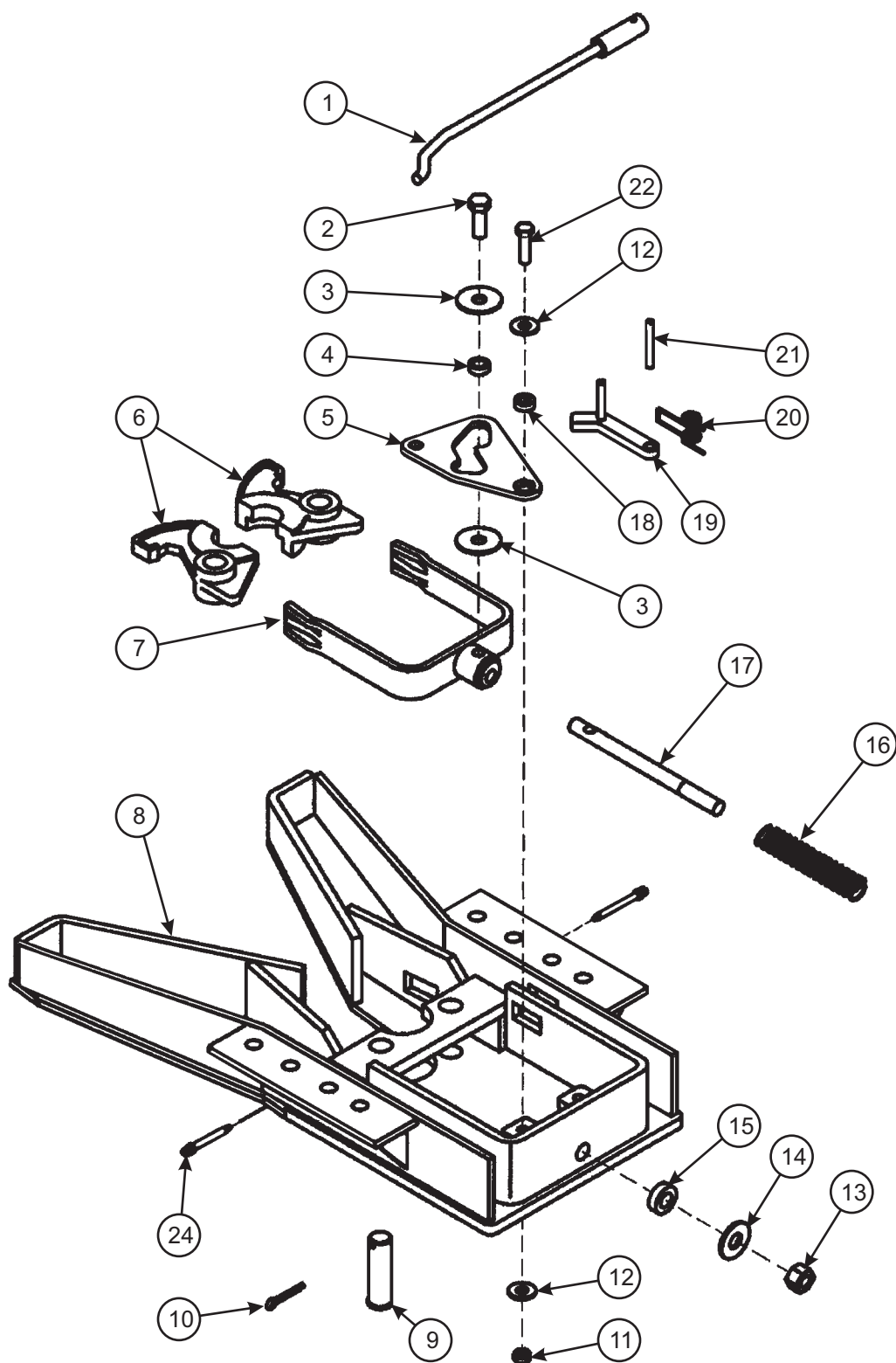
Figure 1-21 Lock Assembly
