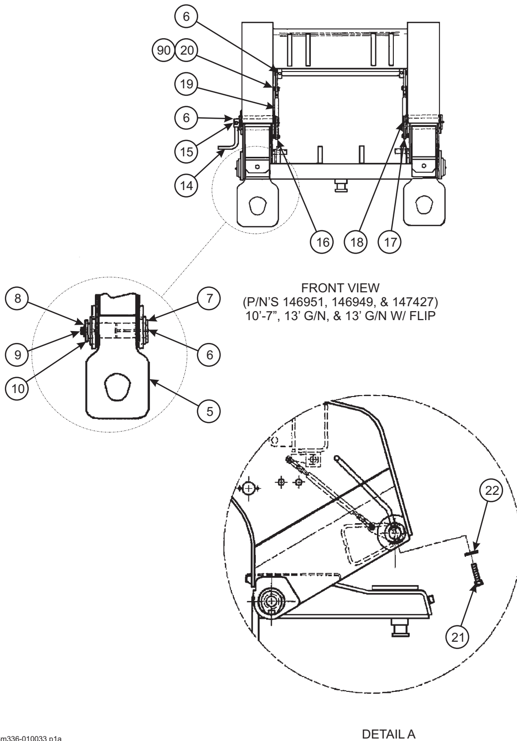
Figure 1-3 Gooseneck Assembly (2 of 5)
