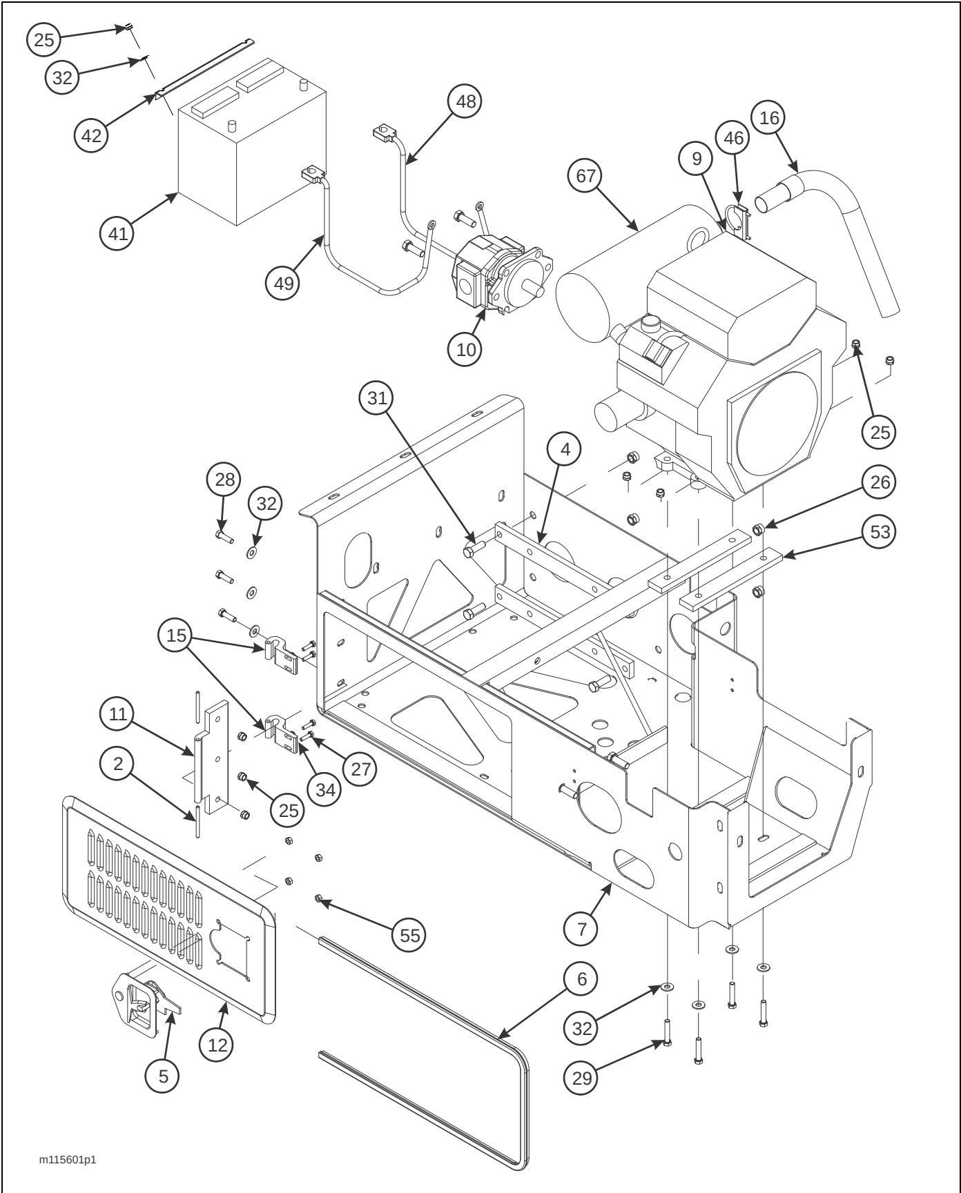
Figure 2-47: Engine Package, Front Mount (1 of 2)
