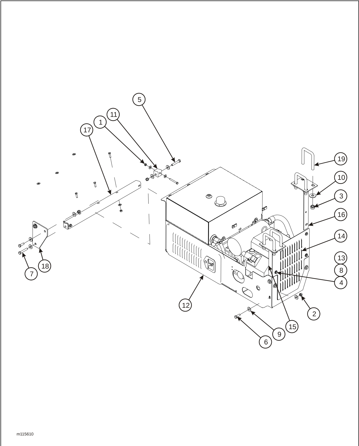
Figure 2-49: Underslung Engine Package Installation
