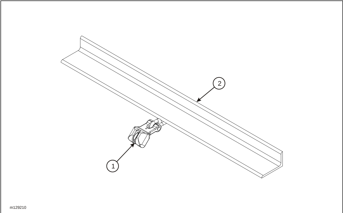
Figure 2-41: Container Pusher Assembly (Option)
