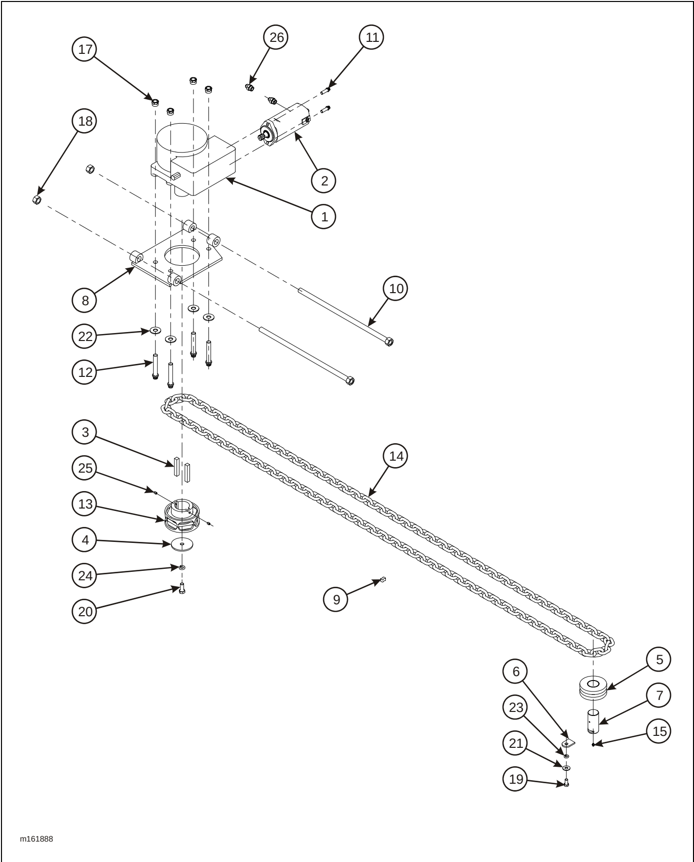
Figure 2-37: Gearbox Assembly (Chain Drive Model)
