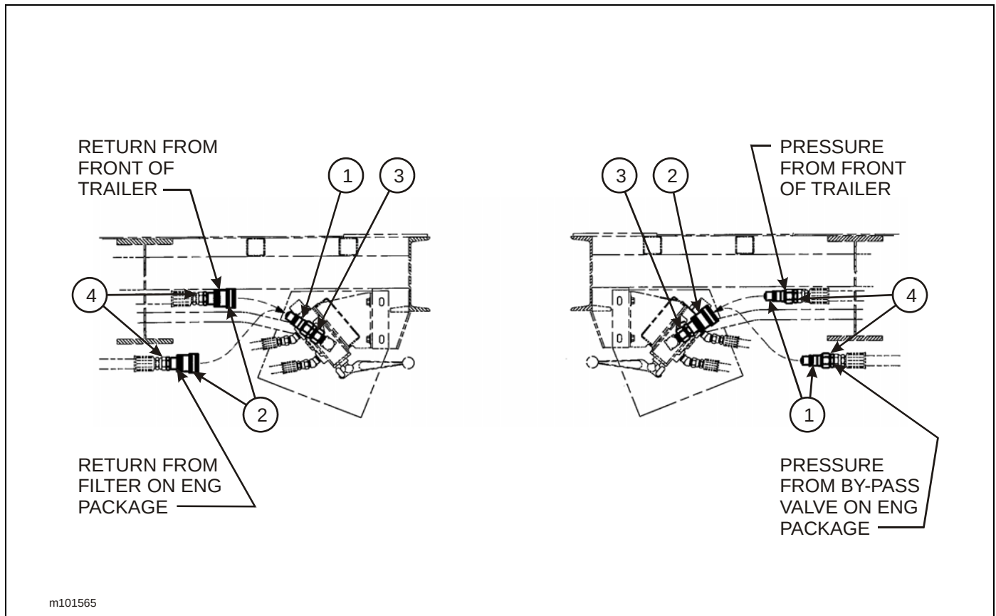
Figure 2-59: Hydraulic Dual Plumbing (Option)
