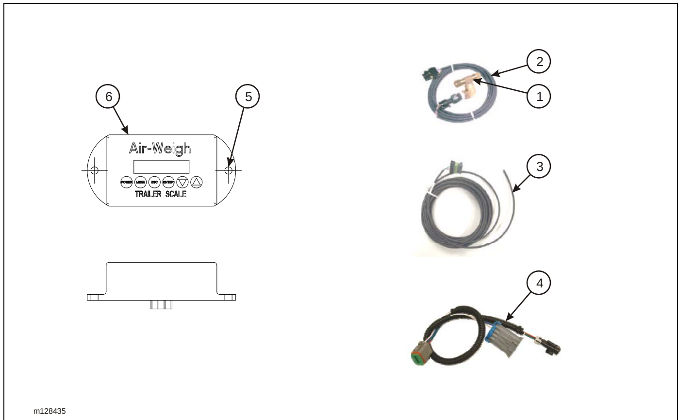
Figure 2-65: Air Digital Scale (Option)
