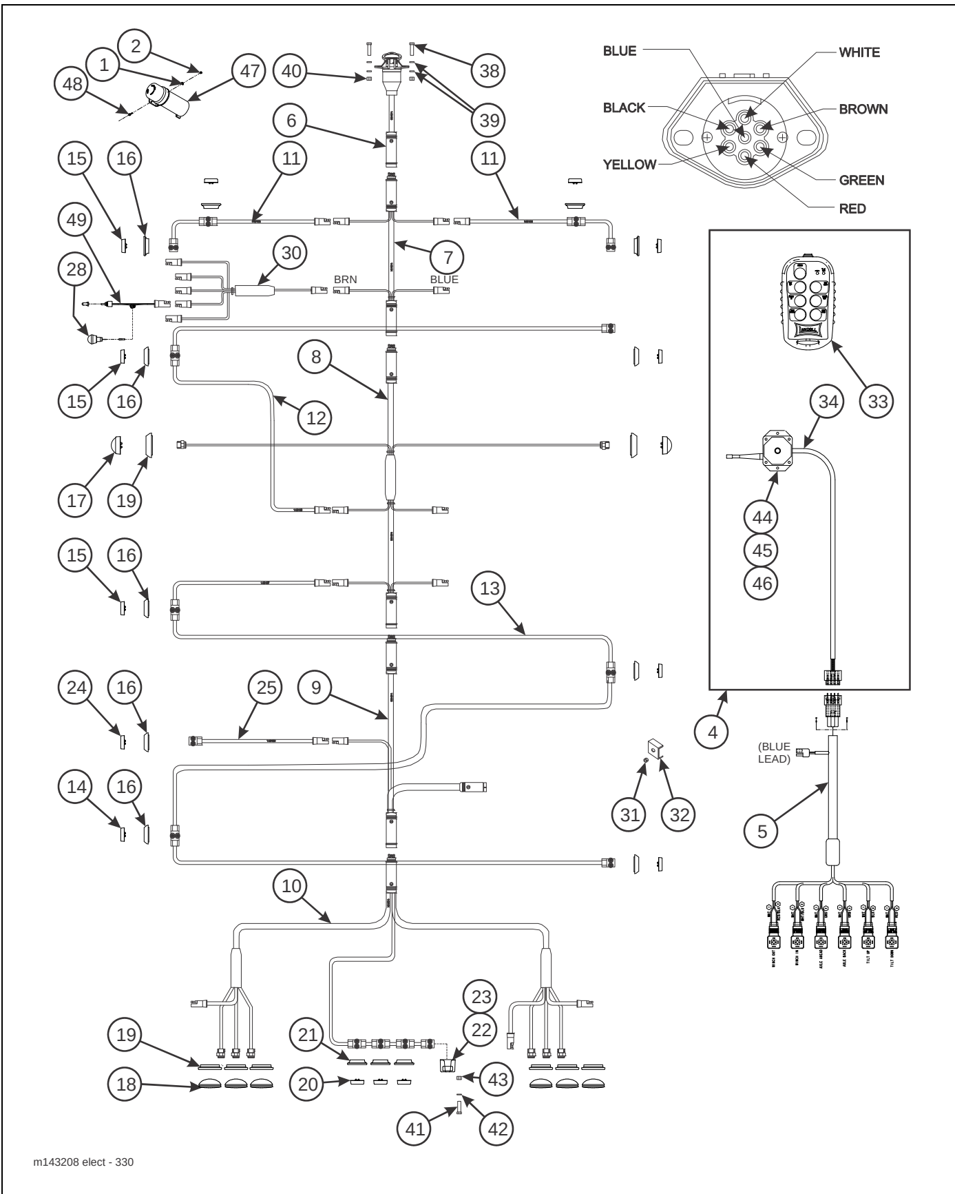
Figure 2-13: Electrical System
