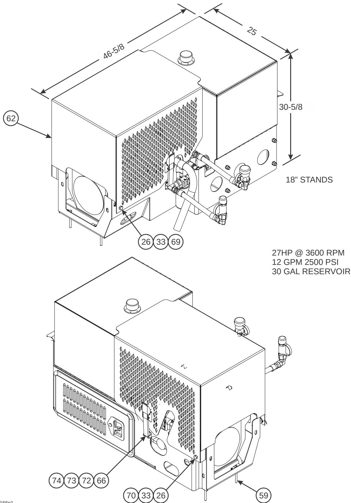
Figure 2-50: Engine Package, Front Mount (1 of 4)
