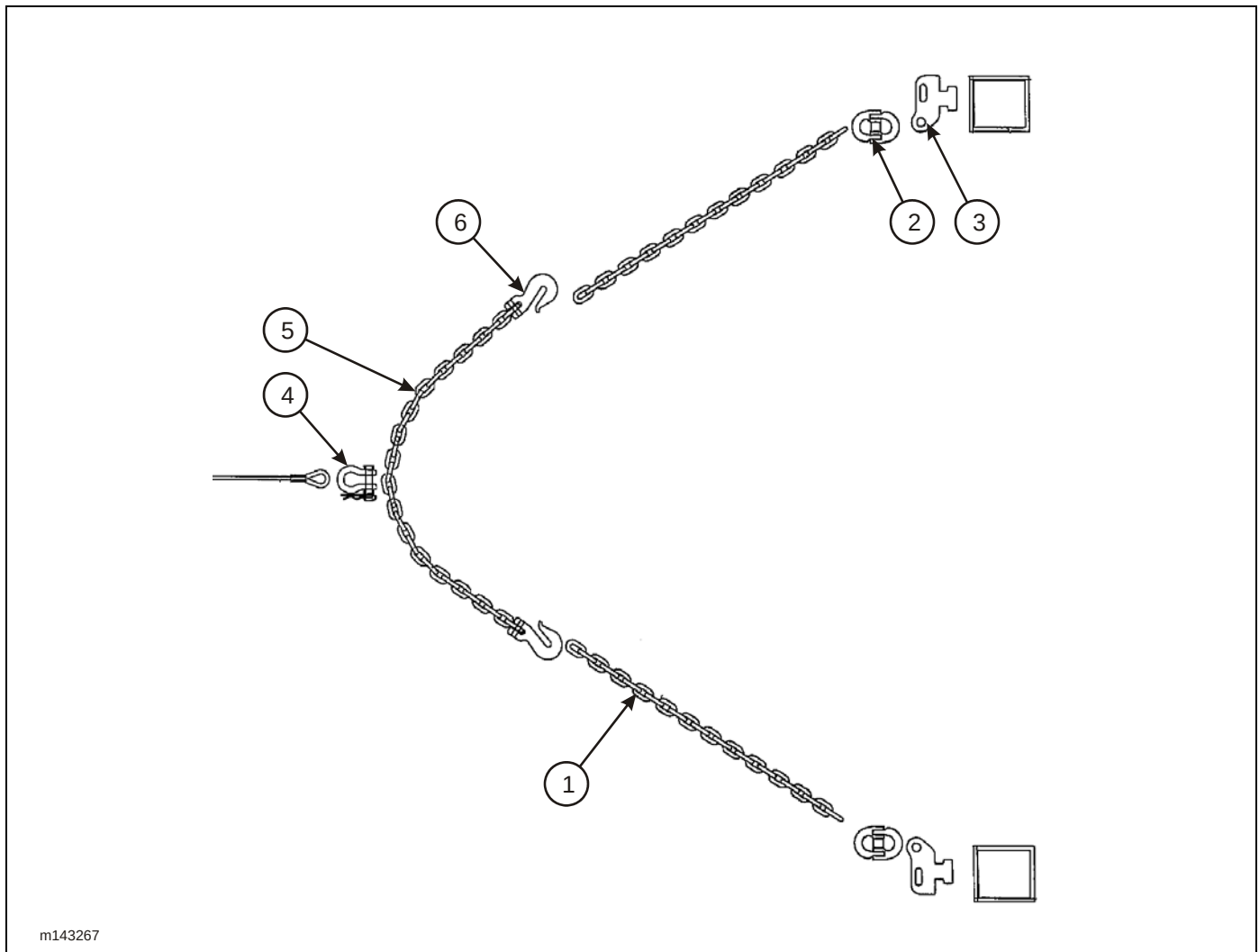
Figure 2-42: Container Chain and Bridle Assembly (Option)
