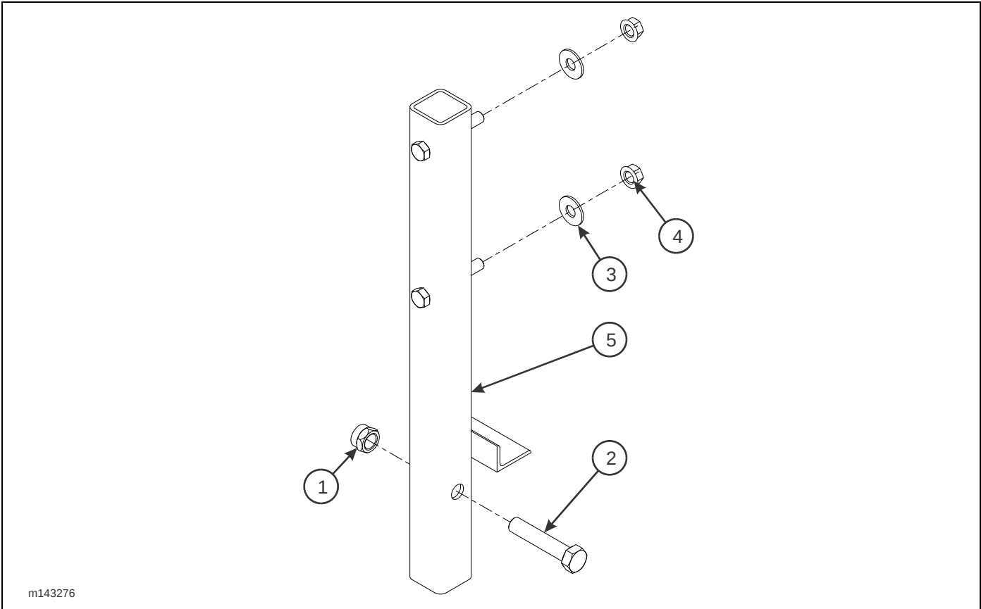
Figure 2-66: Spare Tire Mount Assembly (Option)
