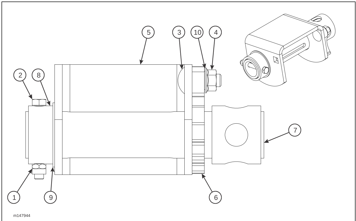
Figure 2-63: Winch Strap Ratchet Assembly (Option)
