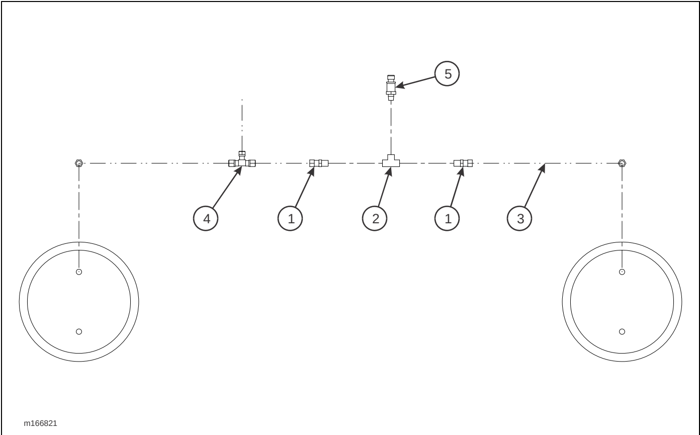
Figure 2-64: Digital Air System Scale Installation (Option)
