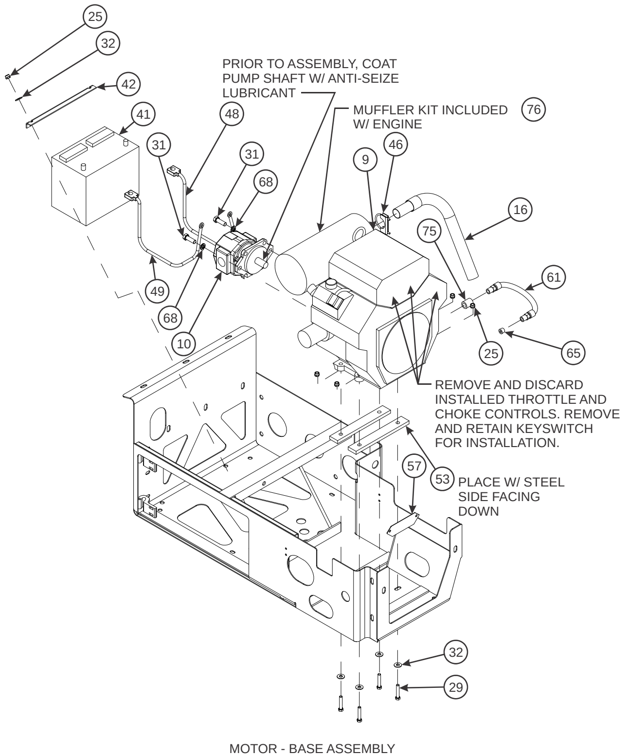
Figure 2-51: Engine Package, Front Mount (2 of 4)
