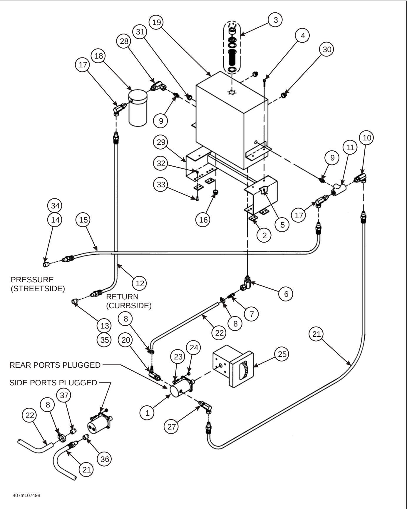
Figure 2-46: Hydraulic Wet Kit Assembly (Option)
