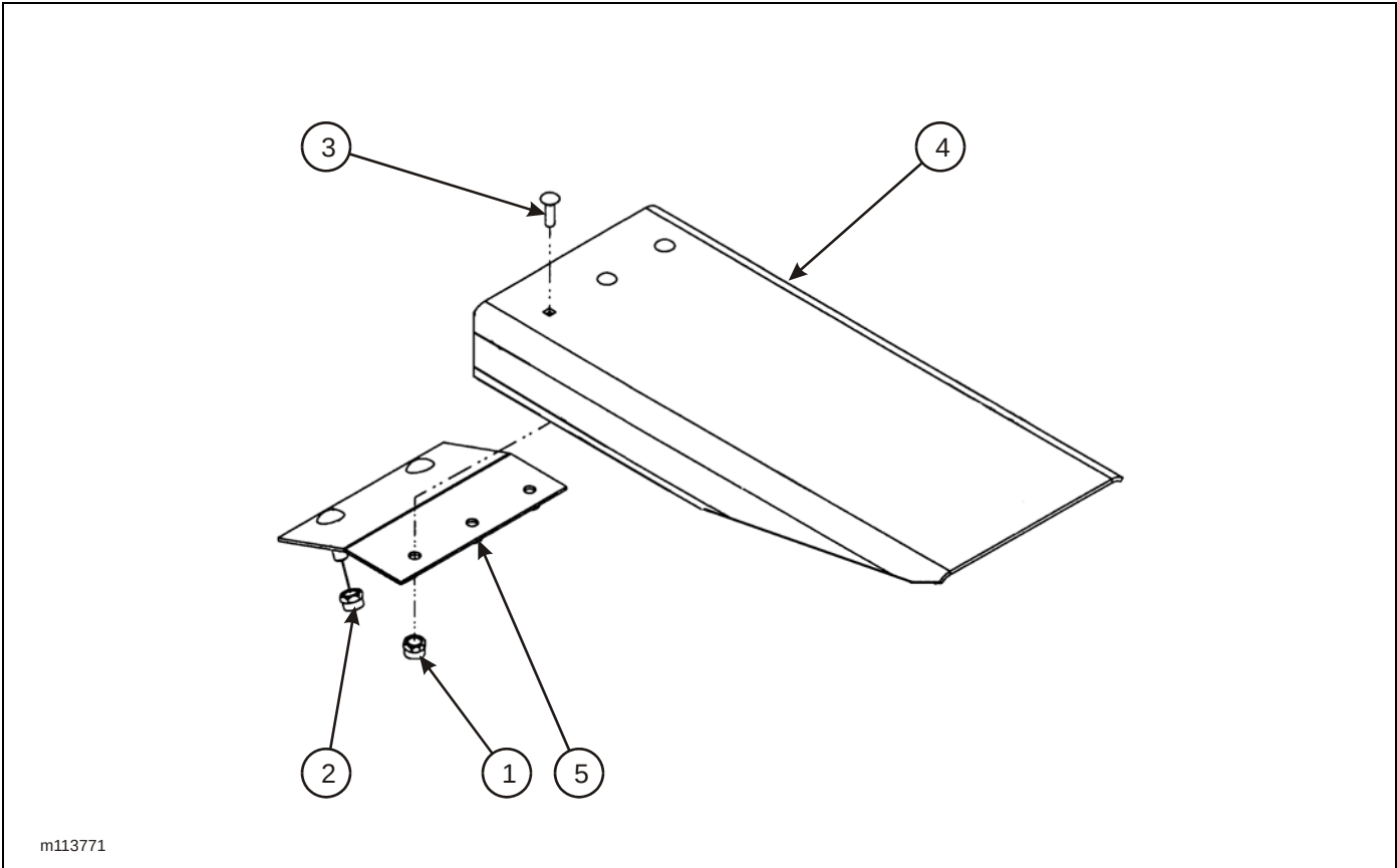
Figure 2-58: Aluminum Ramps (Option)
