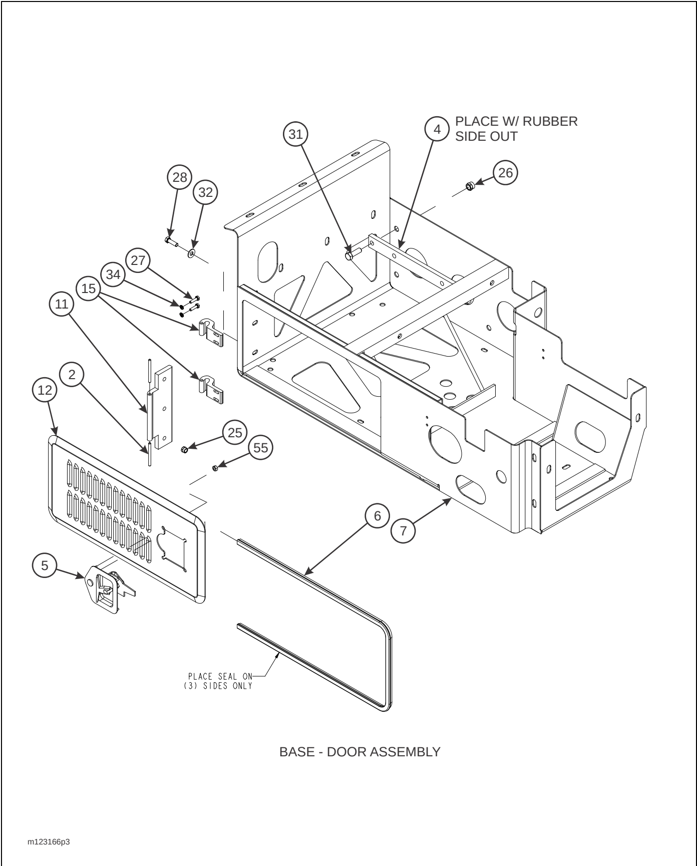
Figure 2-52: Engine Package, Front Mount (3 of 4)
