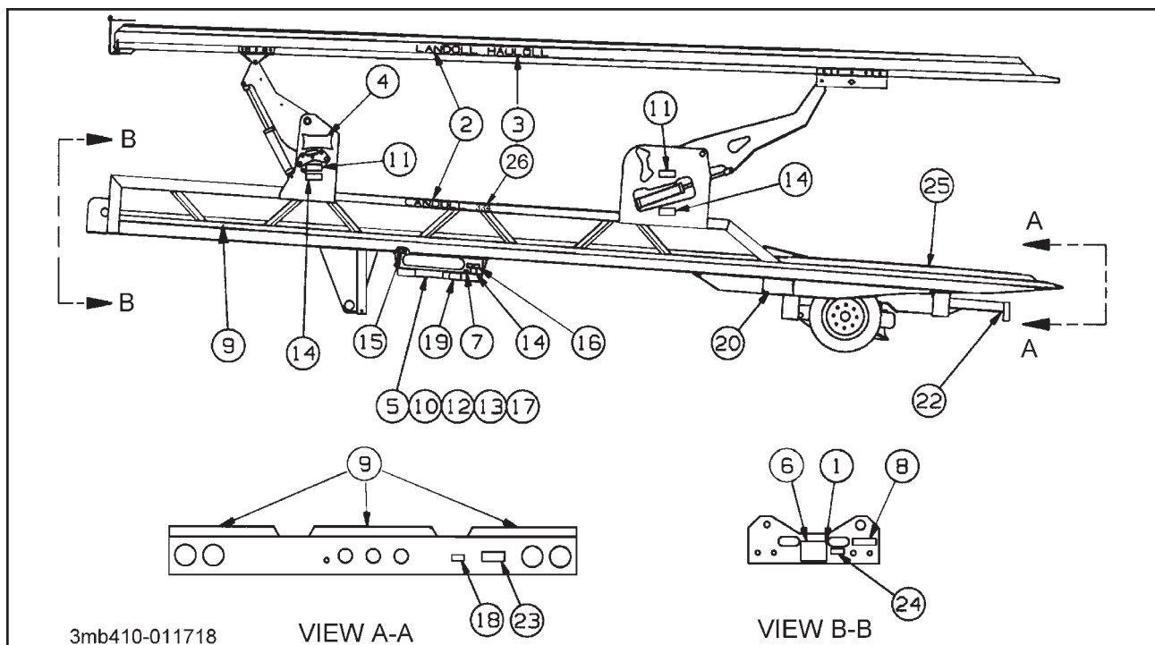
Figure 1-21 Decal Placement
