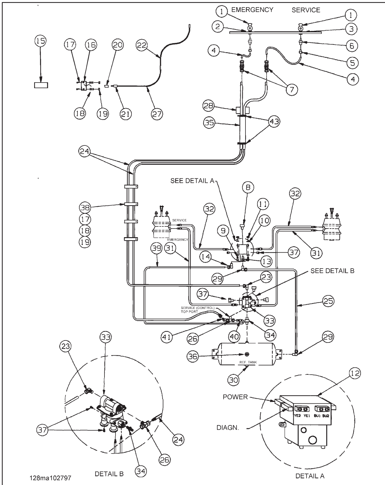
Figure 1-27 Air Brake System
