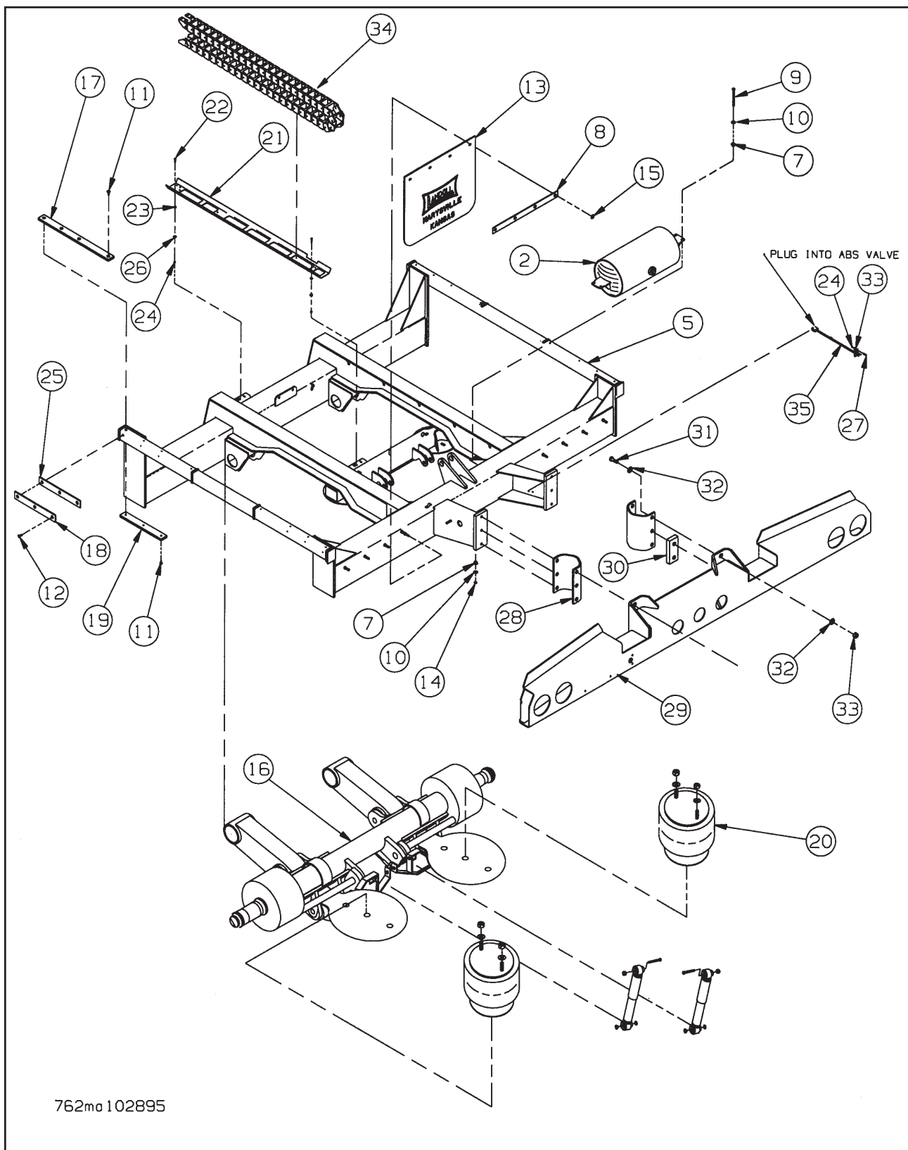
Figure 1-22 Undercarriage Assembly (1 of 2)
