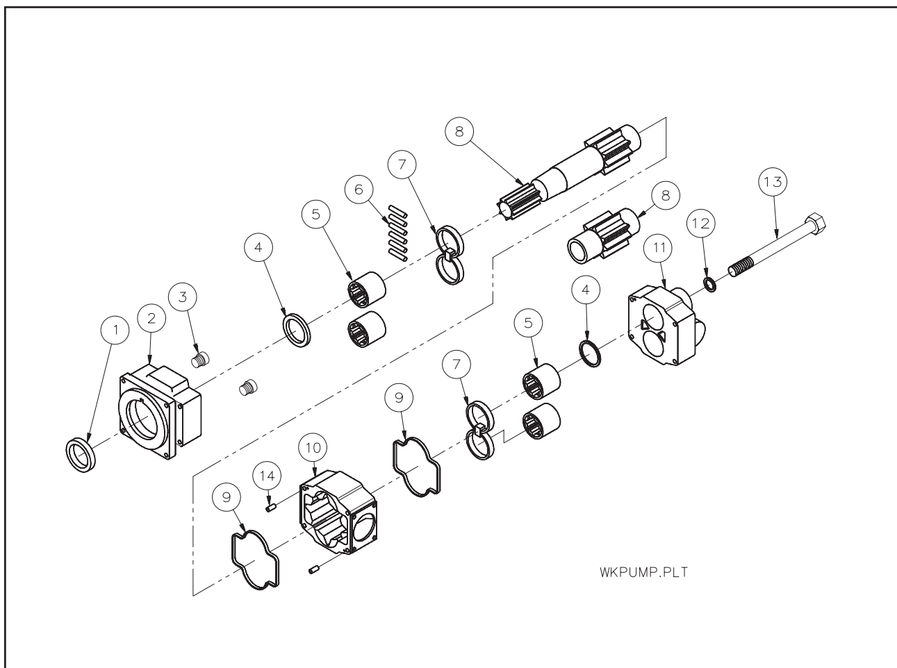
Figure 1-54 Wet Kit Pump
