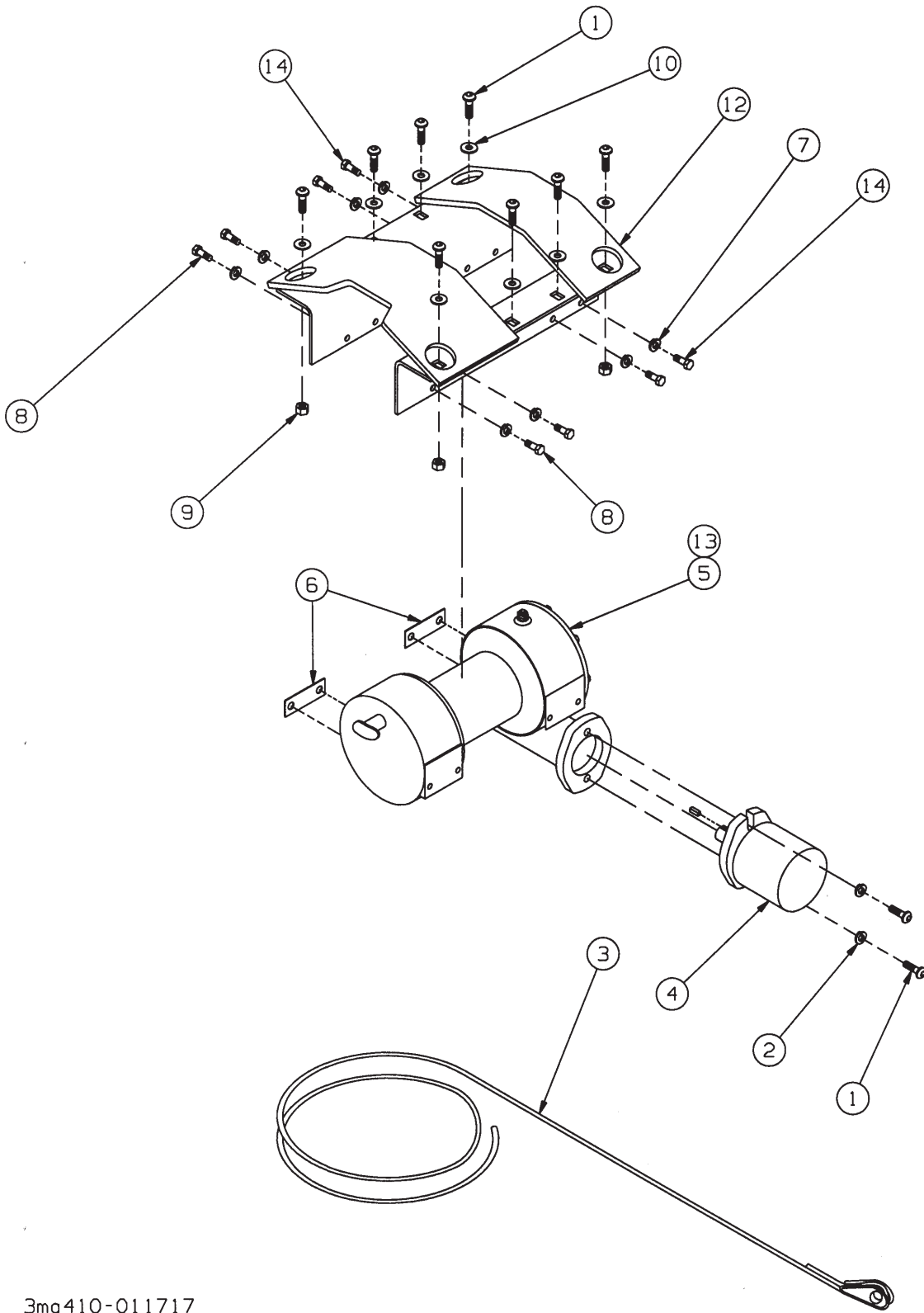
Figure 1-31 Winch Installation
