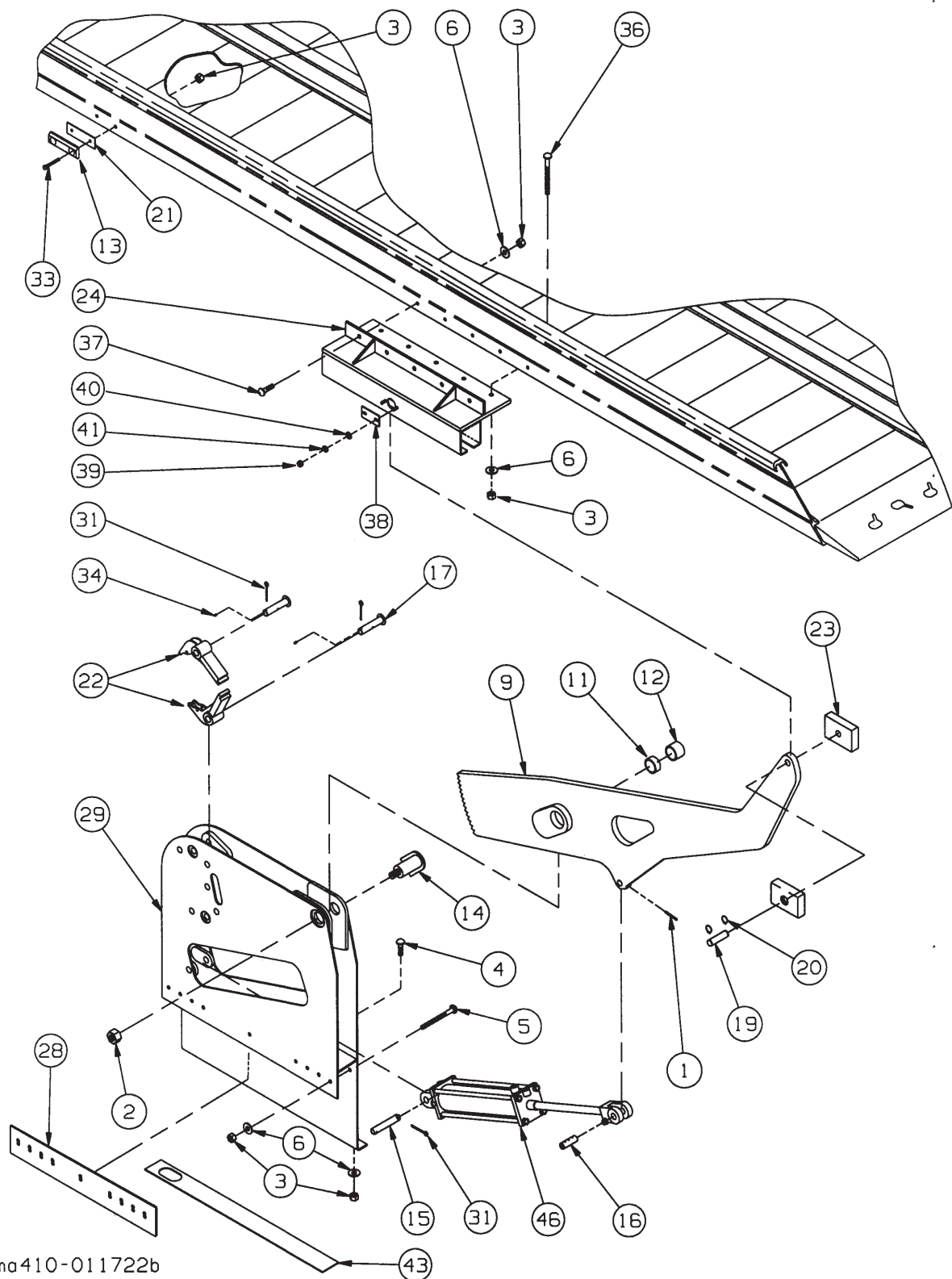
Figure 1-4 Rear Upper Deck Support
