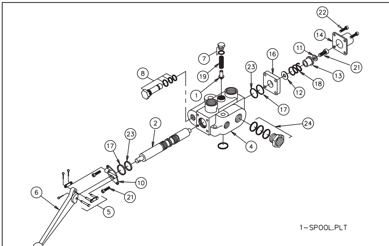
Figure 1-51 Hydraulic Single Spool Valve
