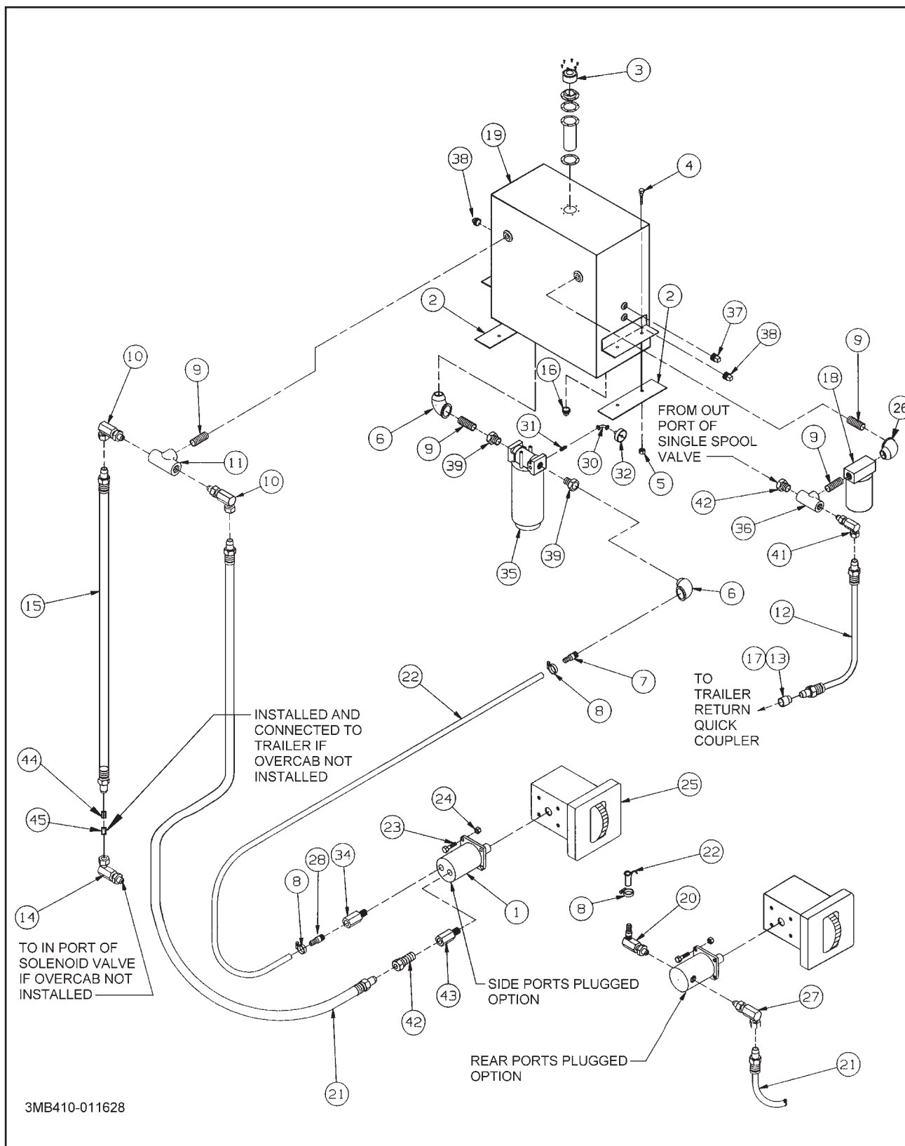
Figure 1-53 Wet Kit Assembly
