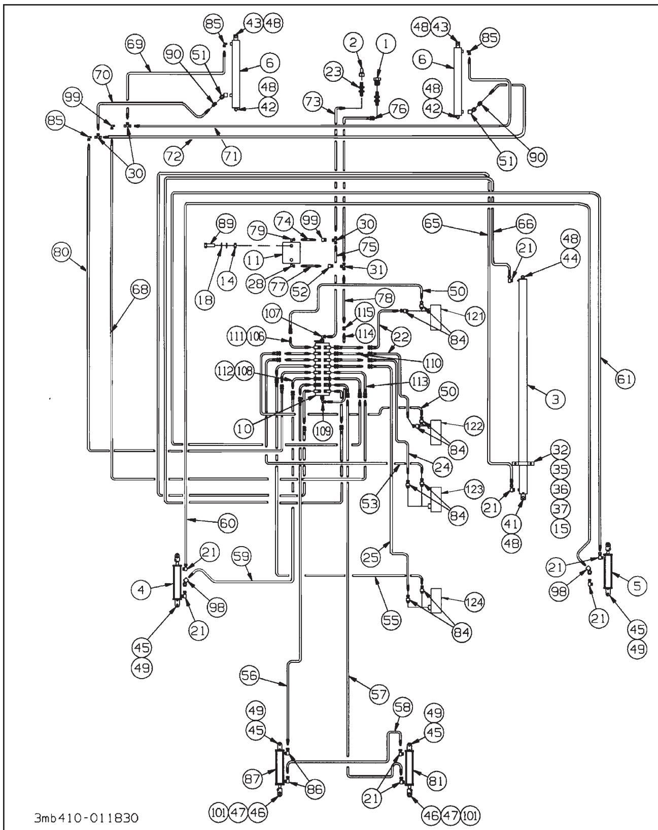
Figure 1-9 Hydraulic System
