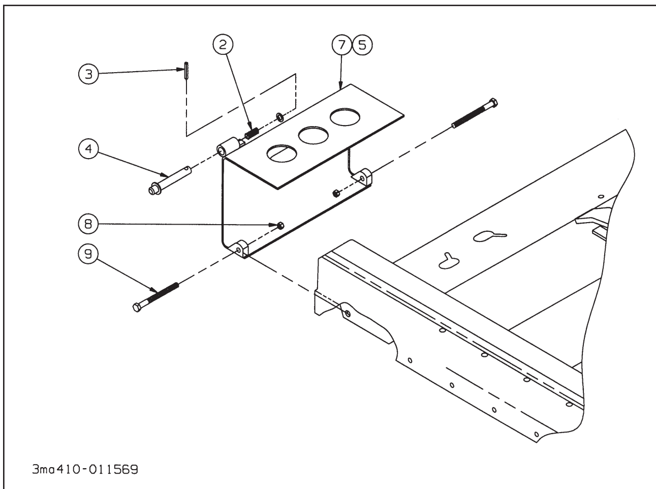
Figure 1-2 Wheel Stops
