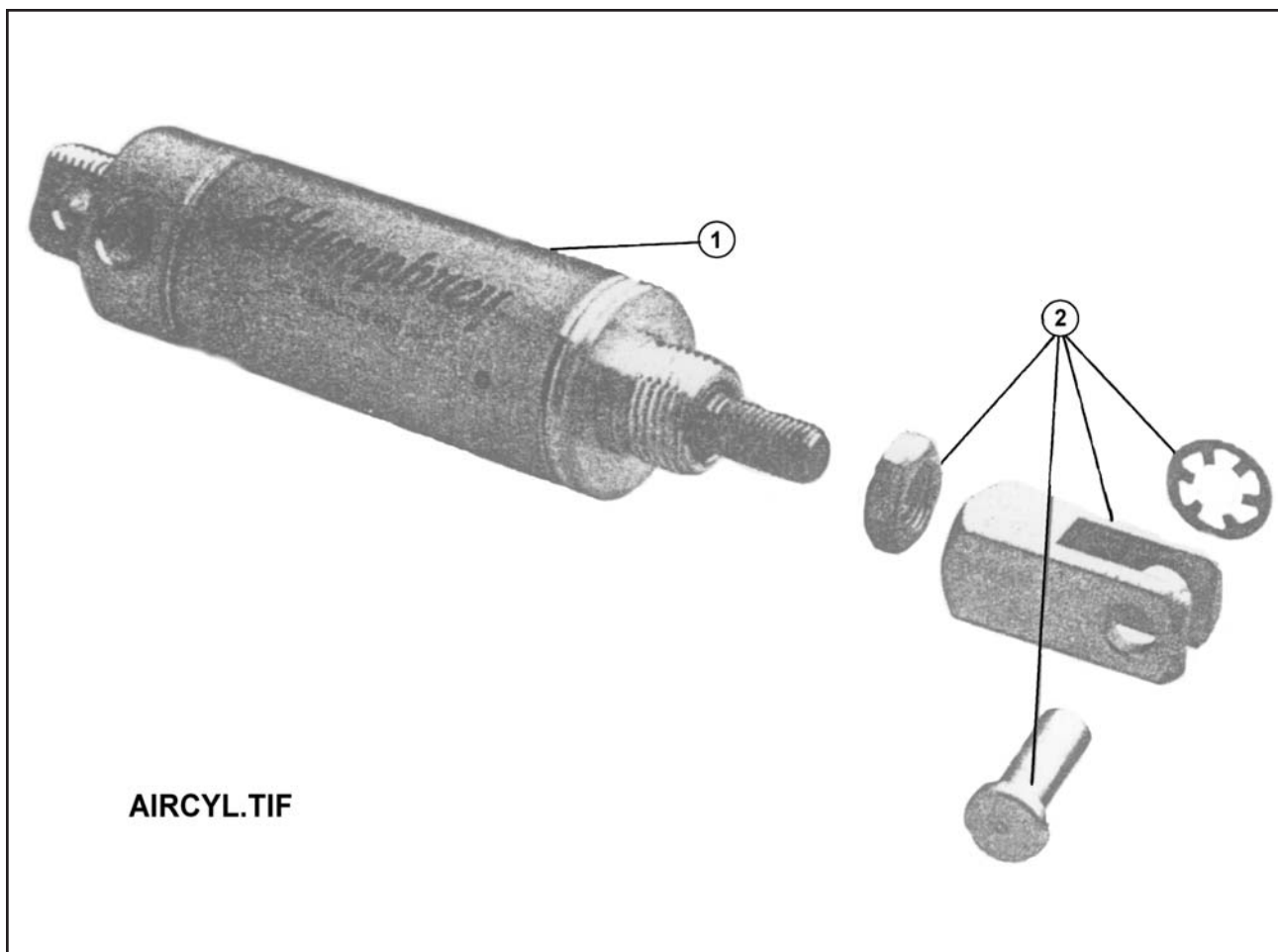
Figure 1-57 Cylinder, Air 1-3/4 Bore
