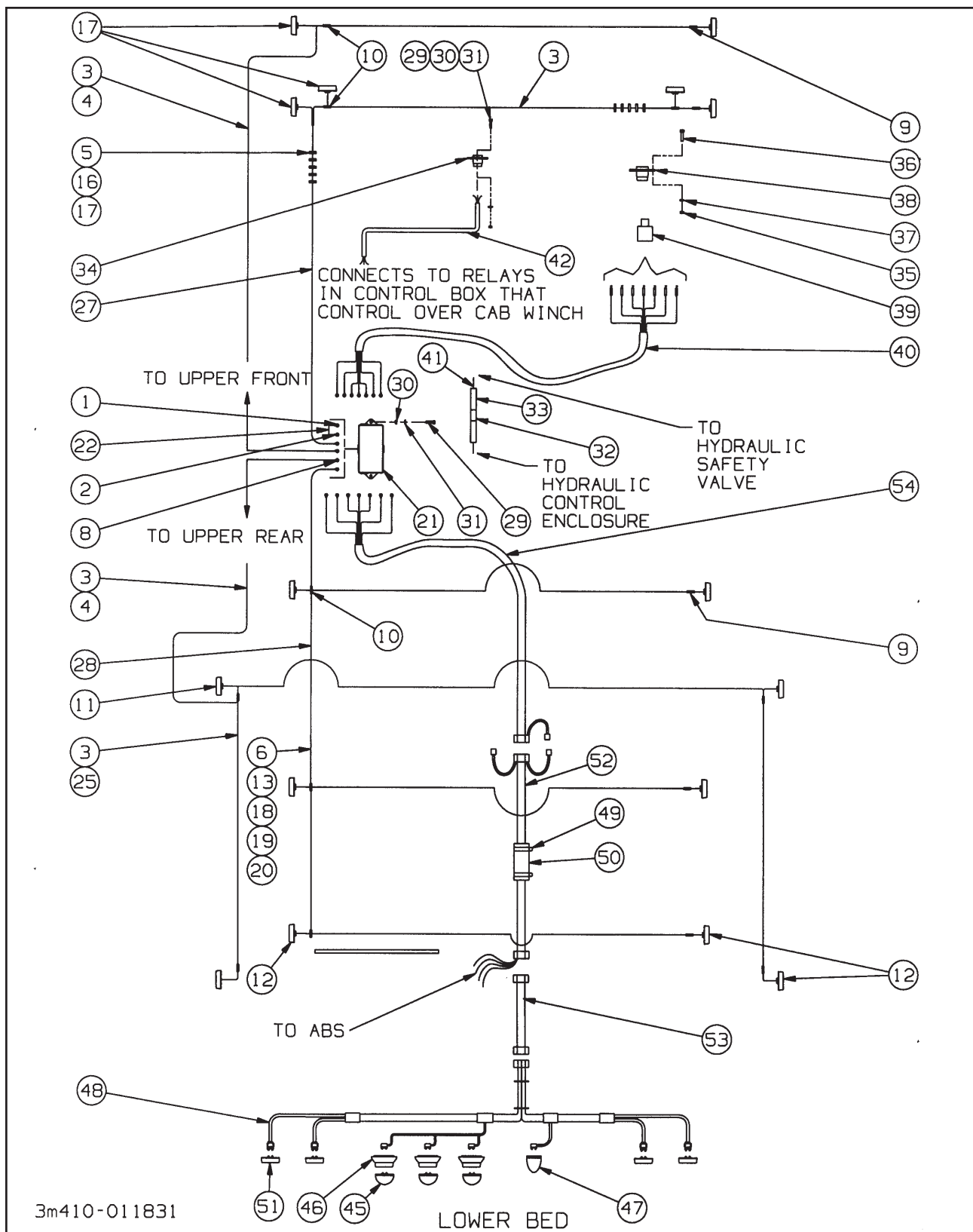
Figure 1-18 Electrical System
