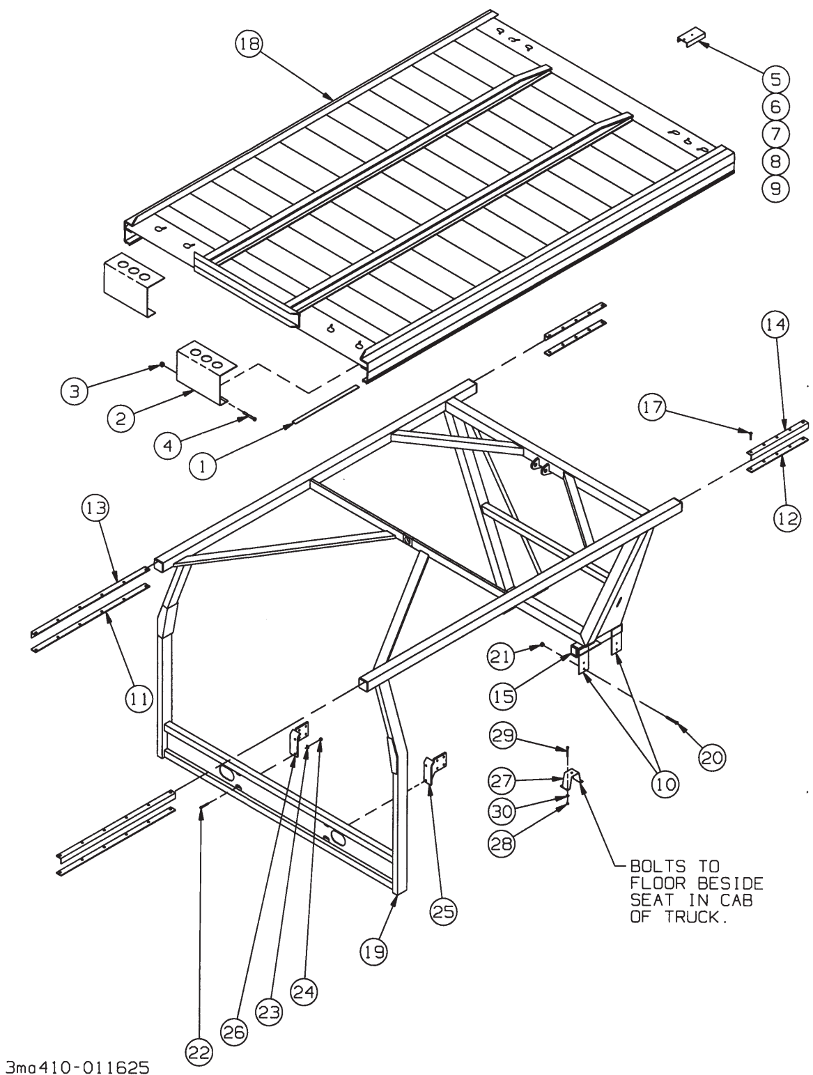
Figure 1-45 "Over-the-cab" Frame and Bed
