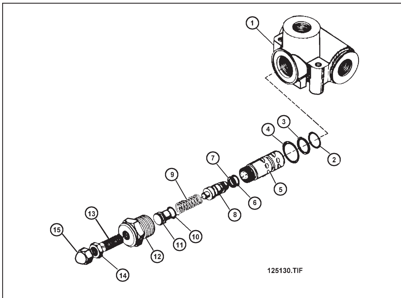
Figure 1-55 Pressure Relief Valve
