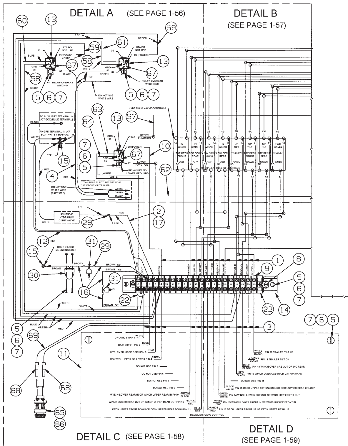
Figure 1-34 Electrical System, Remote Control
