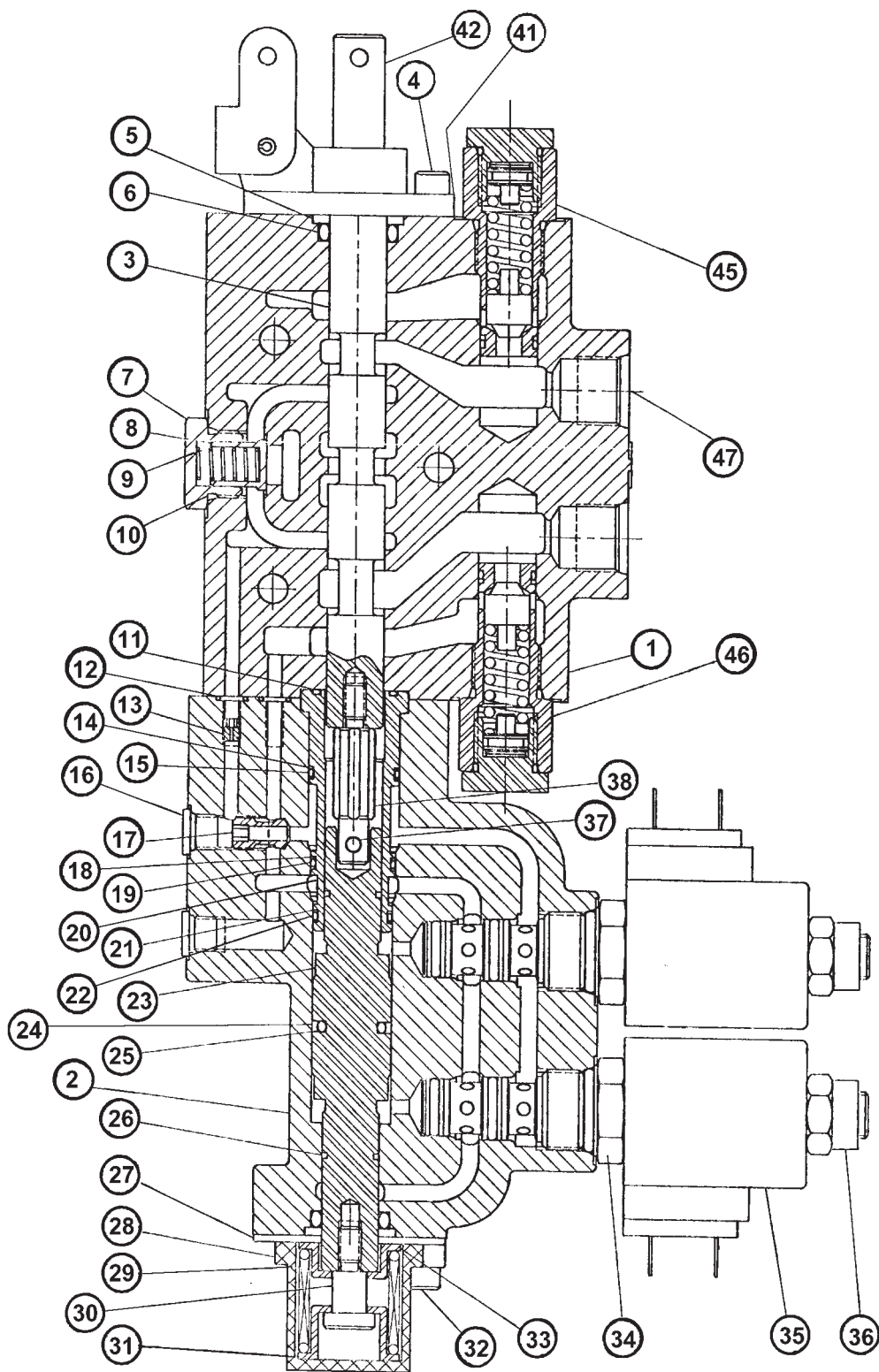
Figure 1-16 Eight Spool Valve, Work Sections
