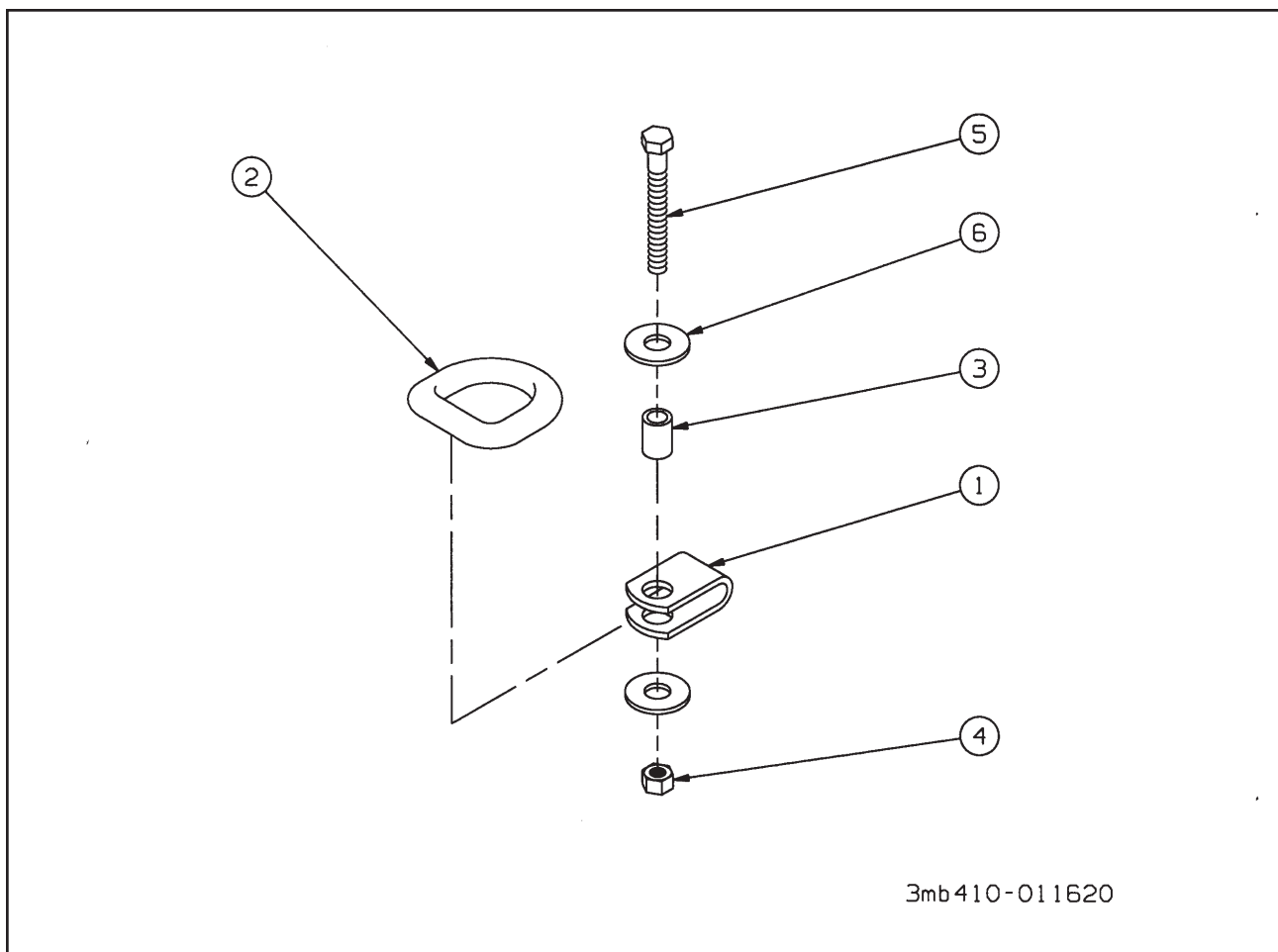
Figure 1-43 D-Ring Kit
