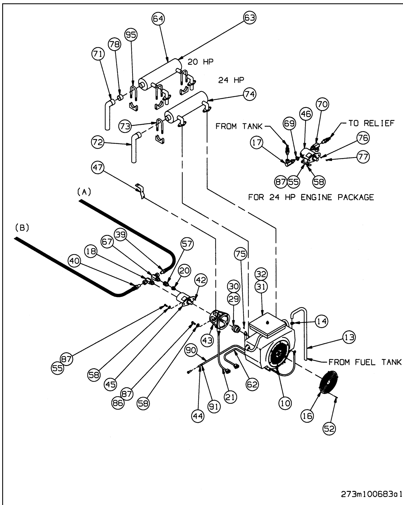
Figure 1-43 Auxiliary Engine Package Upperdeck (2 of 2)
