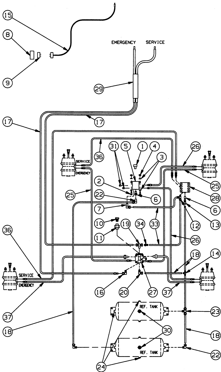
Figure 1-24 Air Brake System, Tandem Axle
