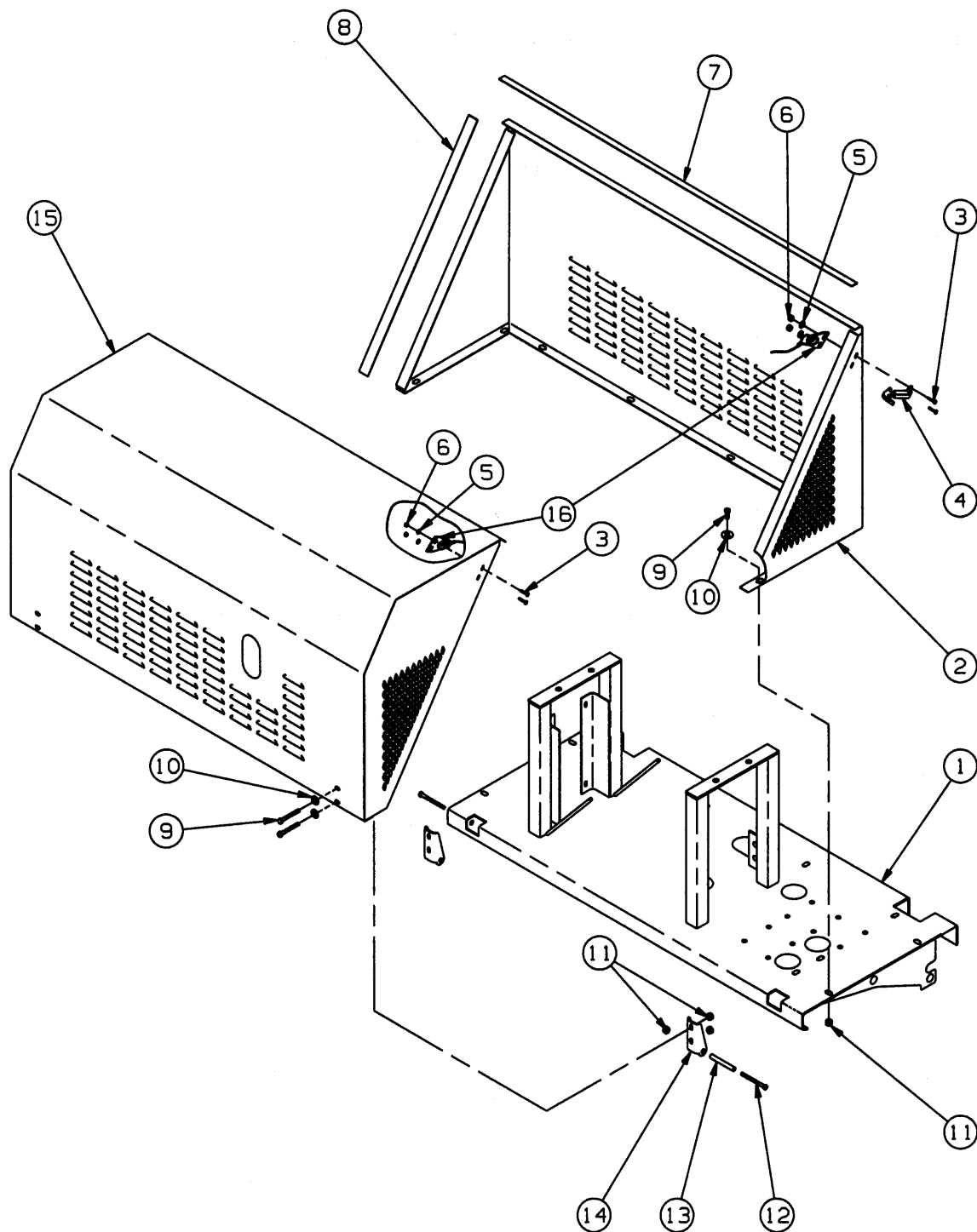
Figure 1-46 Engine Cover Assembly
