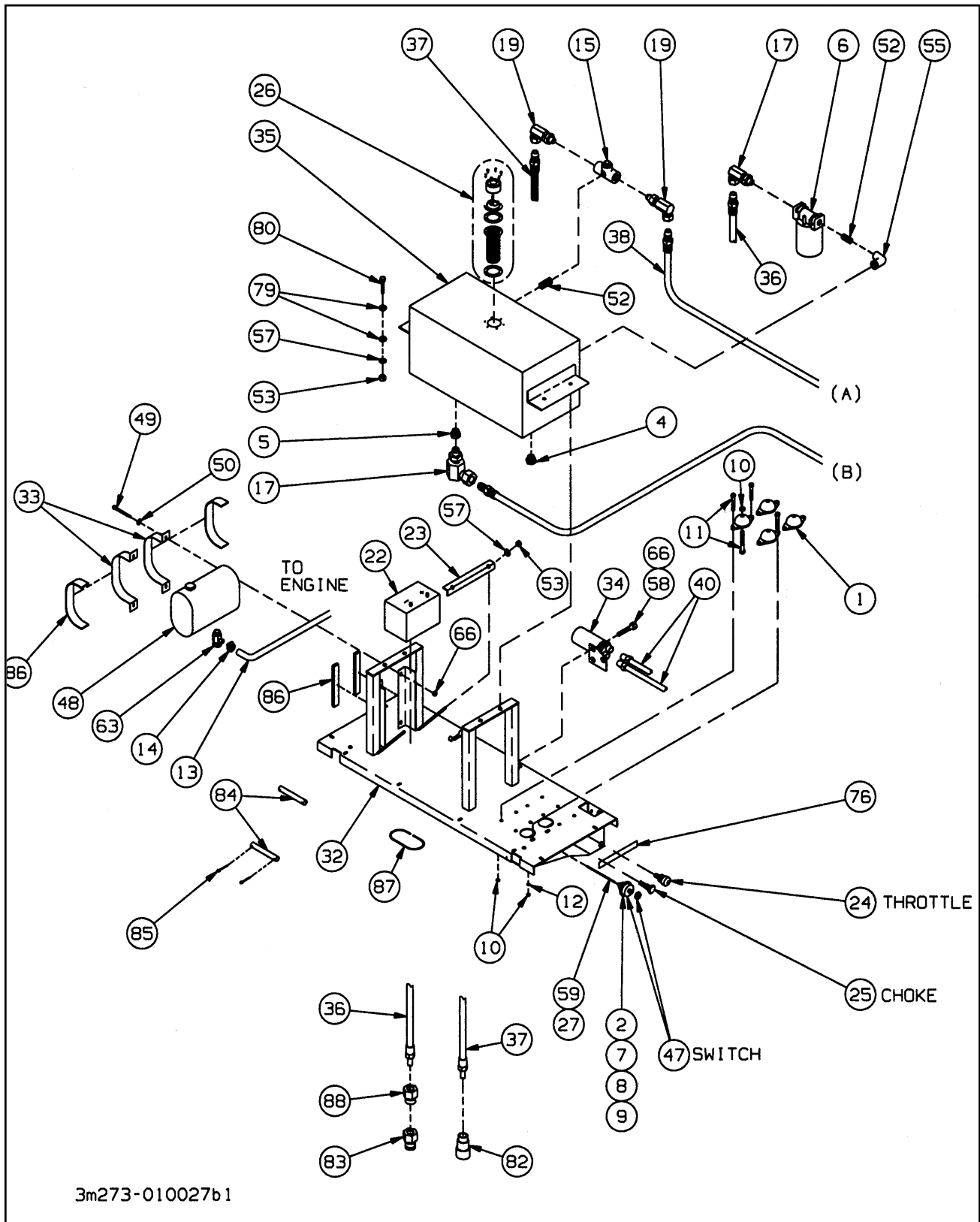
Figure 1-44 Engine Package Front Mount (1 of 2)
