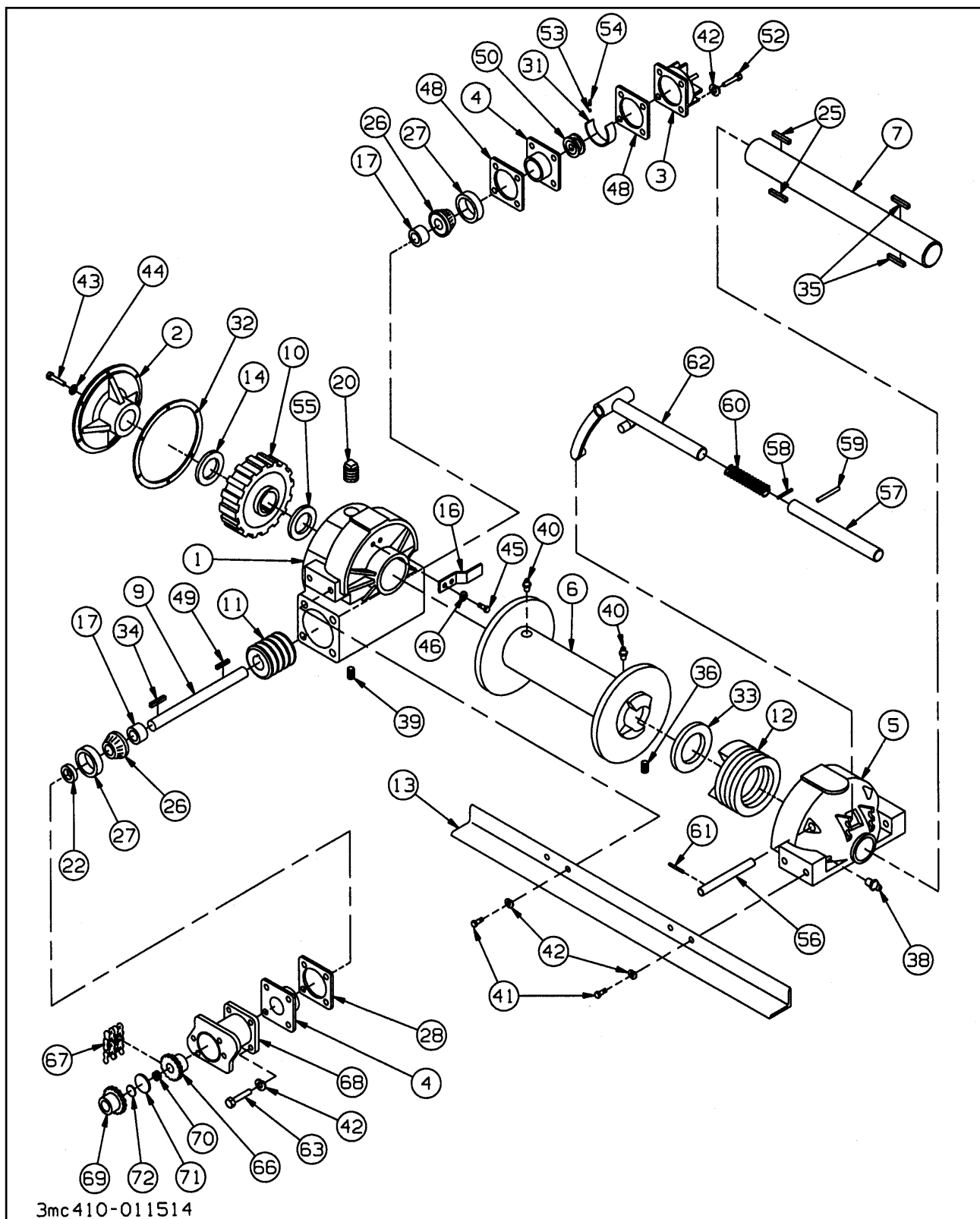
Figure 1-31 12,000# Winch Assembly
