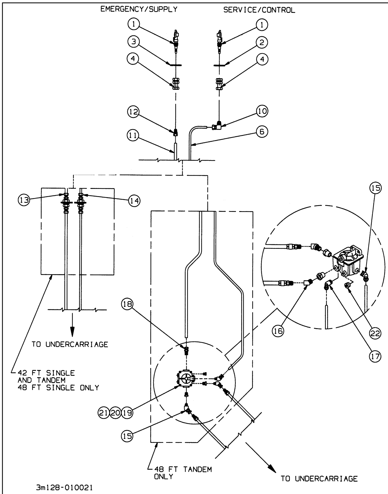
Figure 1-29 Air System
