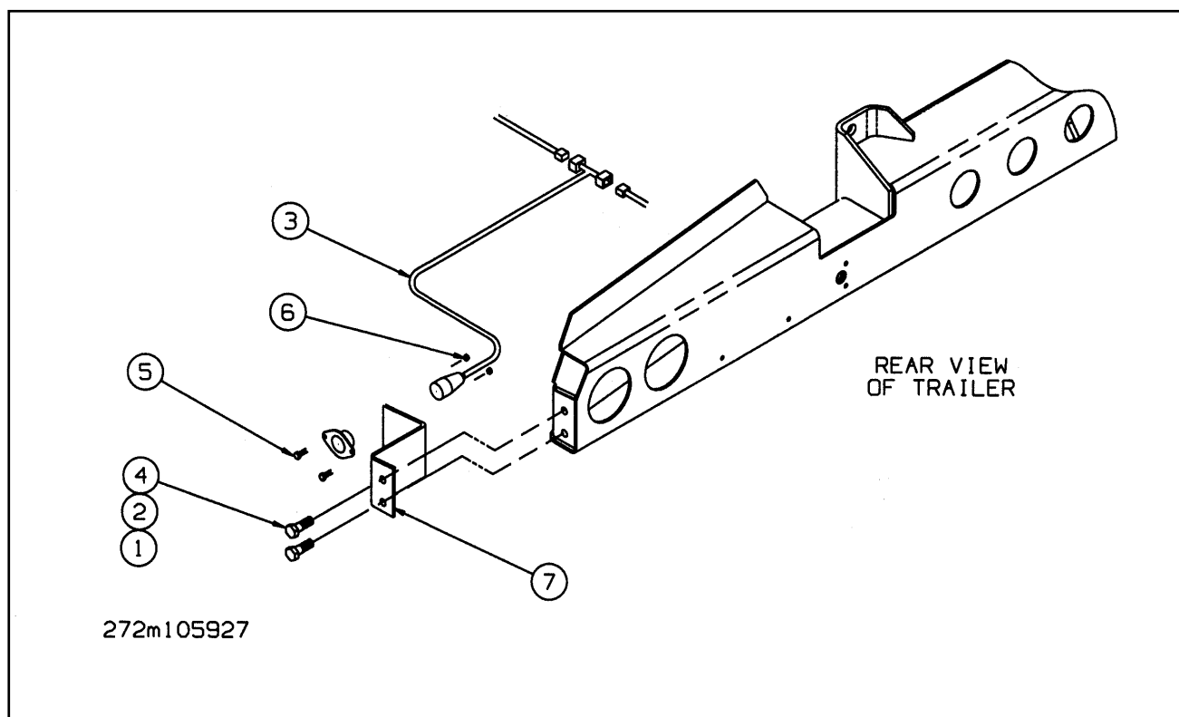
Figure 1-50 Electrical Installation, 7-Way Recp Bumper
