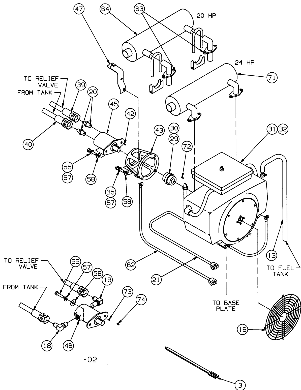
Figure 1-44 Auxiliary Engine Package (1 of 2)
