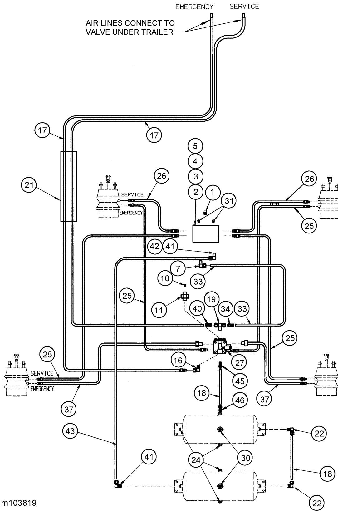
Figure 1-27 Air Brake System, Tandem Axle
