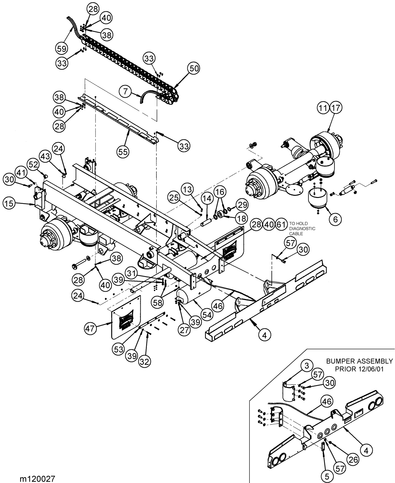
Figure 1-20 Undercarriage Assembly - Air Ride (Tandem)
