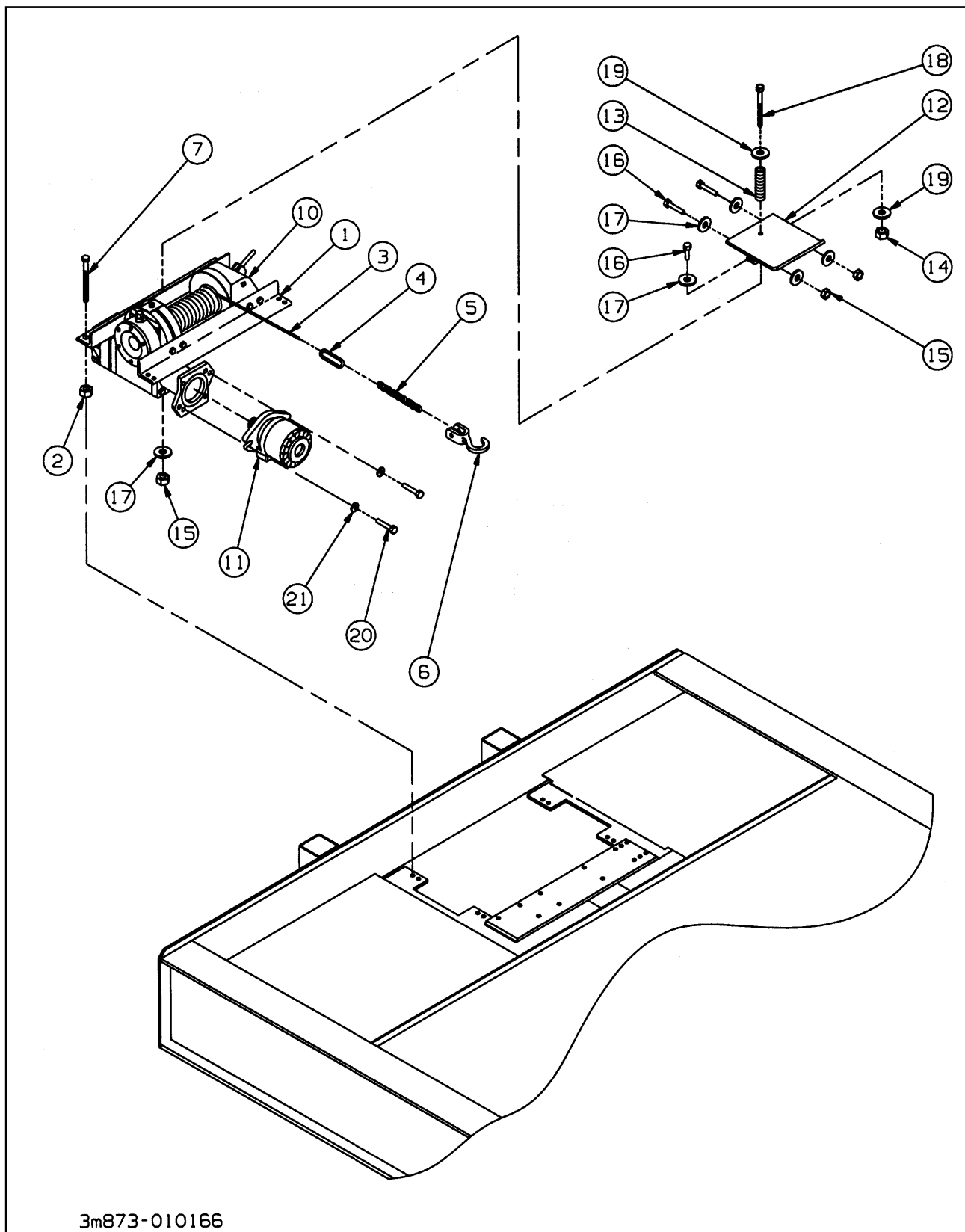
Figure 1-31 Winch Installation
