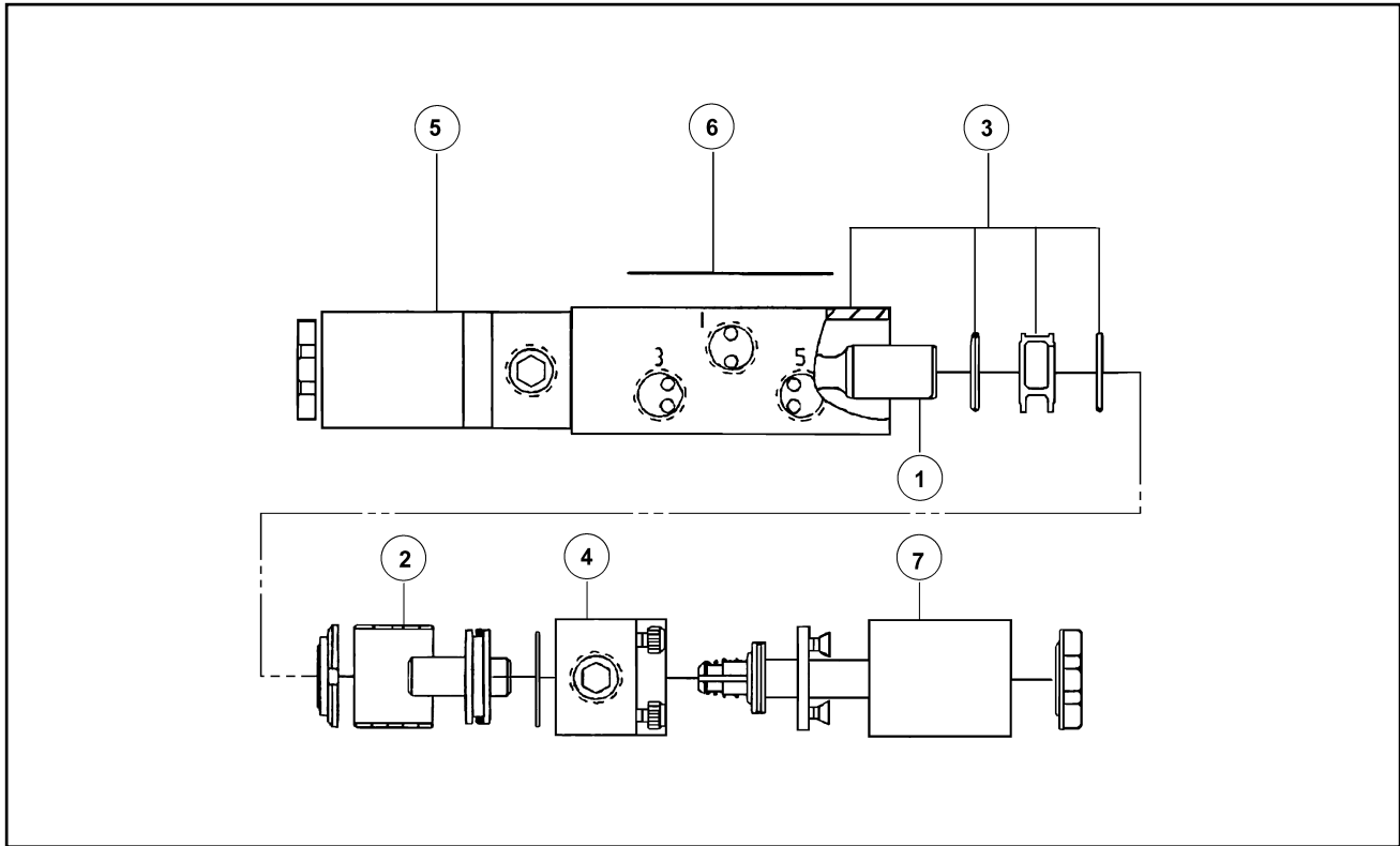
Figure 1-9 Pneumatic Valve
