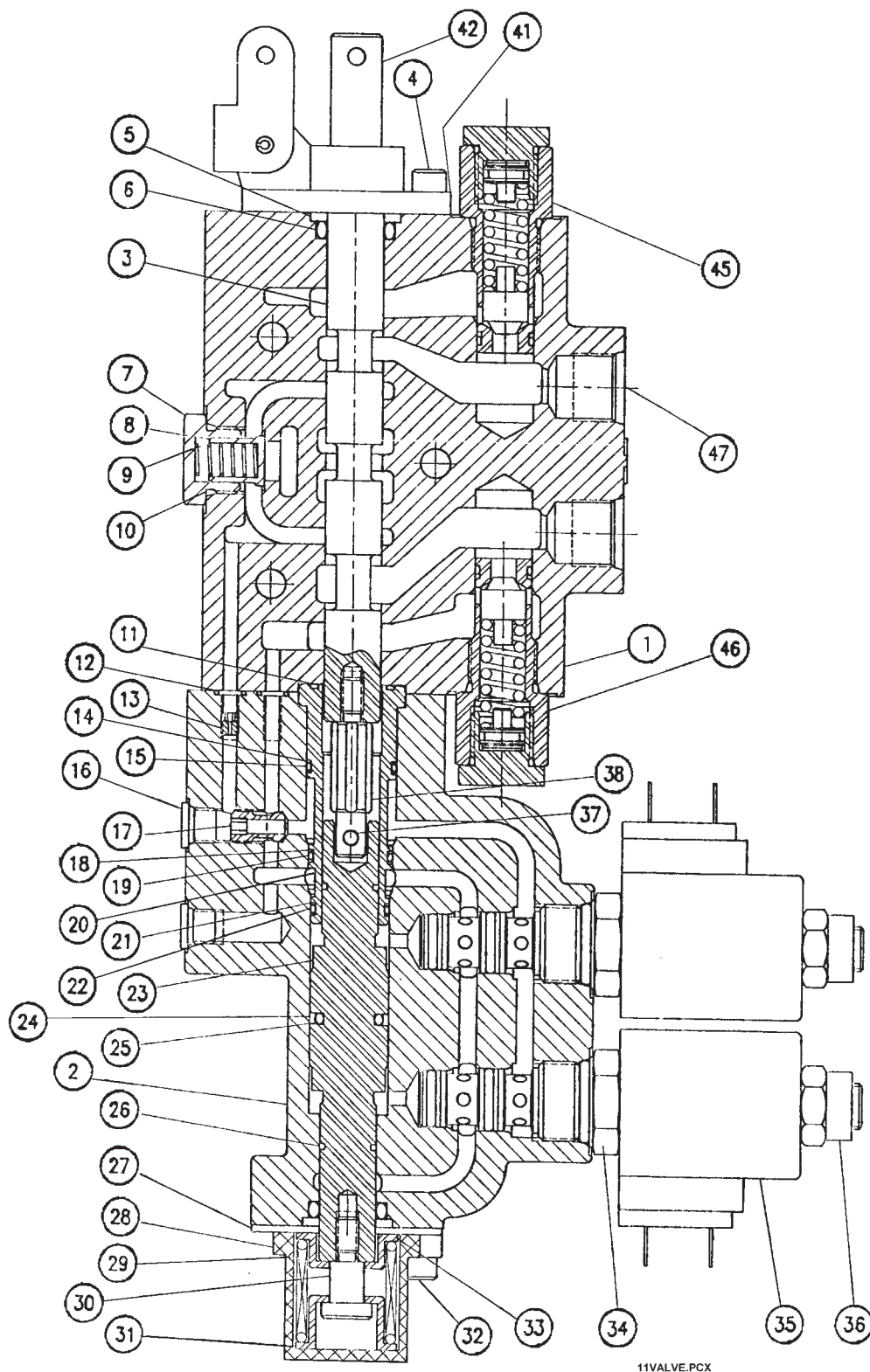
Figure 1-22 Spool Valve, Work Sections
