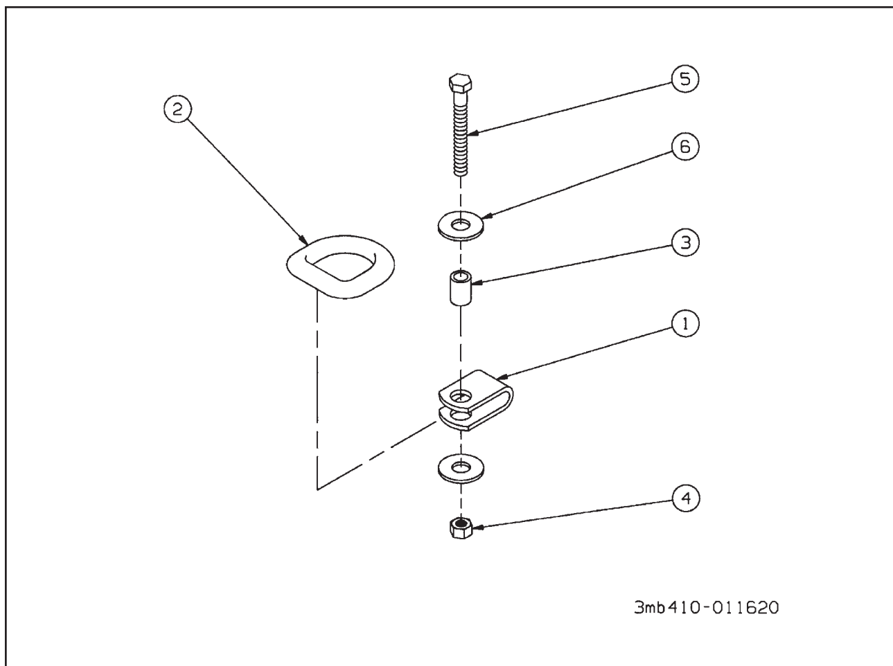
Figure 1-11 D-Ring Kit
