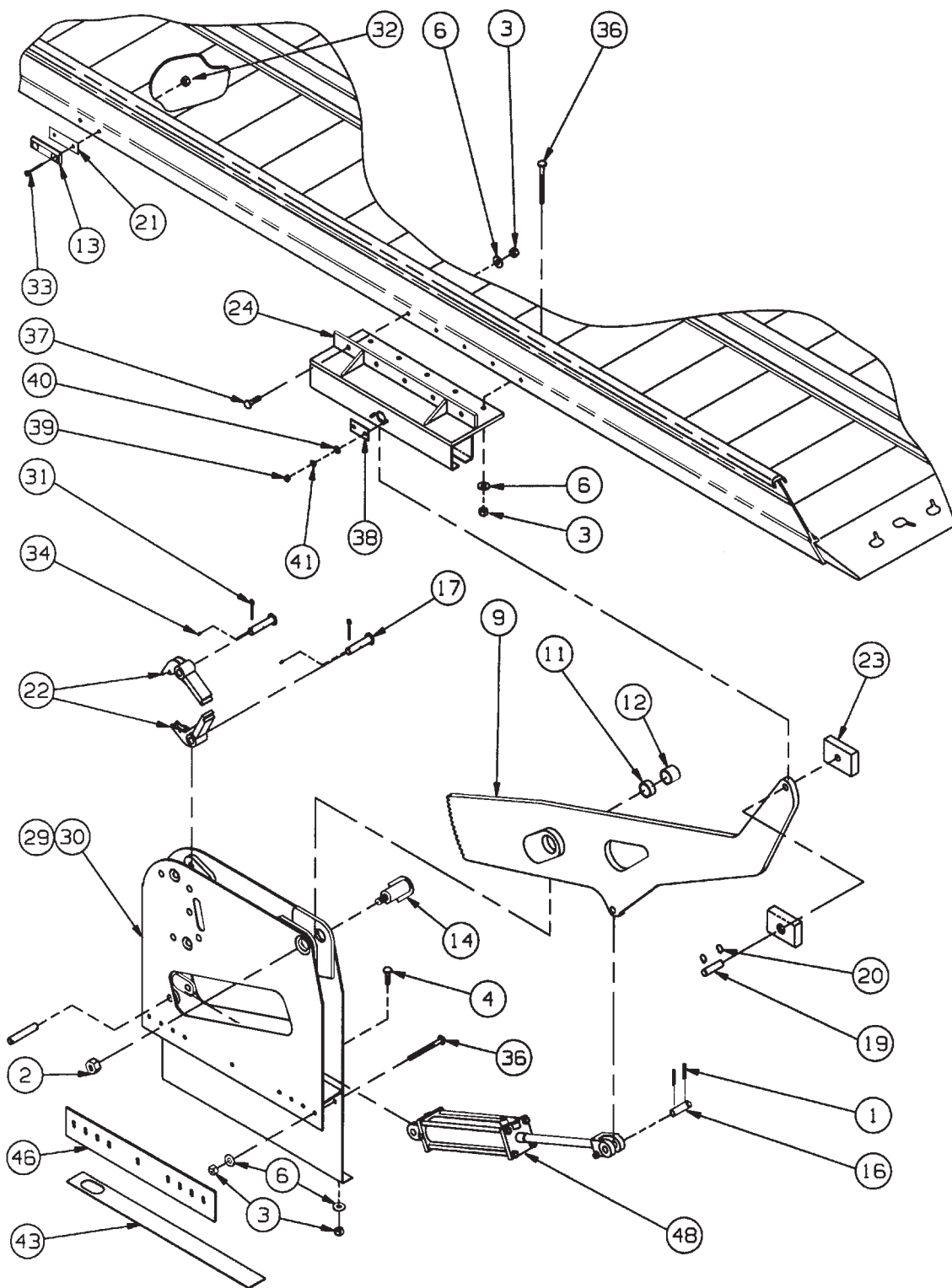
Figure 1-6 Rear Upper Deck Support
