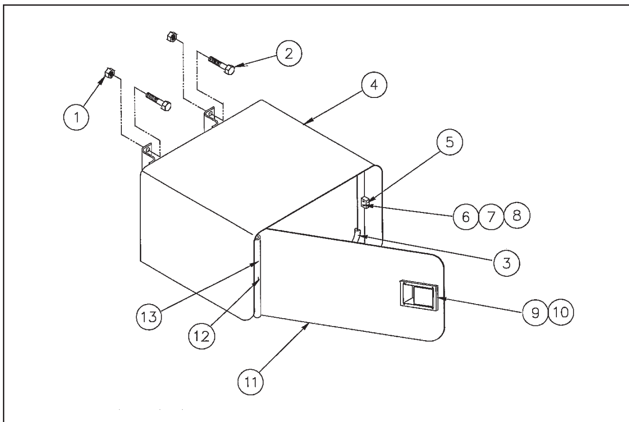
Figure 1-52 Tool Box
