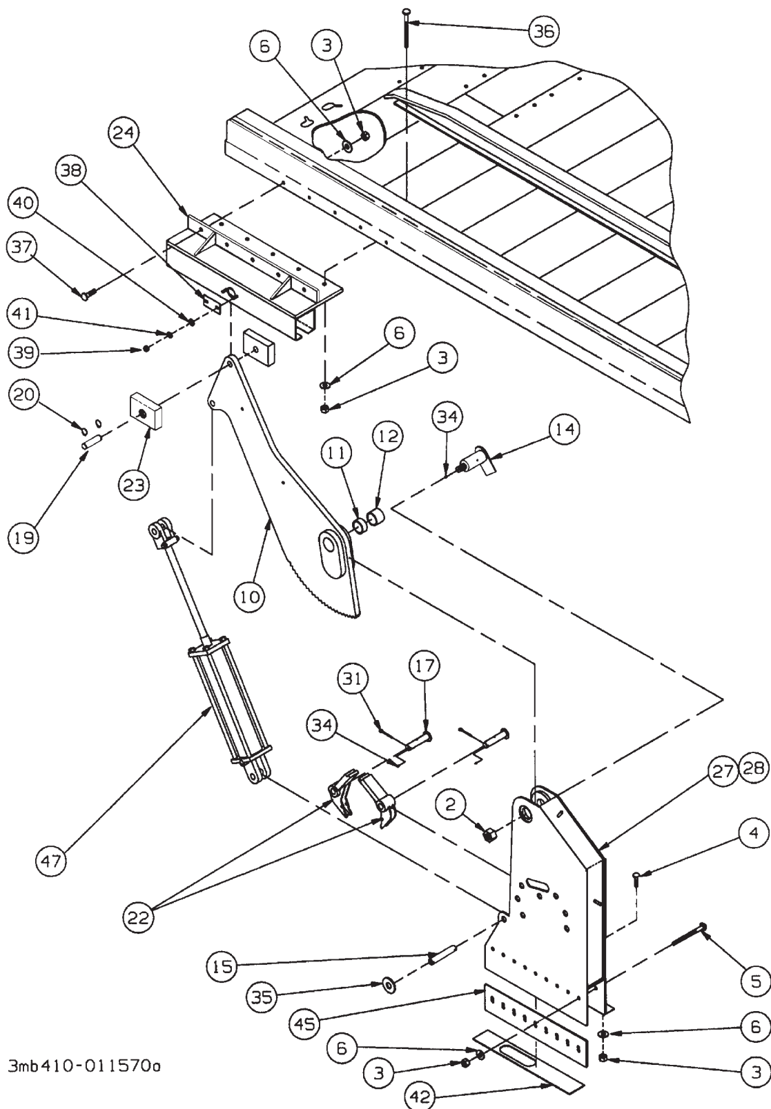
Figure 1-4 Front Upper Deck Support
