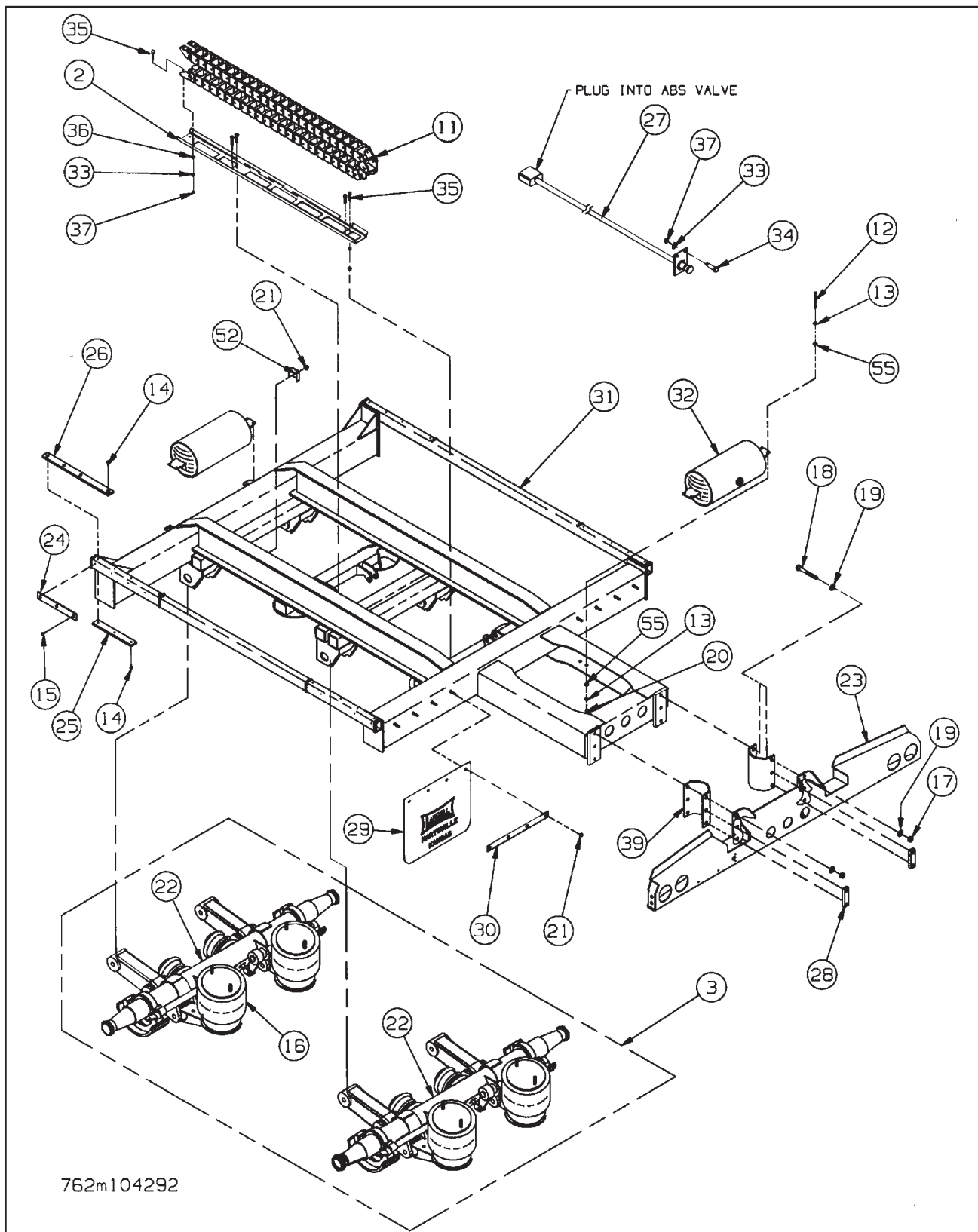
Figure 1-29 Undercarriage Assembly (1 of 2)
