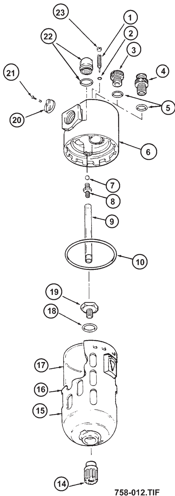
Figure 1-9 Air System Lubricator
