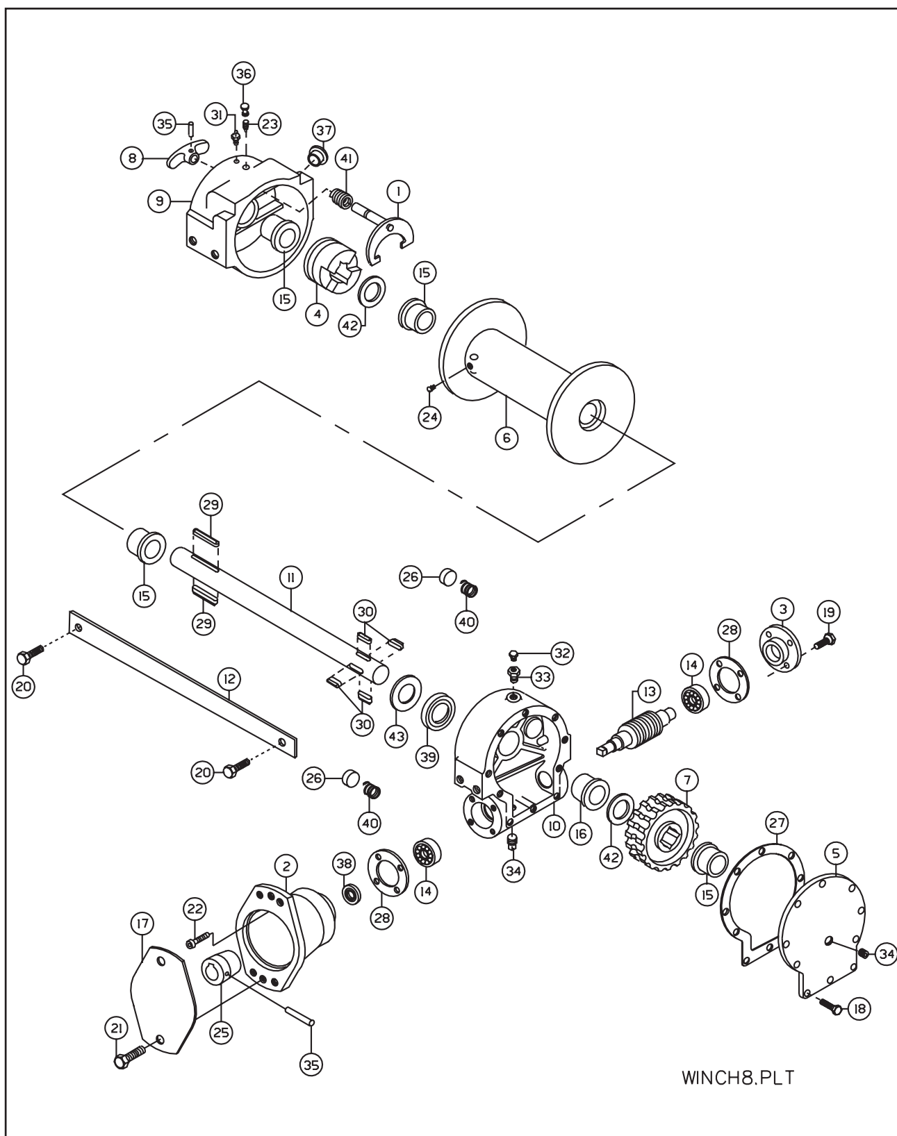
Figure 1-40 8,000# Winch Assembly
