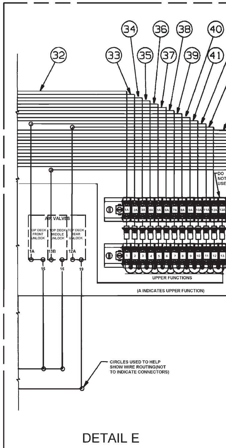
Figure 1-48 Electrical System, Remote Control Detail E
