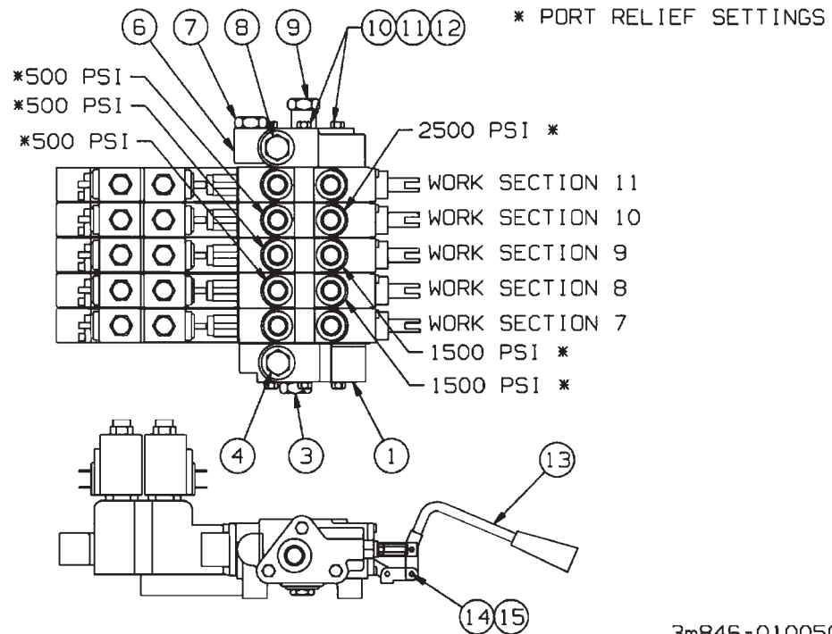
Figure 1-21 Five Spool Valve
