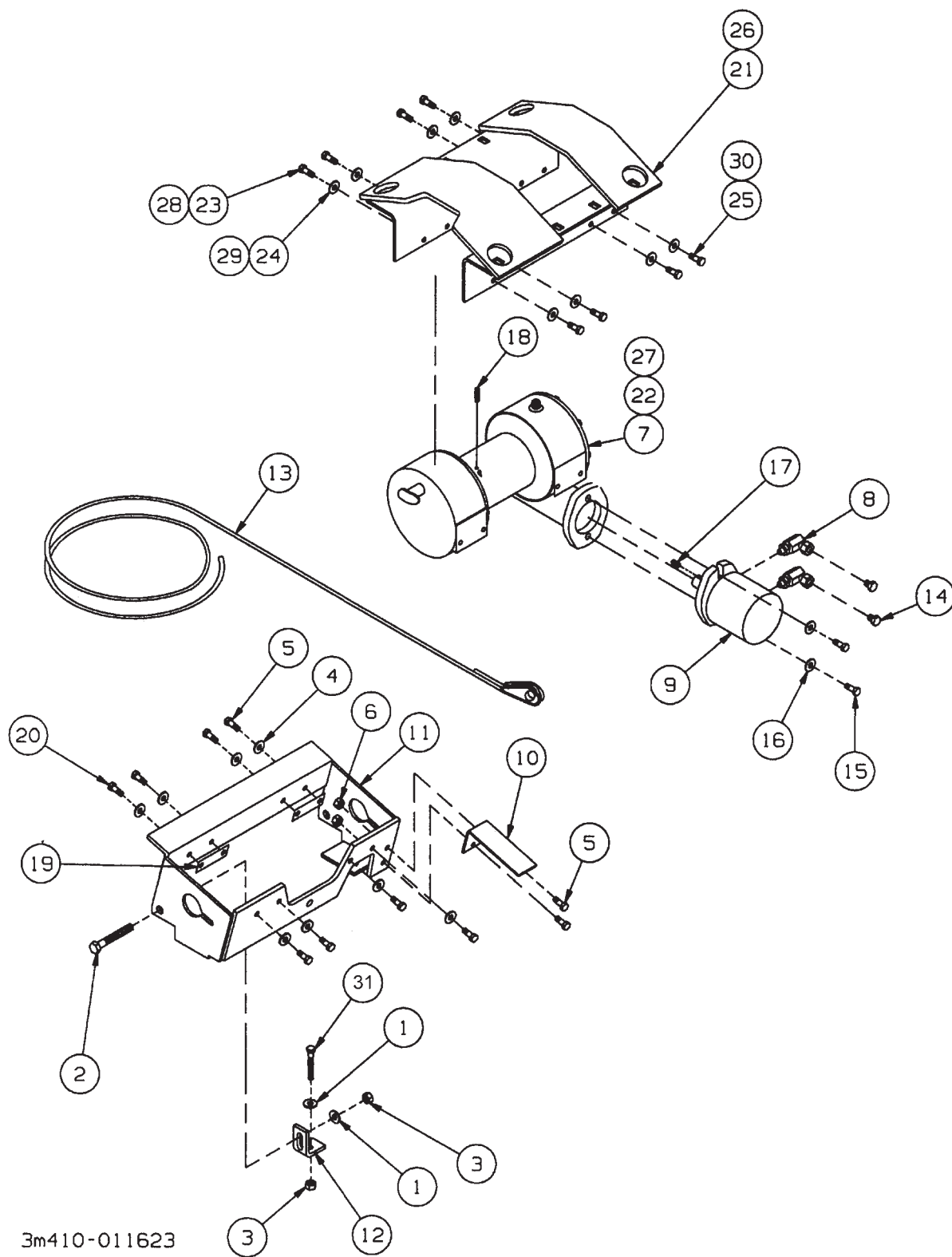
Figure 1-39 Winch Assembly
