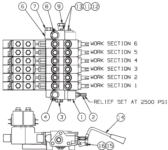
Figure 1-20 Six Spool Valve
