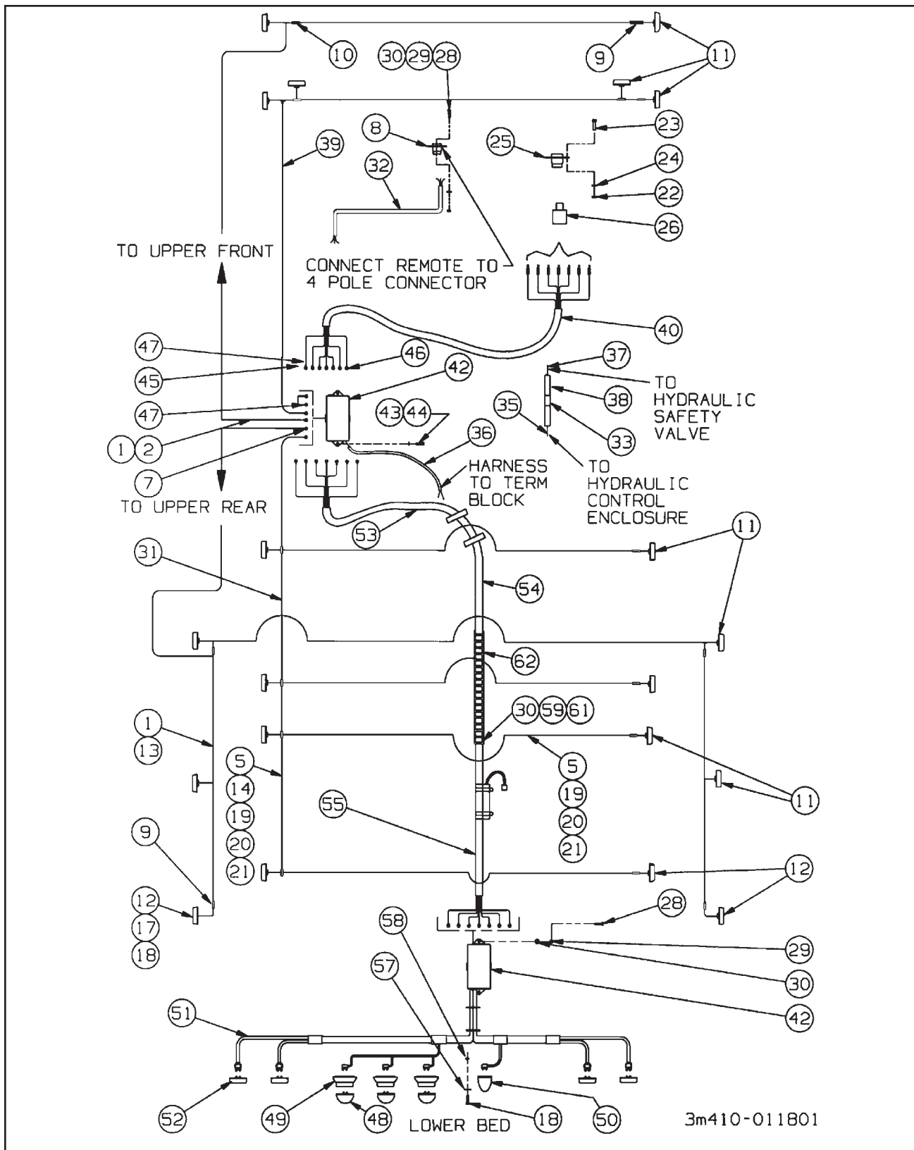
Figure 1-25 Electrical System
