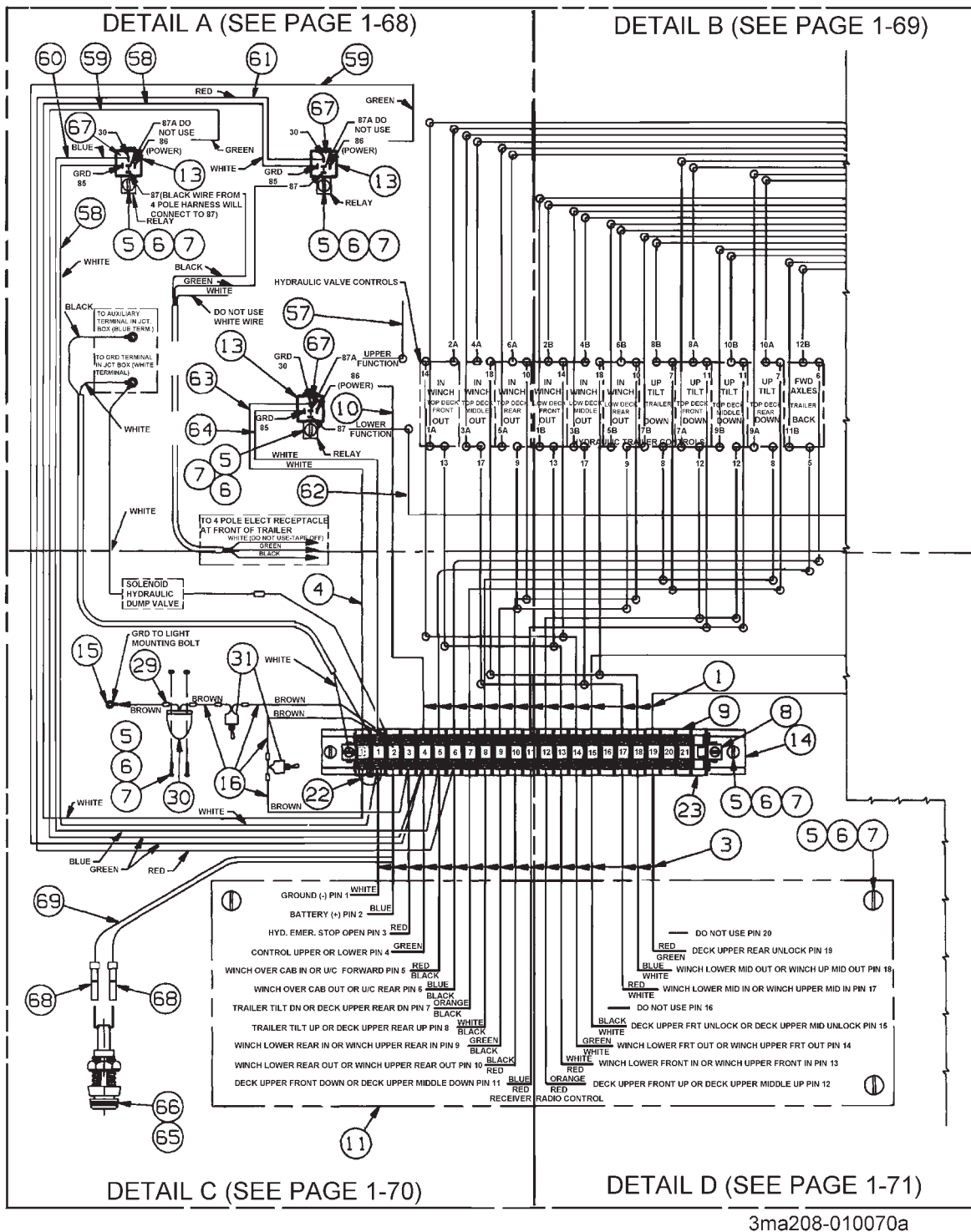
Figure 1-42 Electrical System, Remote Control
